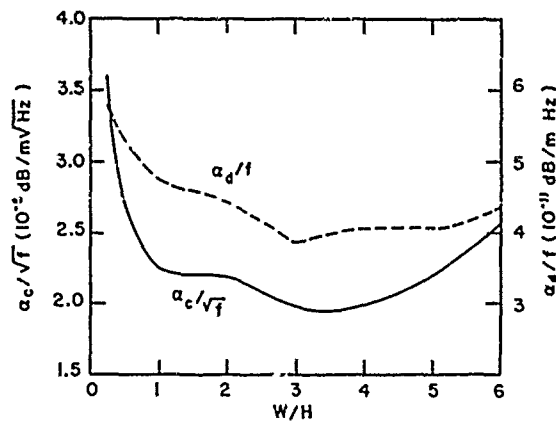
Fig. 13 — Loss constants vs aspect ratio for trapped inverted microstrip (Fig. 12)
