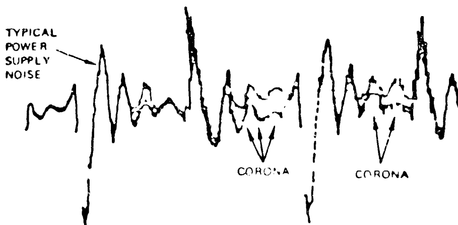
CORONA DETECTED BY REF COIL DISPLAY ON FIBER OPTICS RECORDER
