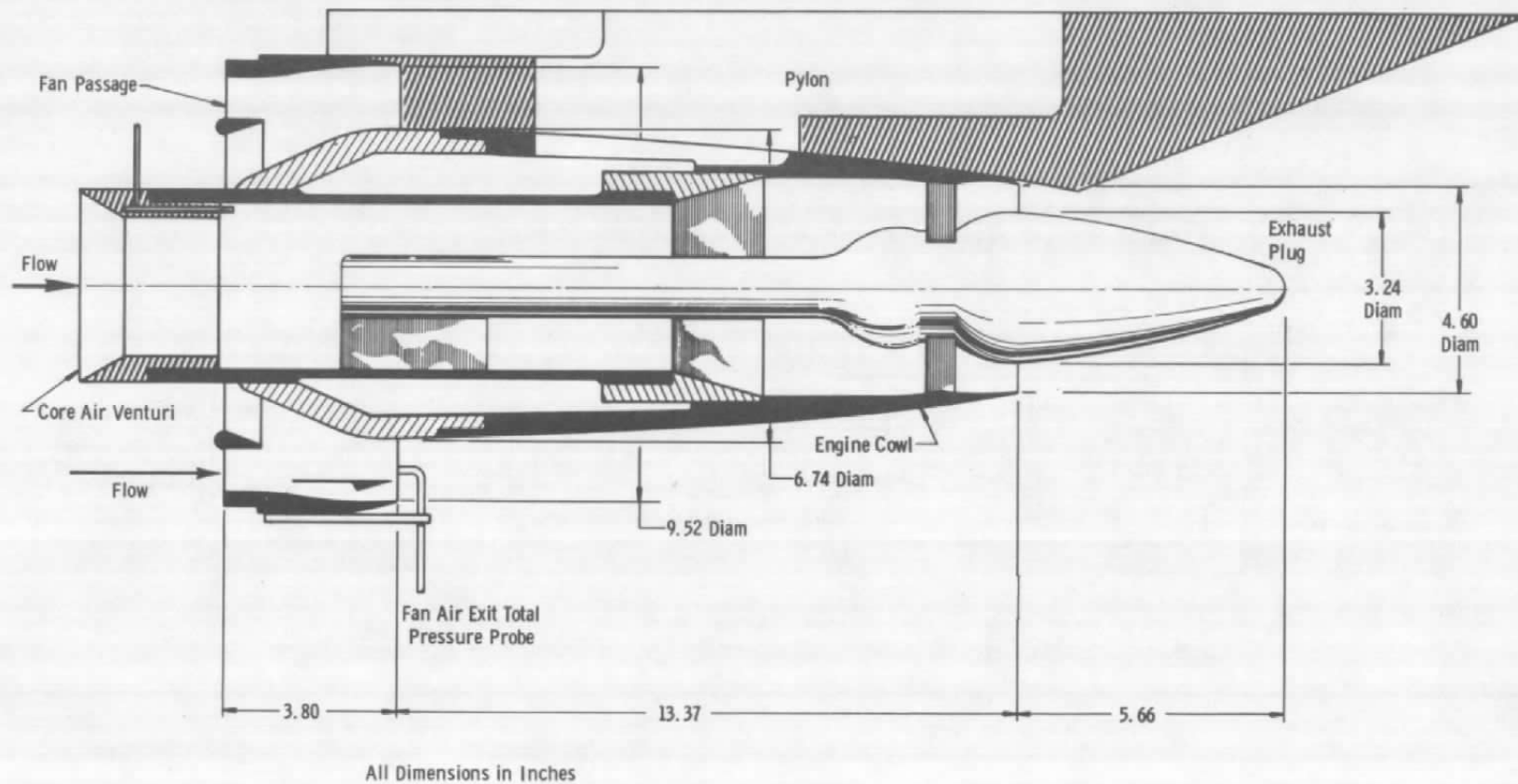
Figure 2. TF-39 model engine.
