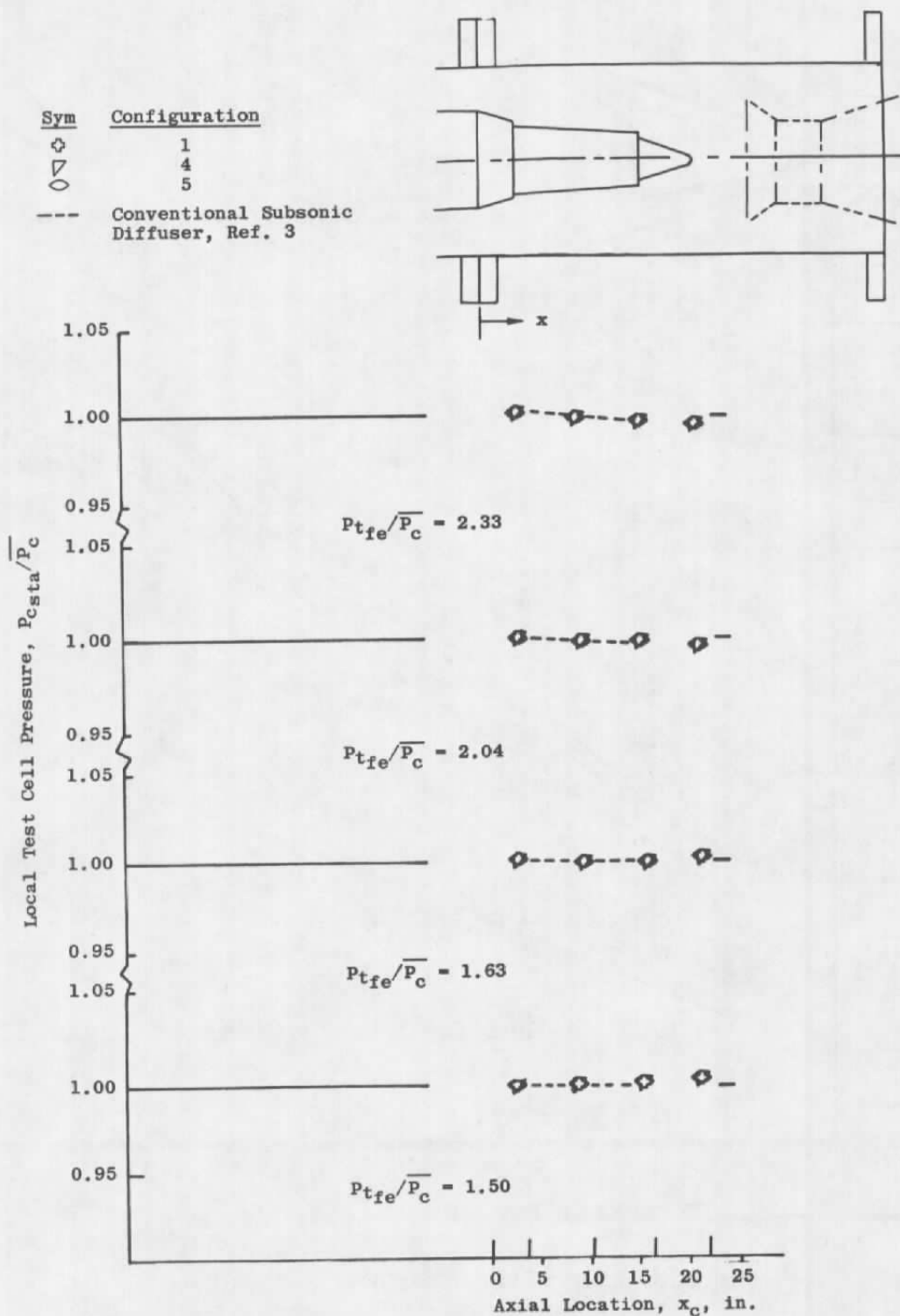
Figure 14. Axial variation of test cell pressure.
