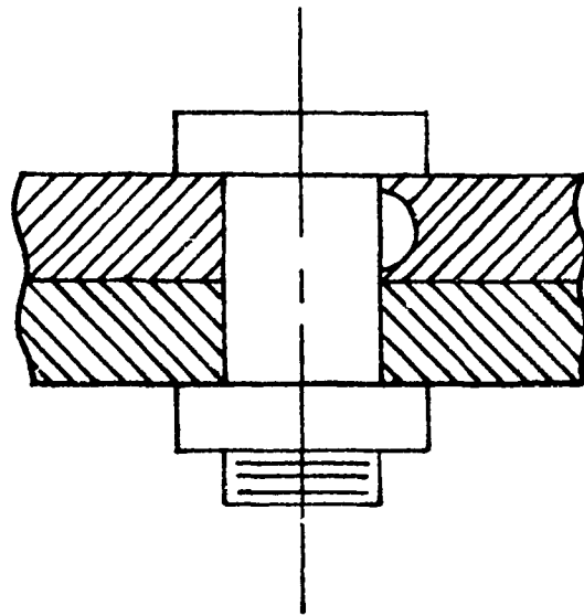
Internal Defect
