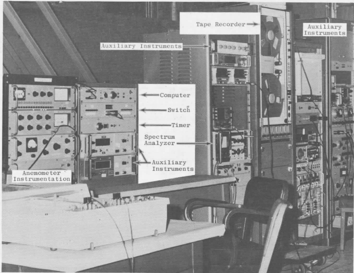
Figure 4. Assembled instrumentation.
