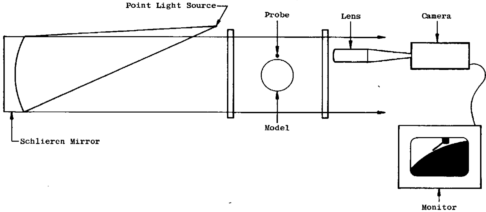
Figure 9. Video and light source system.
