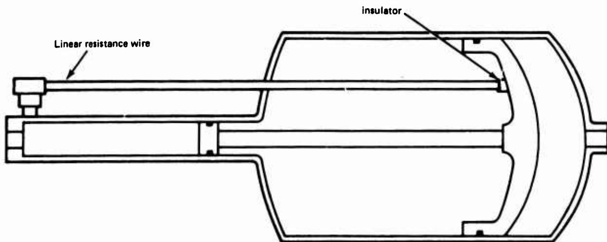
Figure 18. Linear potentiometer reservoir level sensor: method 2.
