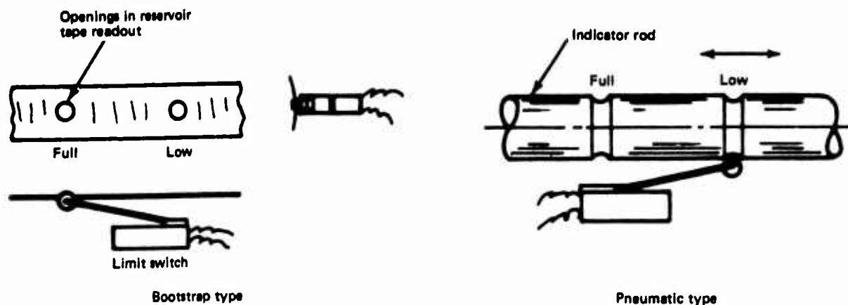
Figure 19. Limit switch type indicators; method 3.
