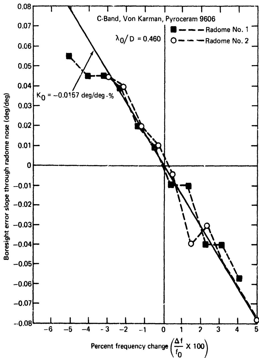
Fig. 4 C-Band Boresight Error Slope versus Percent Frequency Change
