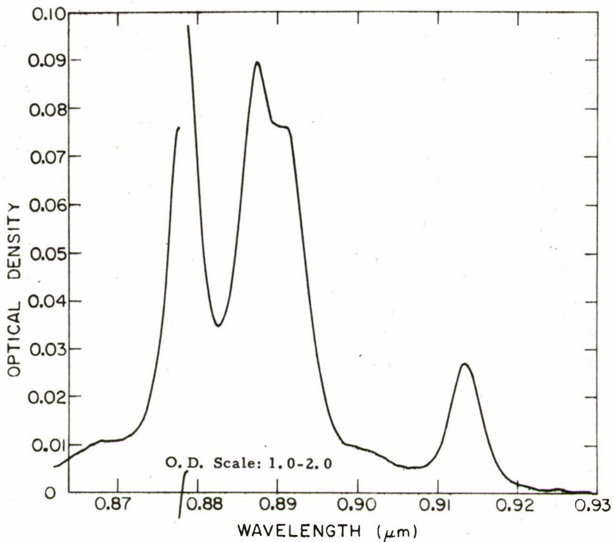
Figure 33. 0.89 μm Band of Nd:YVO 4 Absorption Spectra at Room Temperature. σ spectrum. 3% Nd. 8.5 mm thick.
