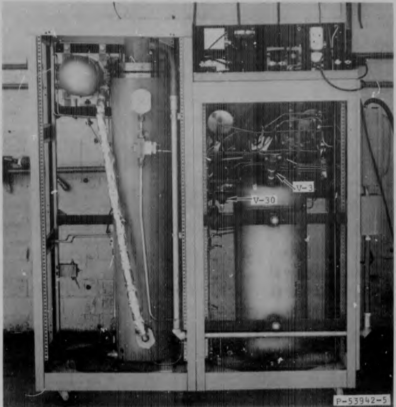
REAR VIEW OF COMPRESSOR BLEED AIR SIMULATOR
