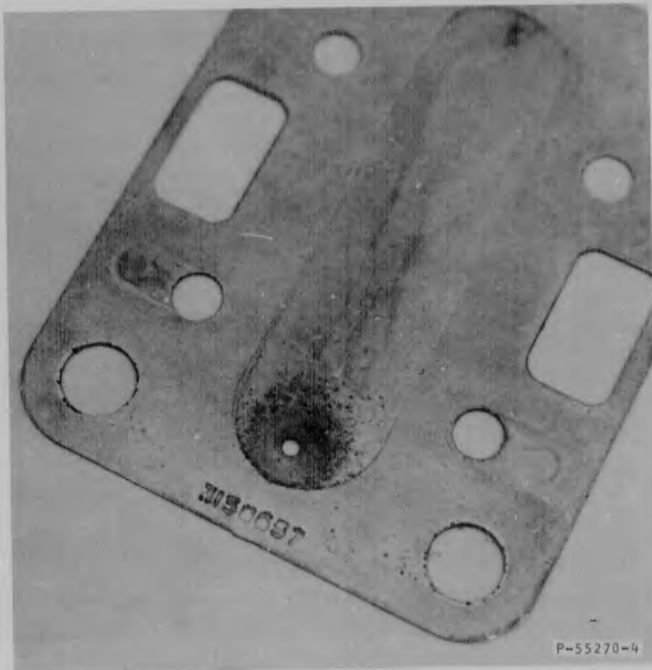
FIGURE 103 ORIFICE LAMINATION CIRCUIT 2, RUN 13
