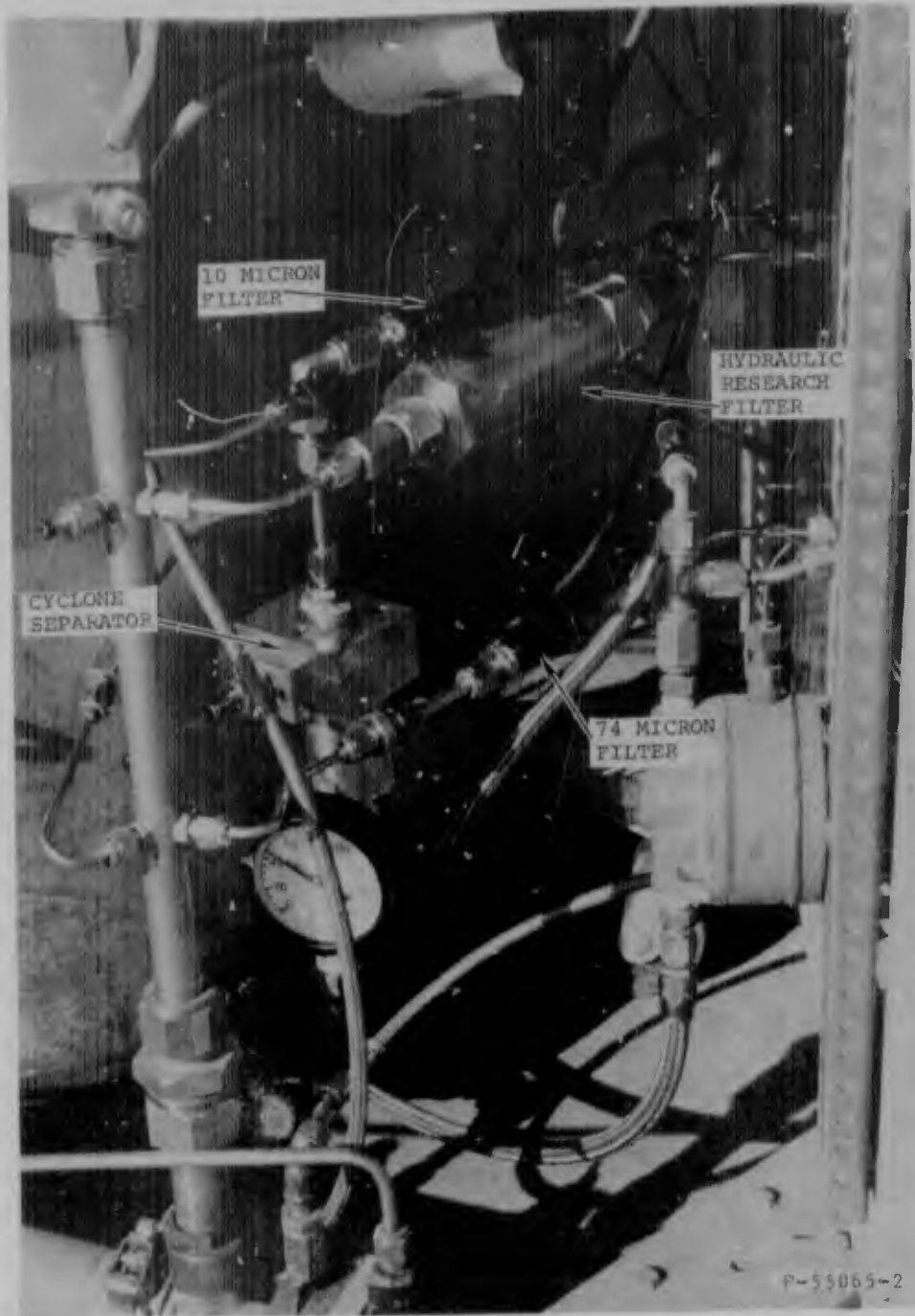
FIGURE 60 SERVICE LIFE TESTS TEST FILTER CONFIGURATIONS RUN 12
