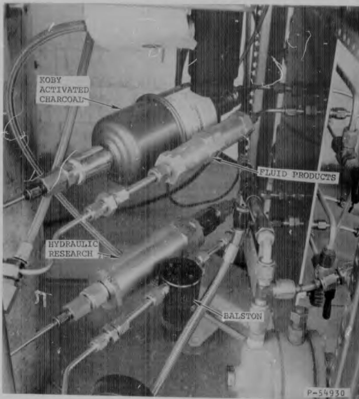
FIGURE 53 VIEW OF FOUR TEST FILTERS INSTALLED IN TEST SETUP
