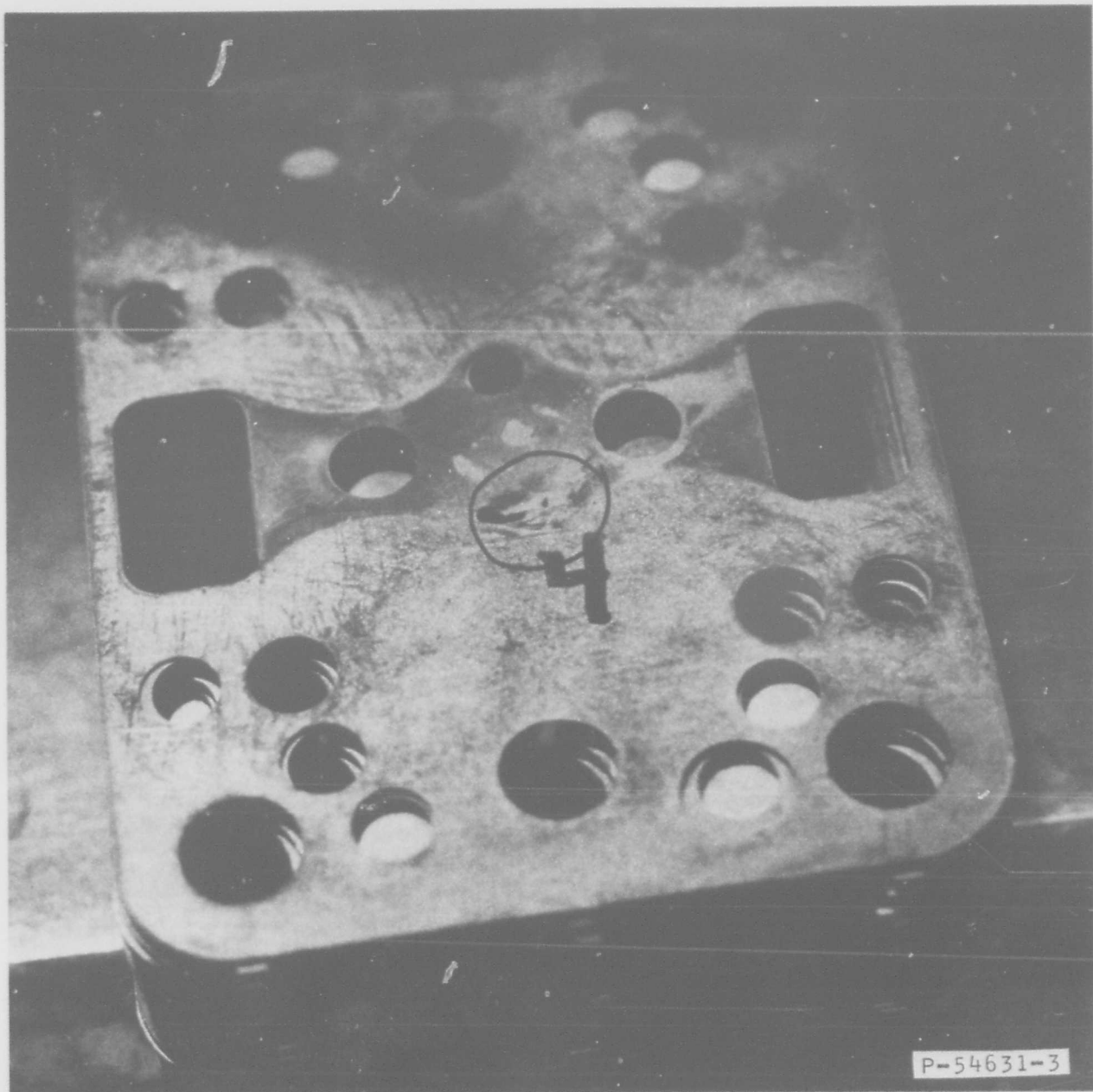
FIGURE 35 UNFILTERED BLEED AIR PARTIALLY BLOCKED VENT VIEWED FROM EXHAUST SIDE RUN 2, STATION 4, LAMINATION 26
