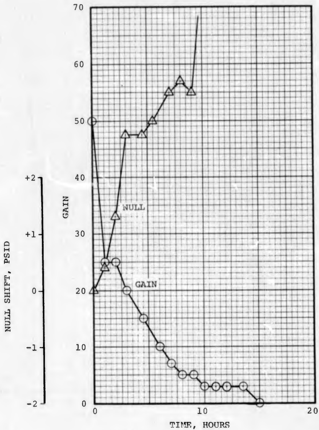
FIGURE 38 RUN THREE SUMMARY CIRCUIT STATION 3
