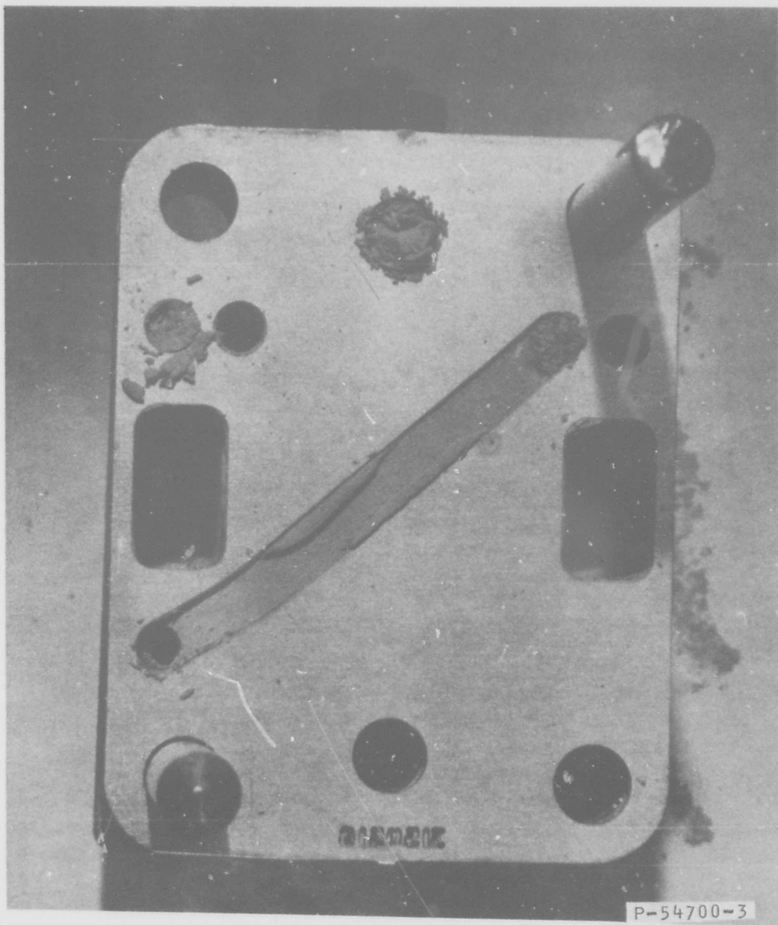
FIGURE 43 UNFILTERED BLEED AIR TEST DIRT PATTERNS IN TRANSFER RUN 3, STATION 1, LAMINATION 15
