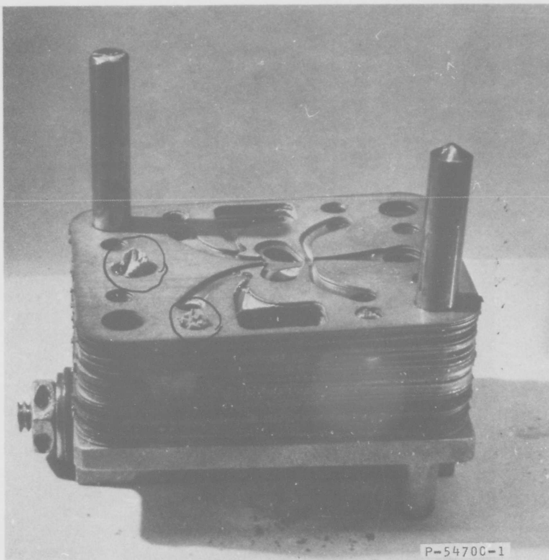
FIGURE 41 UNFILTERED BLEED AIR TEST BLOCKED SIGNAL PORTS RUN 3, STATION 1, LAMINATION 11
