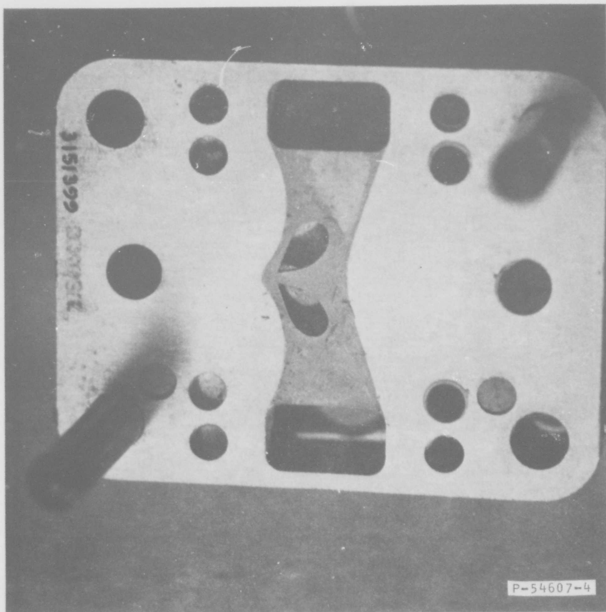
FIGURE 31 UNFILTERED BLEED AIR TEST DIRT BUILDUP IN FIRST STAGE EXHAUST REGION RUN 1, STATION 1, LAMINATION 12
