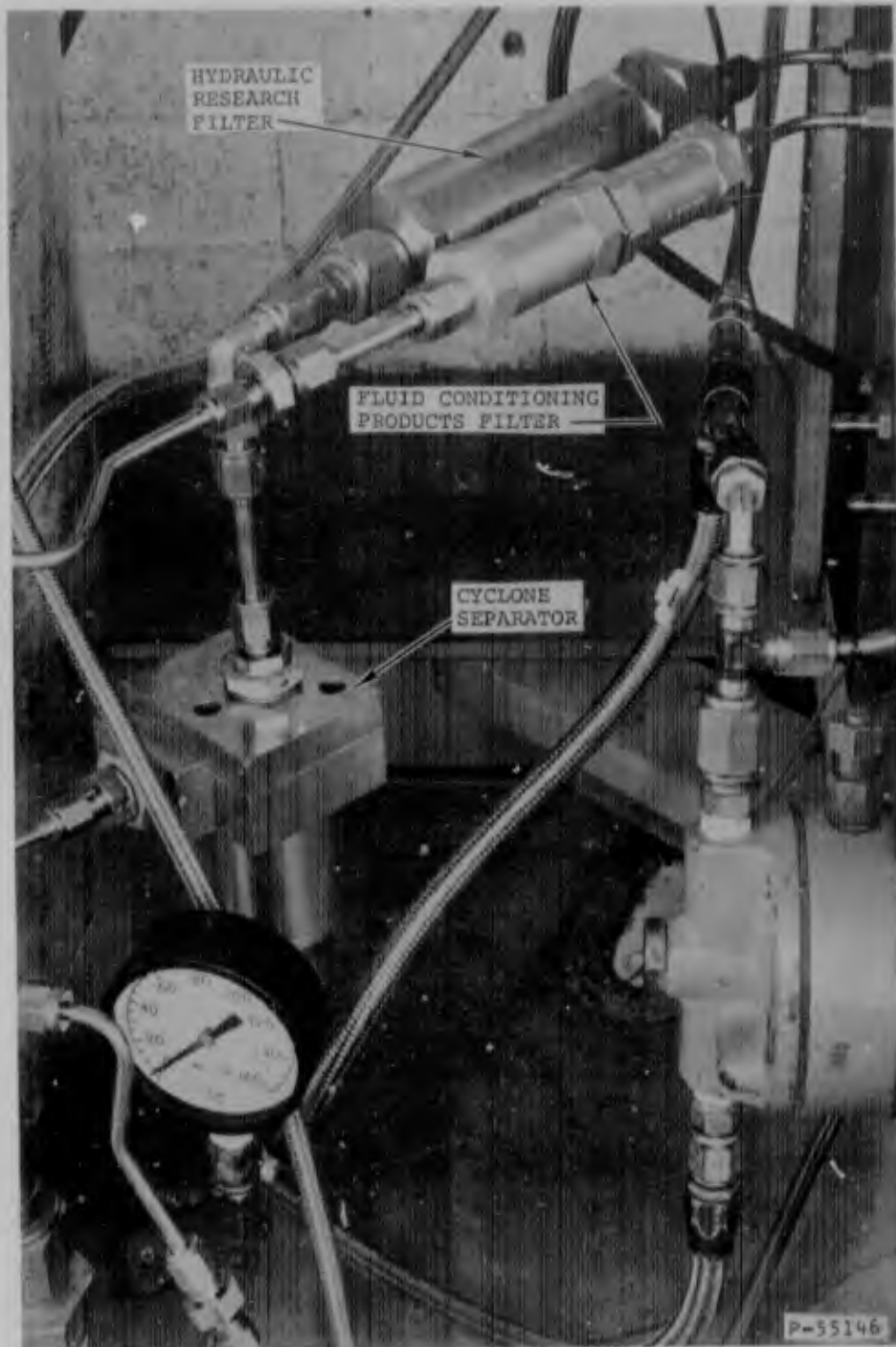
FIGURE 90 FILTER TEST SETUP RUN 13
