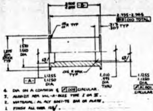
ITEM NO. 6. ROLLER, IDLER
