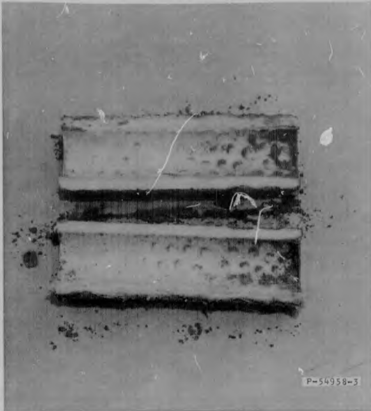
FIGURE 56 CUTAWAY VIEW OF BALSTON ELEMENT SHOWING DIRT MIGRATION THROUGH ELEMENT (NOTE SUPPORT TUBE PATTERN)
