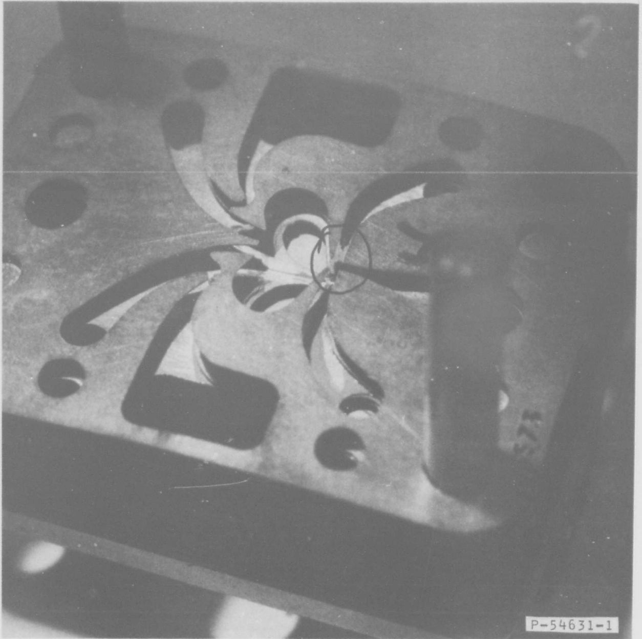
FIGURE 34 UNFILTERED BLEED AIR PLUGGED CONTROL PORT RUN 2, STATION 3, LAMINATION 11
