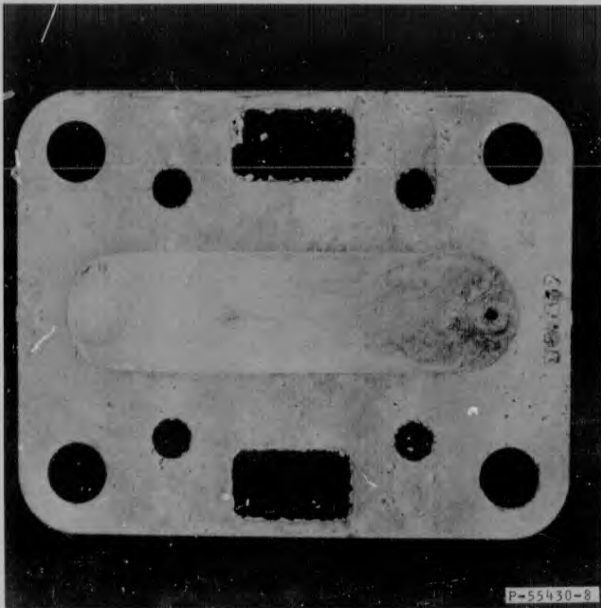
FIGURE 116 SUPPLY ORIFICE LAMINATION 4 CIRCUIT 1, RUN 14
