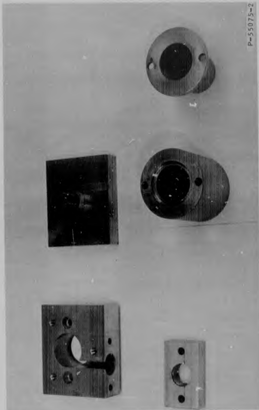
FIGURE 58 PHOTO OF CYCLONE SEPARATOR DISASSEMBLED
