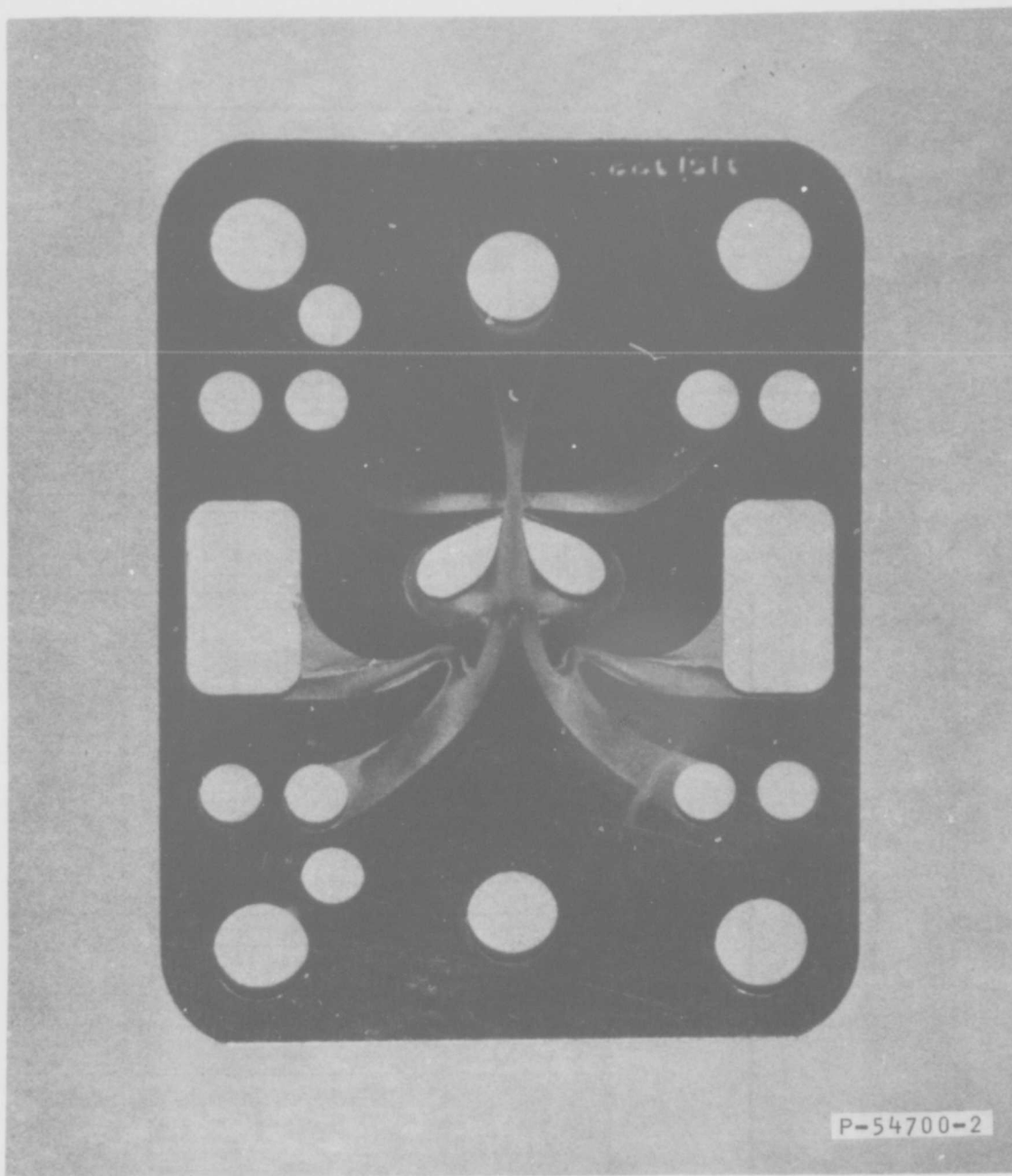
FIGURE 40 UNFILTERED BLEED AIR TEST DIRT PATTERNS ON VENT PLATE DEPICT FLOW PATTERNS THROUGH AMPLIFIER
