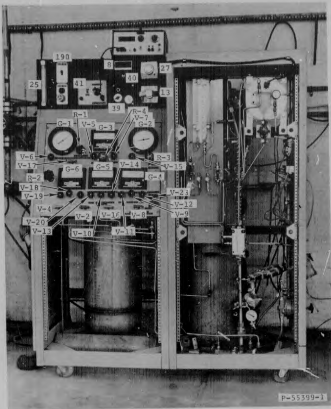
CONTROL PANEL COMPRESSOR BLEED AIR SIMULATOR
