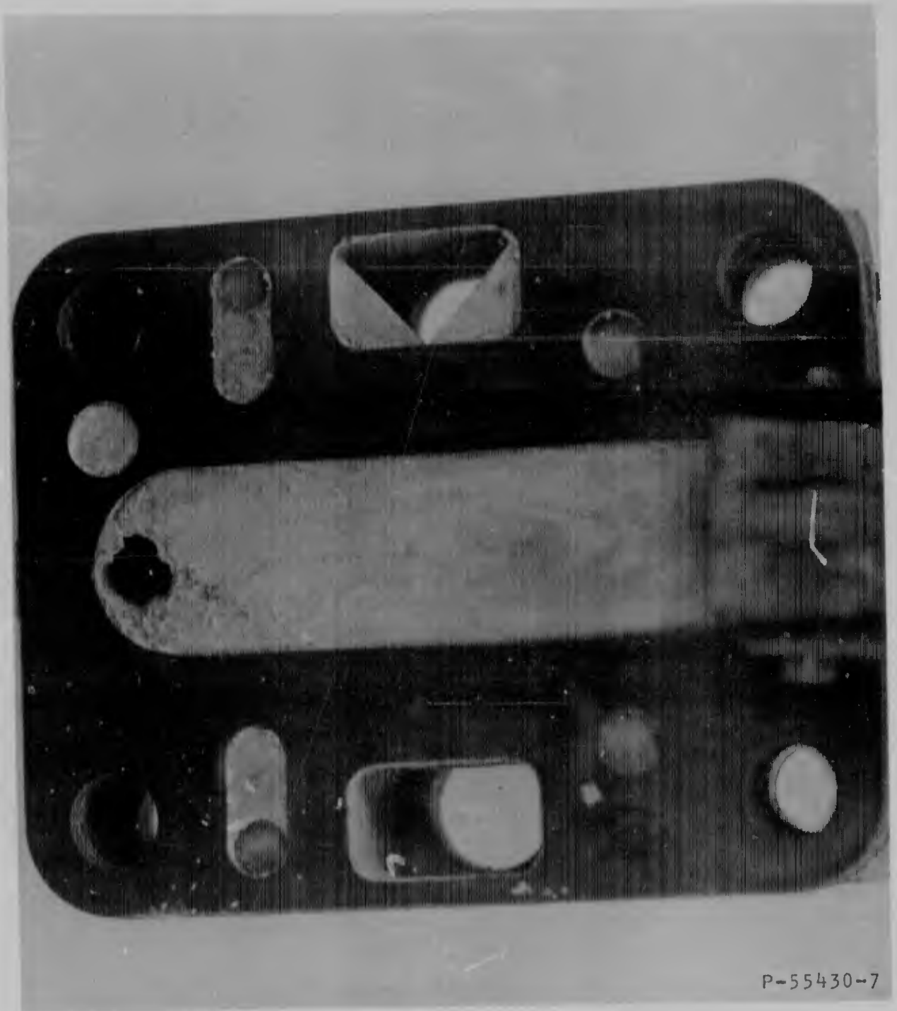
FIGURE 117 SUPPLY TRANSFER LAMINATION 5 CIRCUIT 1, RUN 14
