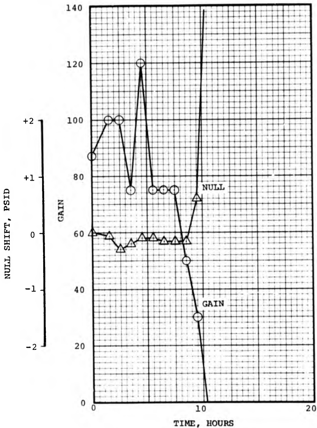
FIGURE 47 RUN FOUR SUMMARY CIRCUIT STATION 3
