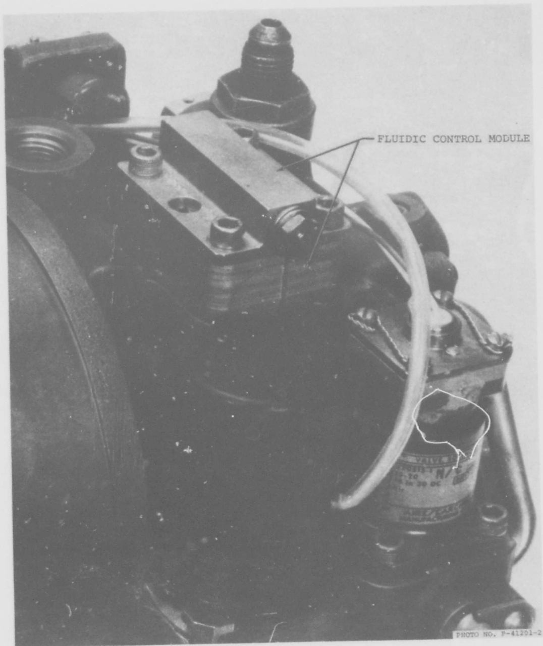
FIGURE 19 S-3A RAM AIR VENTILATION VALVE (AIRESEARCH PART 898524-1-1)
