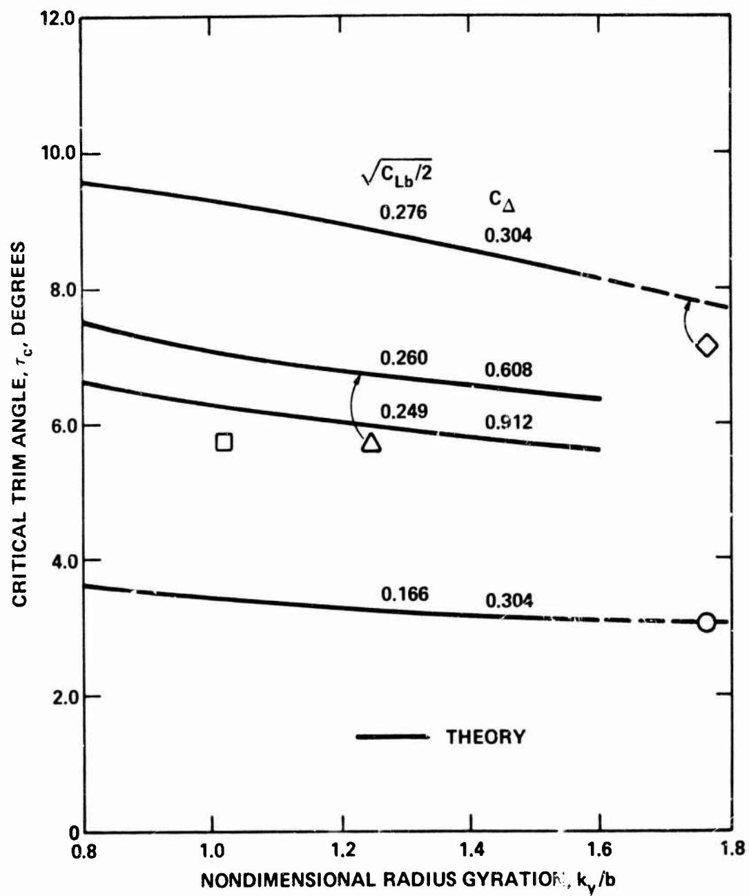
Figure 17a – Deadrise Angle \beta = 10^\circ
