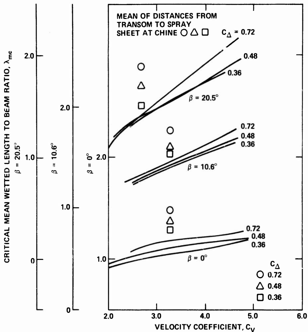
Figure 11 – Variation of Mean Wetted Length to Beam Ratio at Porpoising, with Speed, Deadrise Angle, and Loading
