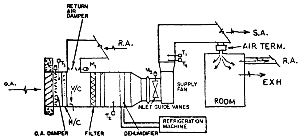
Figure 2. Variable Volume System Schematic Diagram
