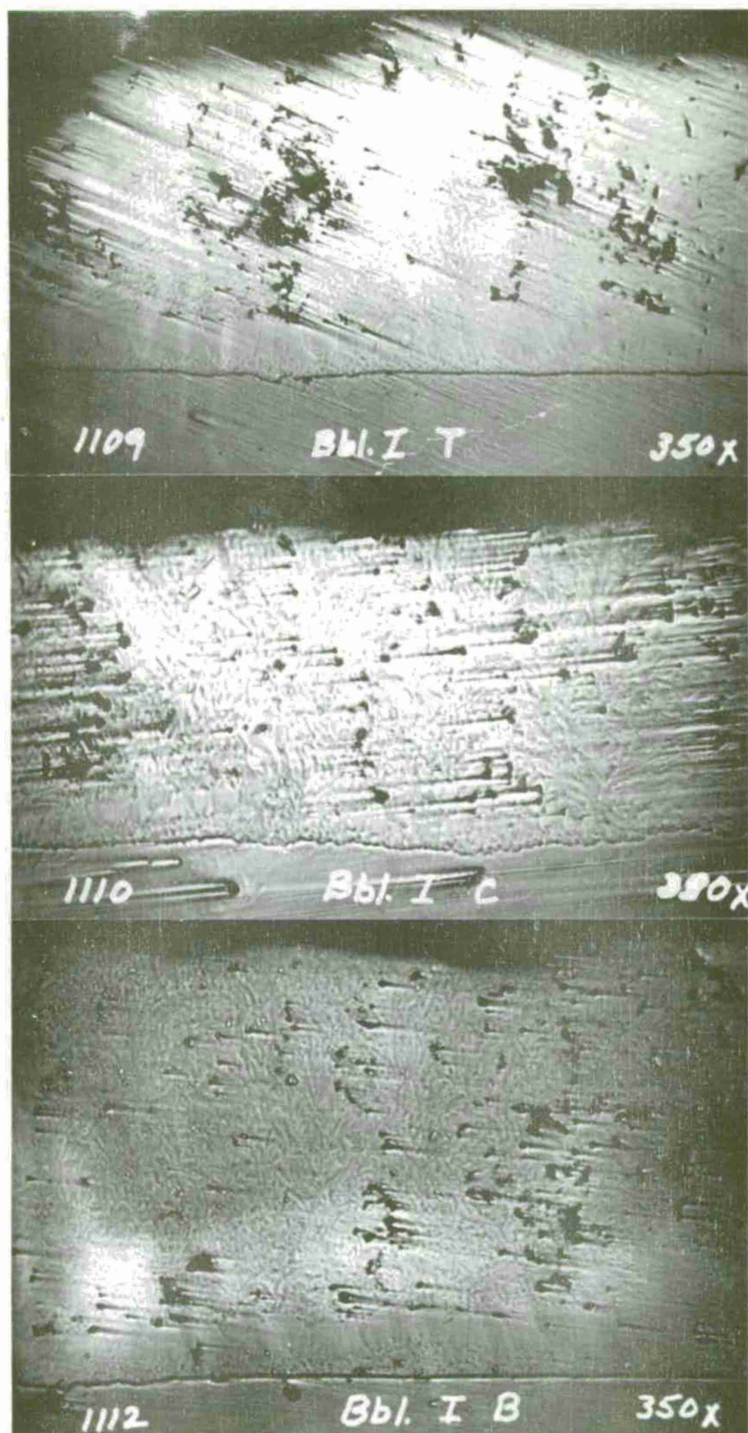
FIGURE 51 Chromium deposit on inside of stainless steel tube 3/8 inch ID x 20 inches long. Chromium deposited at 45°C/30 asd in tube in vertical position from bath containing 3 g/l \text{TiNO}_3 and 30 g/l \text{B}_4\text{C} . Cross-sections taken from top, center, and bottom of tube. Hard particles resist polishing and leave "tails" of raised Cr. No etch.
