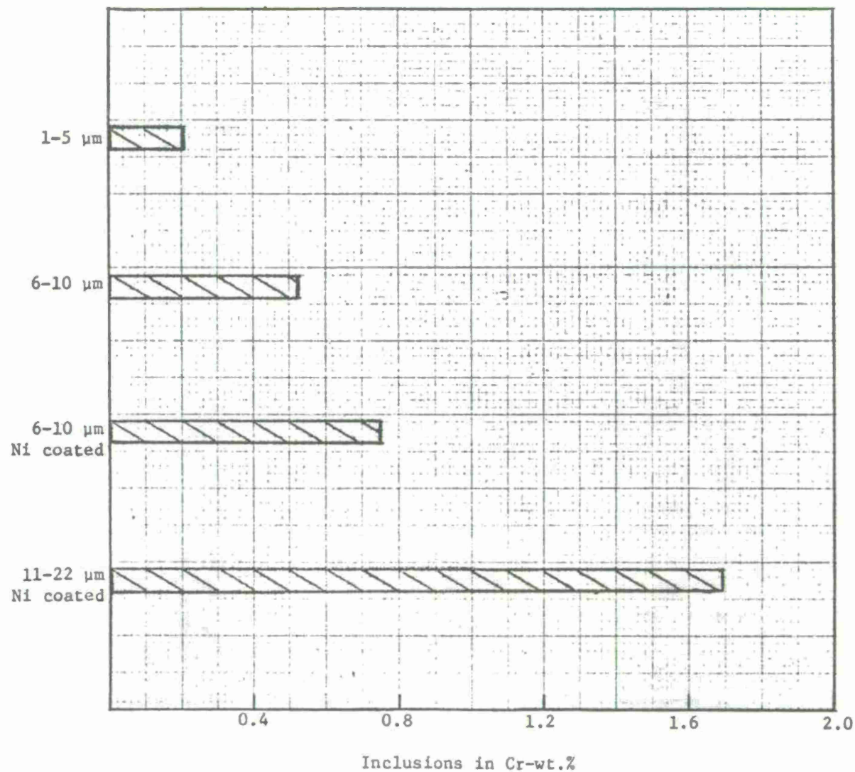
FIGURE 11 Type of diamond particles used with the average amount of each type included in a deposit on a horizontal cathode plated at 60°C and 40-60 asd in the standard 400 g/l \text{CrO}_3 bath plus 5 g/l \text{TiNO}_3 .
