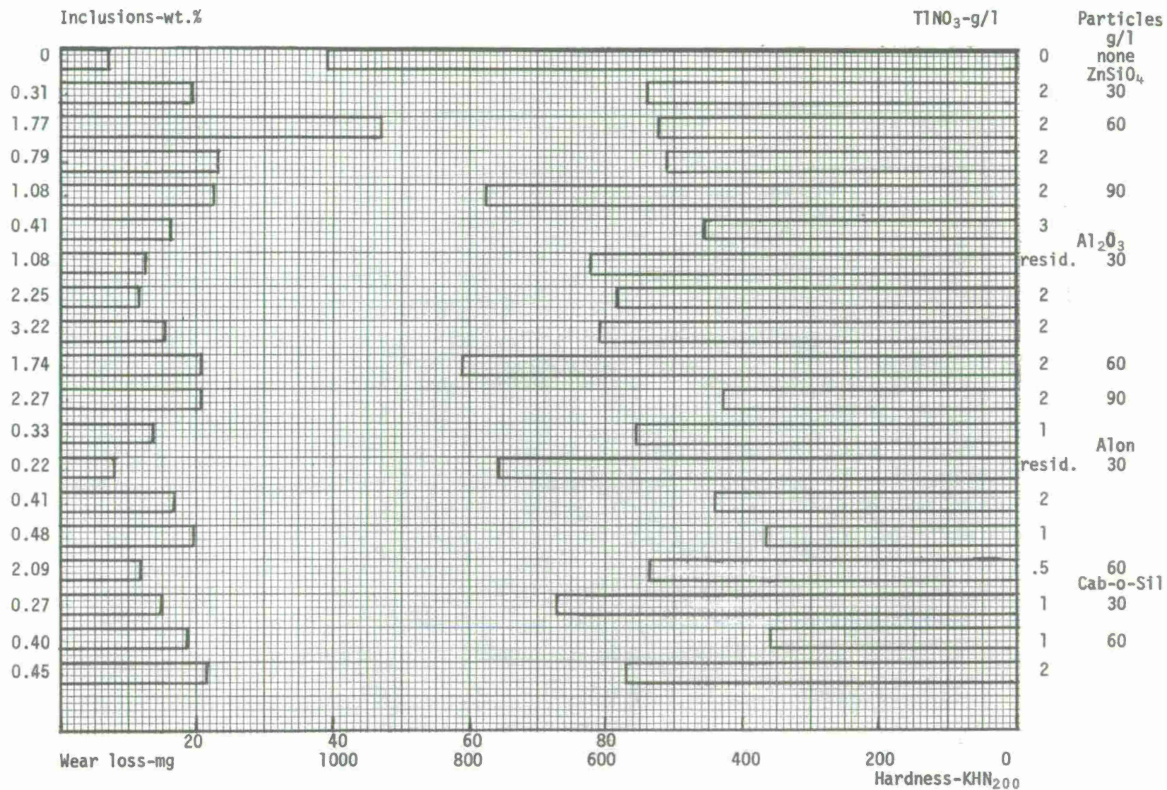
FIGURE 30 Summary of test deposits with new types of particles. Most runs at 45°/30 asd.
