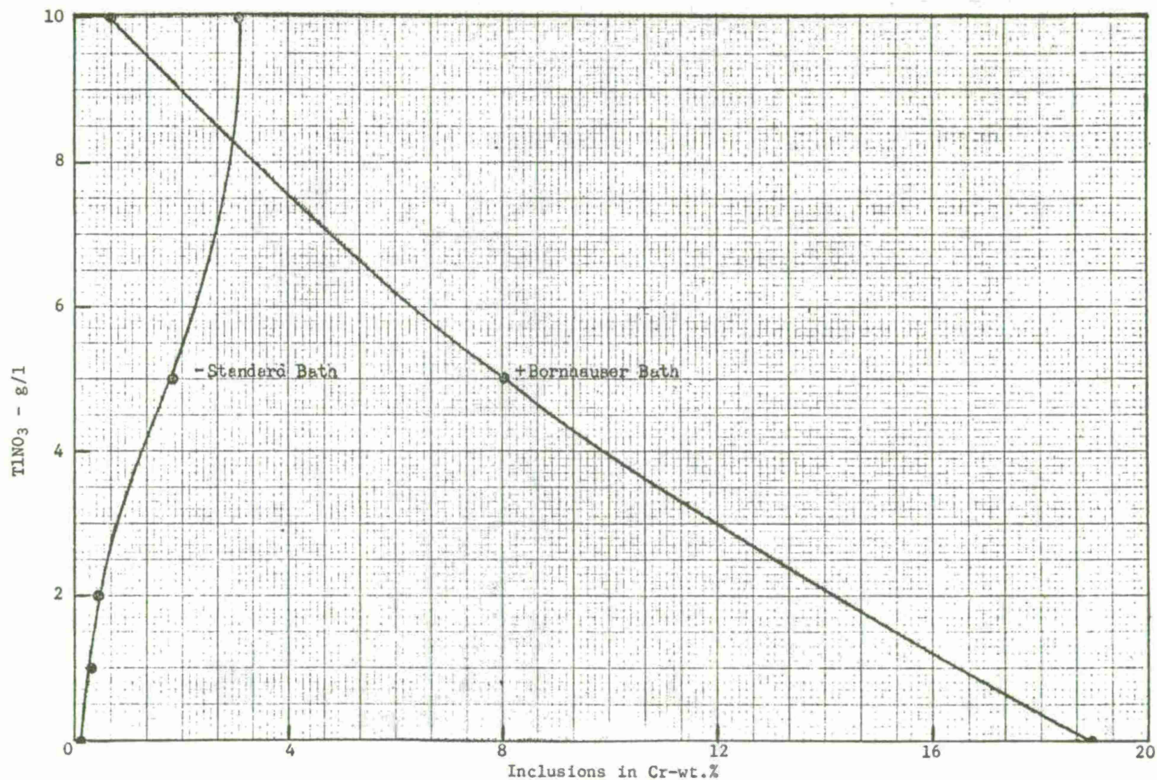
FIGURE 6 Thallium nitrate concentration versus amount of inclusions in the deposits from the standard 400 g/l CrO 3 and Bornhauser chromium baths. Plated at 60°C and 40 asd with 20 g/l SiC.
