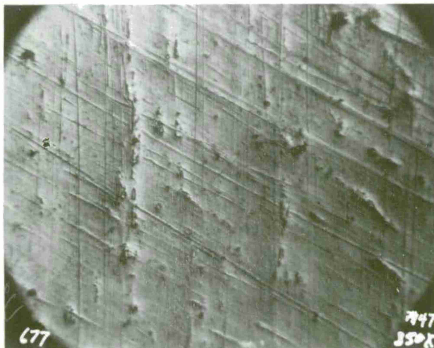
FIGURE 3 Off-center Abraser wheels mark specimen surface at nearly right angles. Deposit contains 0.43 wt.% of codeposited nickel coated diamond particles. Original 350X.
