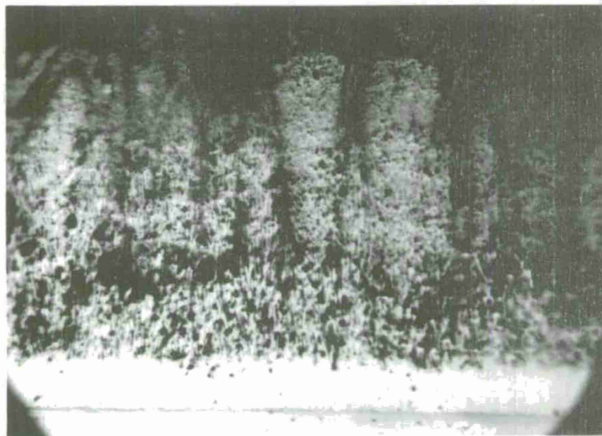
FIGURE 5 Cross-section of deposit plated at 60^\circ/40 asd from the Bornhauser bath plus 20 g/l SiC. Deposit contained 10 wt.% SiC but hardness was only 243 KHN 200 and wear loss an excessive 7+ grams. Original 350X.
