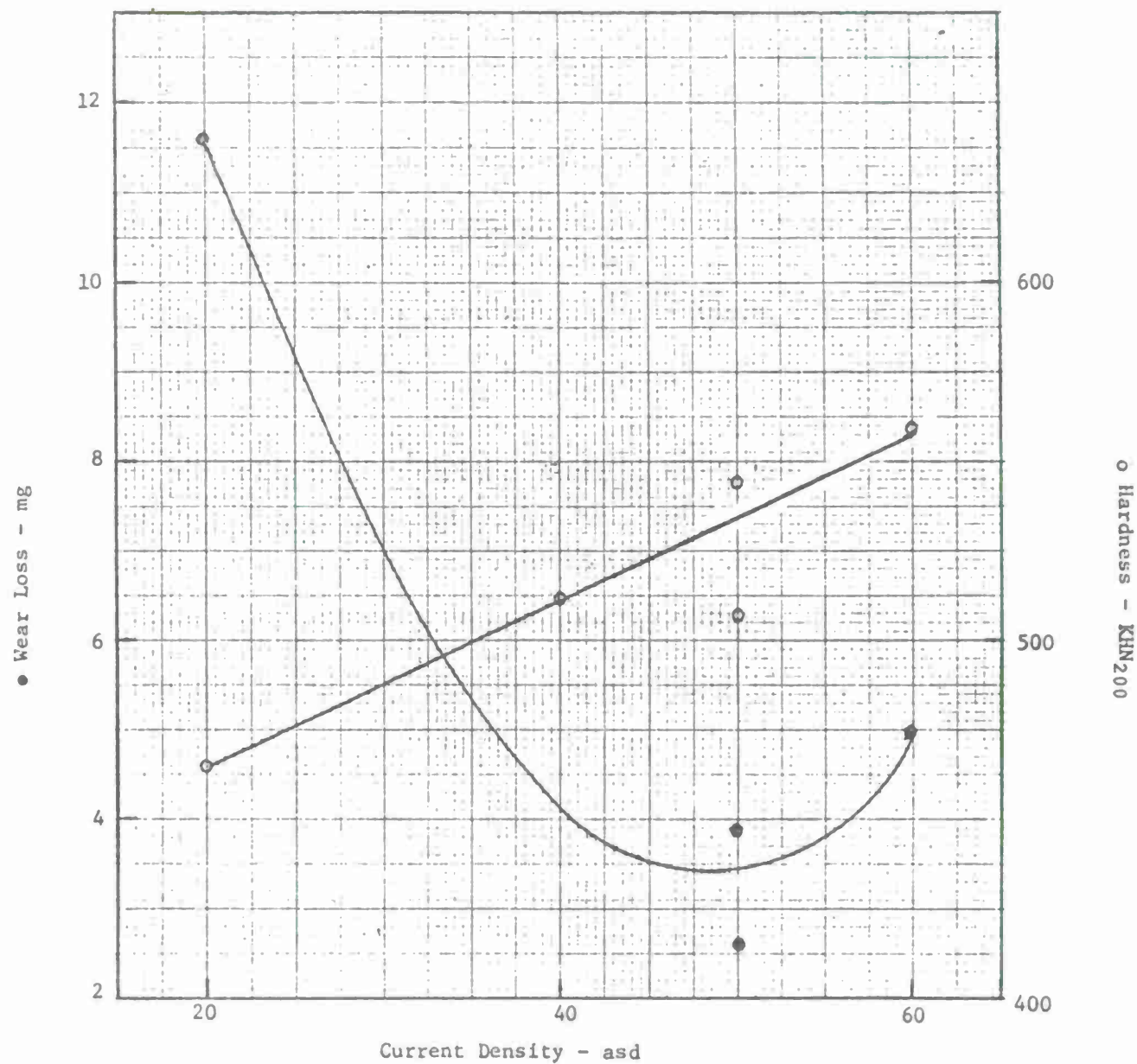
FIGURE 13 Effect of current density on hardness and wear. Deposits made in standard 200 g/l \text{CrO}_3 bath plus 1 g/l \text{TiNO}_3 and 18 g/l 15 \mu\text{m} nickel coated diamond powder at 55°C.
