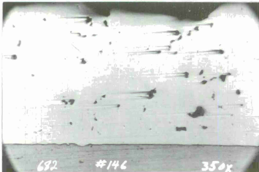
FIGURE 20 Cross-section of deposit made with 1 g/l \text{TiNO}_3 added in increments, one-half first then two additions of one-fourth at equal time intervals. Deposit made in 200 g/l \text{CrO}_3 bath plus 18 g/l of 15 \mu\text{m} nickel coated diamond powder at 55°/50 asd and contained 0.18 wt.% diamond. Original 350X.
