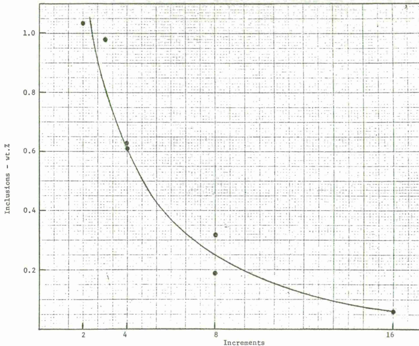
FIGURE 21 Weight percent of included SiC particles versus number of equal and equally spaced incremental additions of \text{TiNO}_3 for a sum total concentration of 1 g/l.
