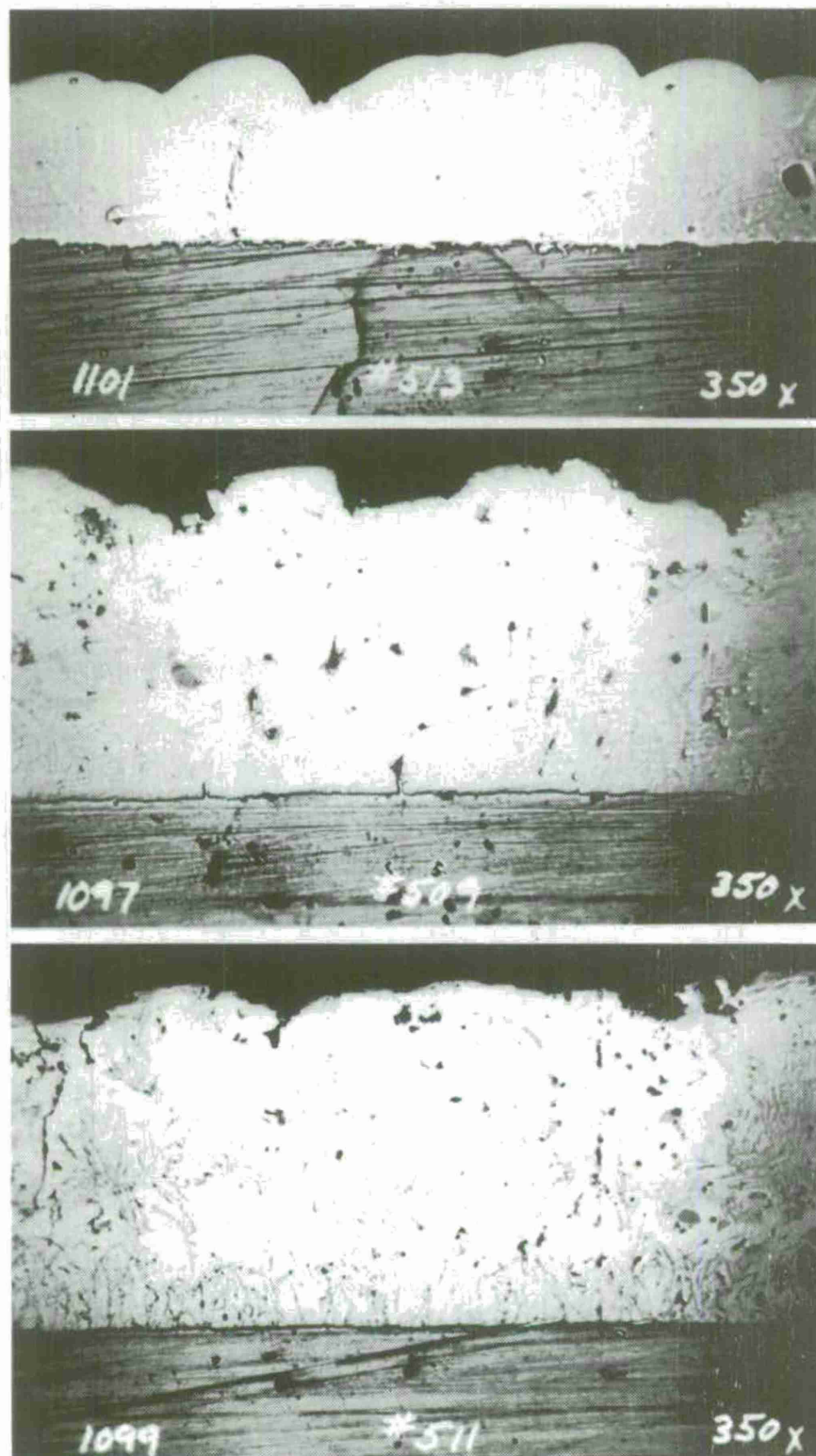
FIGURE 52 Heat-treated series. Top 250°C for 2 hrs, center 400°C for 1 hr, bottom 600°C for 1 hr. Chromium deposited on copper from bath containing 3 g/l \text{TiNO}_3 . No etch.
