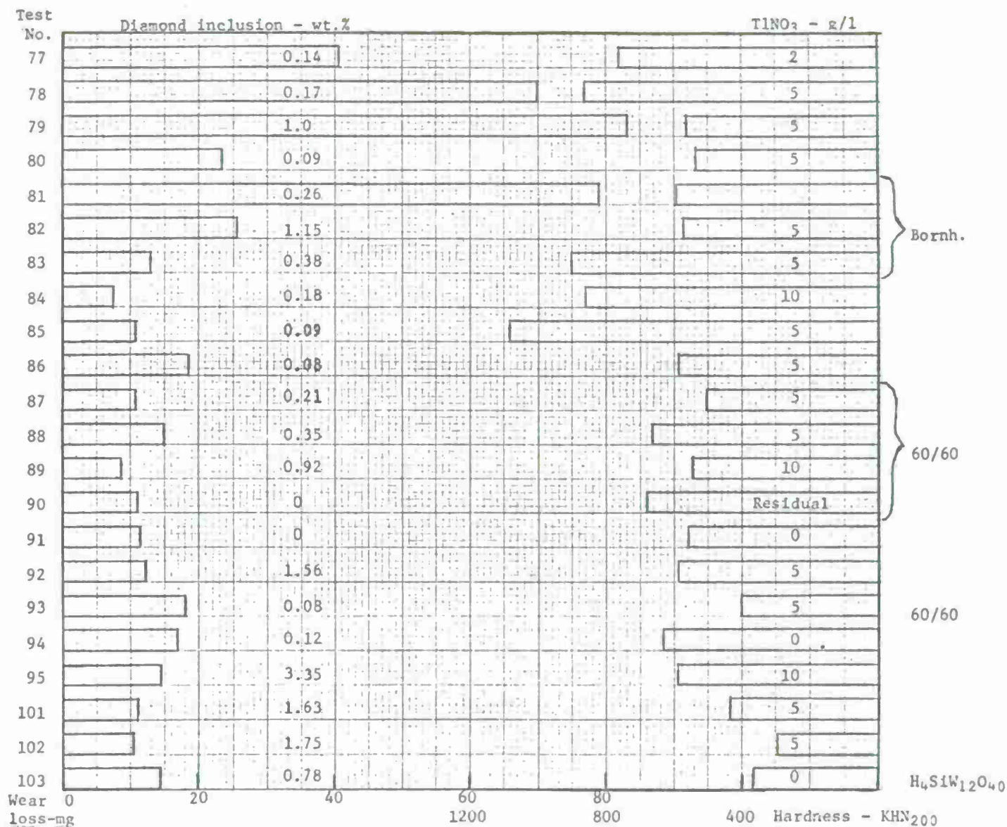
FIGURE 22 Effect of inclusions on wear loss and hardness of chromium deposits plated from standard 400 g/l CrO 3 bath plus TiNO 3 at 60°/40 asd, except as indicated. Distance between ends of bars for a given test roughly indicates effectiveness of inclusions in deposit, the greater the separation between the bar ends the larger the beneficial effect.
