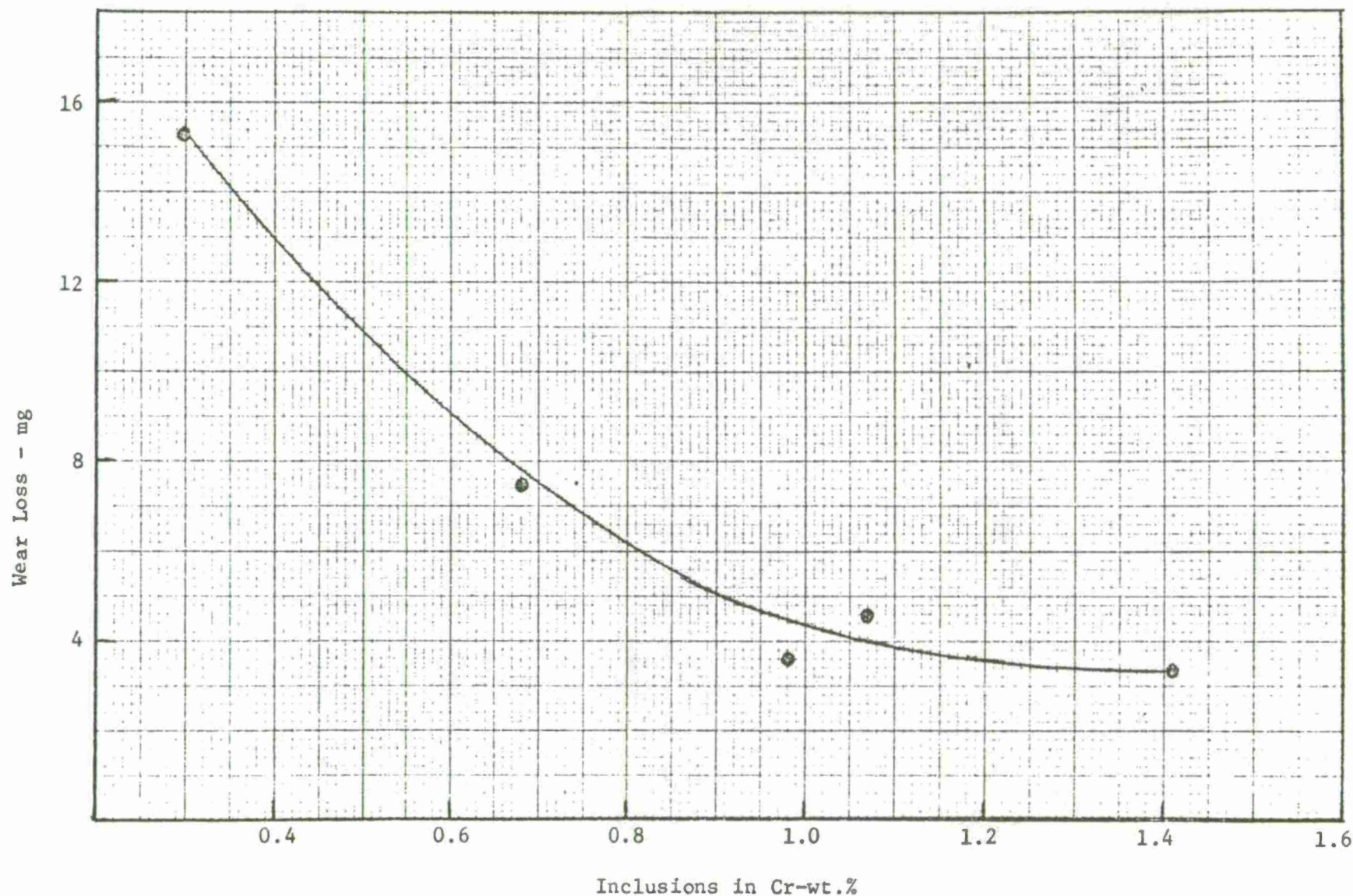
FIGURE 18 Amount of SiC in deposits versus wear loss of deposits plated at 55°C and 50 asd in the standard 200 g/l chromium bath plus 1 g/l \text{TiNO}_3 and SiC particles.
