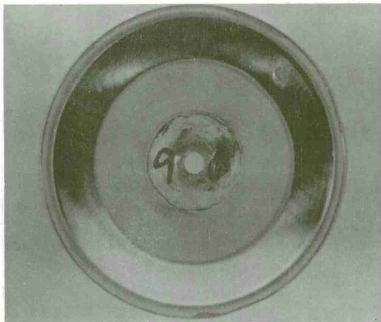
FIGURE 2 Experimental chromium deposit 5 mils thick on 3-3/4 inch horizontal copper cathode disc showing wear track of Tabor Abraser wheels. Center area not plated. Wear resistance of deposit determined by weight loss.
