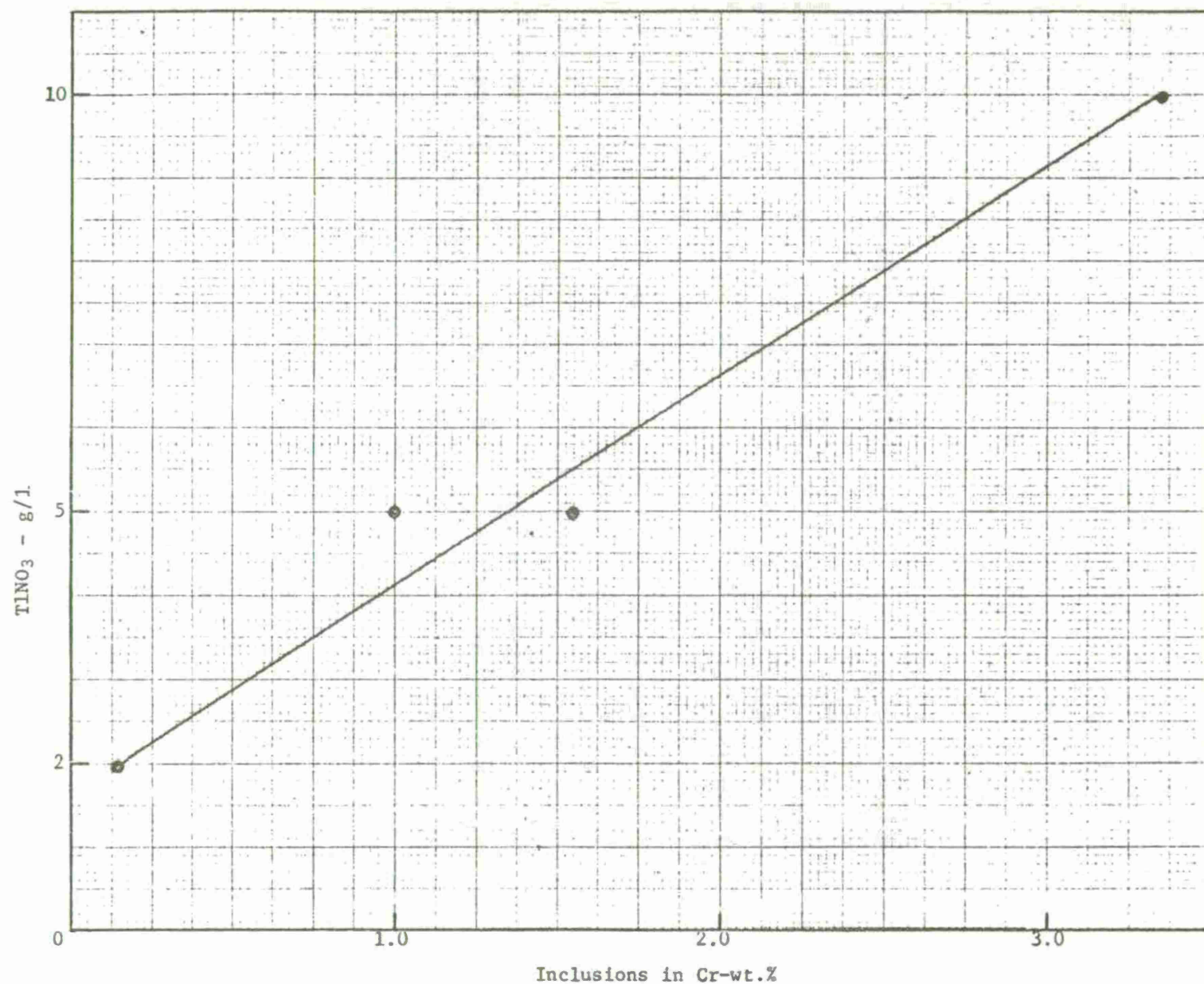
FIGURE 8 Thallium nitrate concentration versus amount of 6-10 \mu m diamond particles included in the deposits from the standard, 400 g/l CrO 3 chromium bath. Plated at 60°C and 40 asd.
