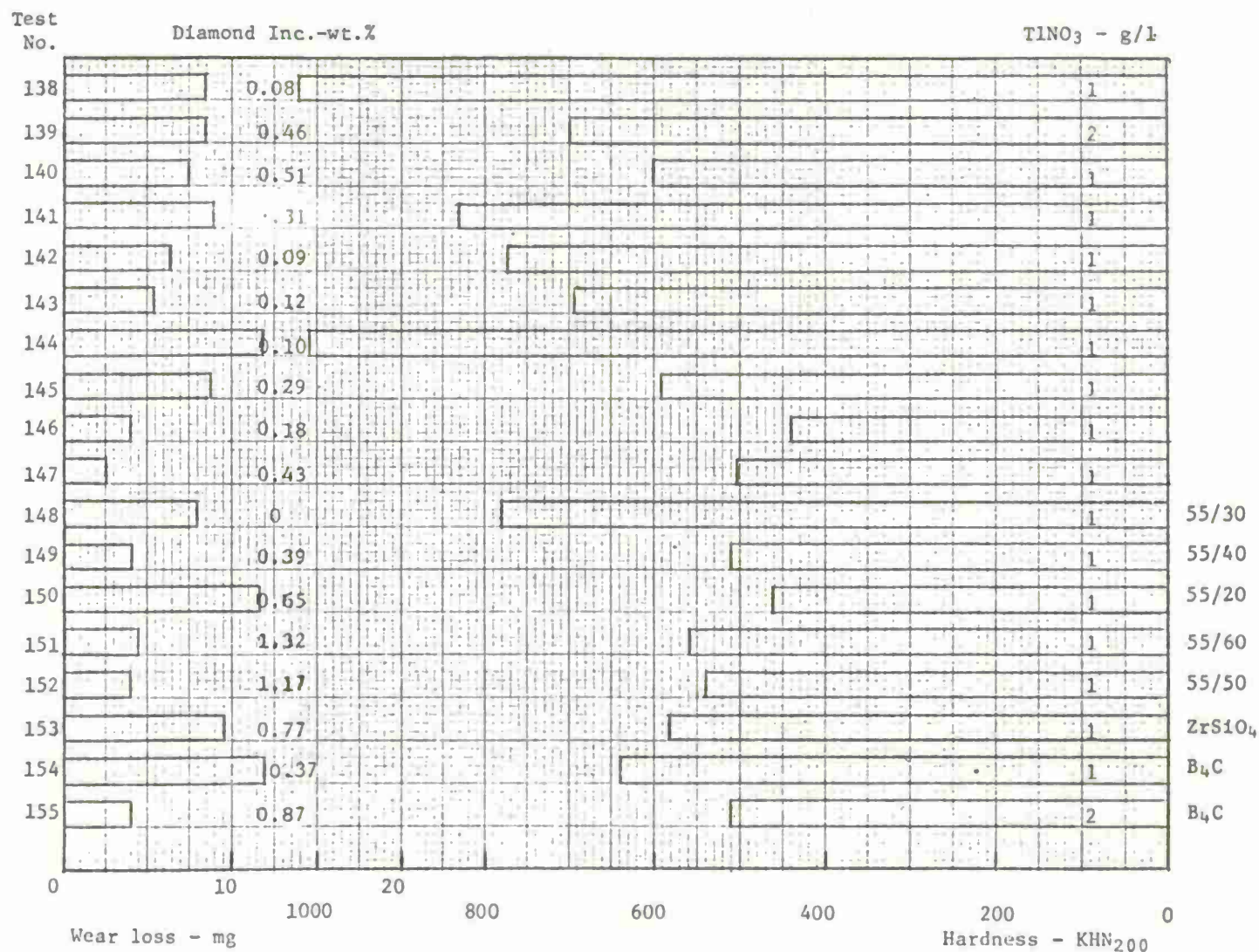
FIGURE 25 Wear loss in relation to hardness of deposits from standard 200 g/l \text{CrO}_3 bath plus \text{TiNO}_3 and diamond powder and at 55°/50 asd, except as otherwise indicated.
