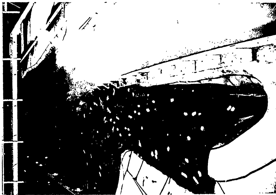
a. Discharge 50,000 cfs (chute), tailwater el 1021.1
