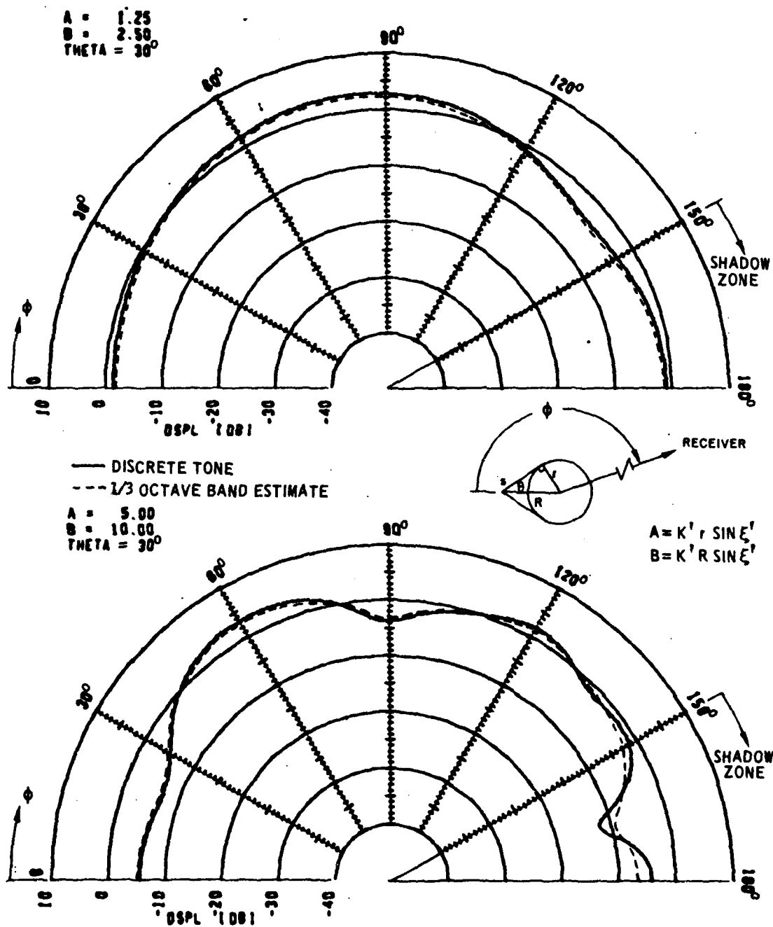
Figure D-4.—Noise Diffraction About a Fuselage
