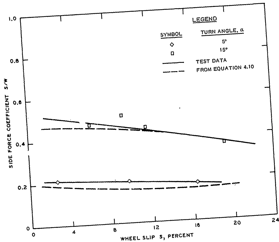
Figure 4.34. Influence of Turn Angle on Side Force Coefficient. Average Cone Penetration Resistance Gradient G = 3.2 , Tire Deflection \delta/h = 0.35 , Design Wheel Load W = 2,000 N. Desired Sand Mobility Number N_s = 13.2 .
