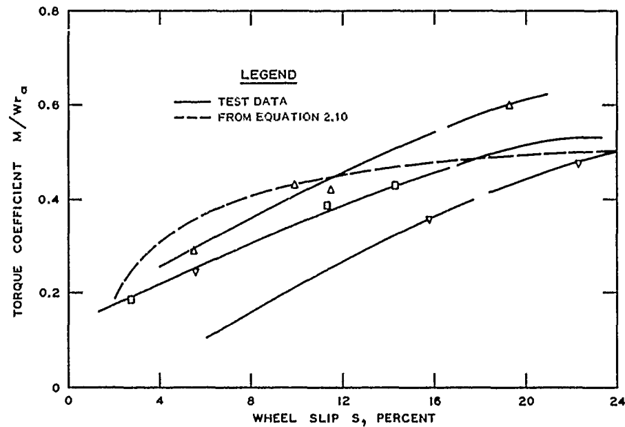
b. TORQUE COEFFICIENT
