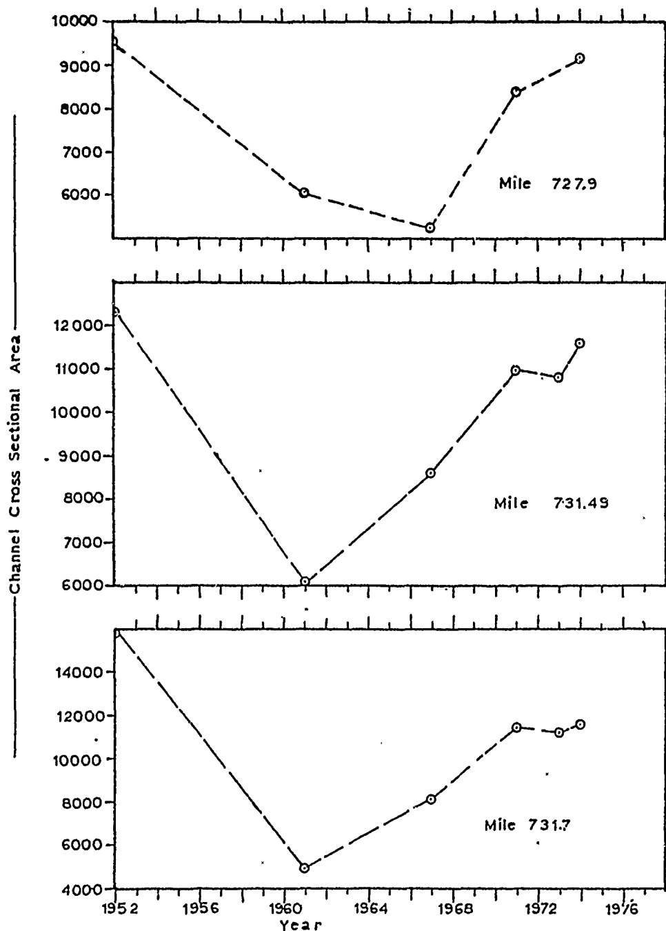
FIGURE 7. CHANNEL CROSS SECTIONAL AREA OF MISSOURI RIVER AT SIOUX CITY, IOWA
