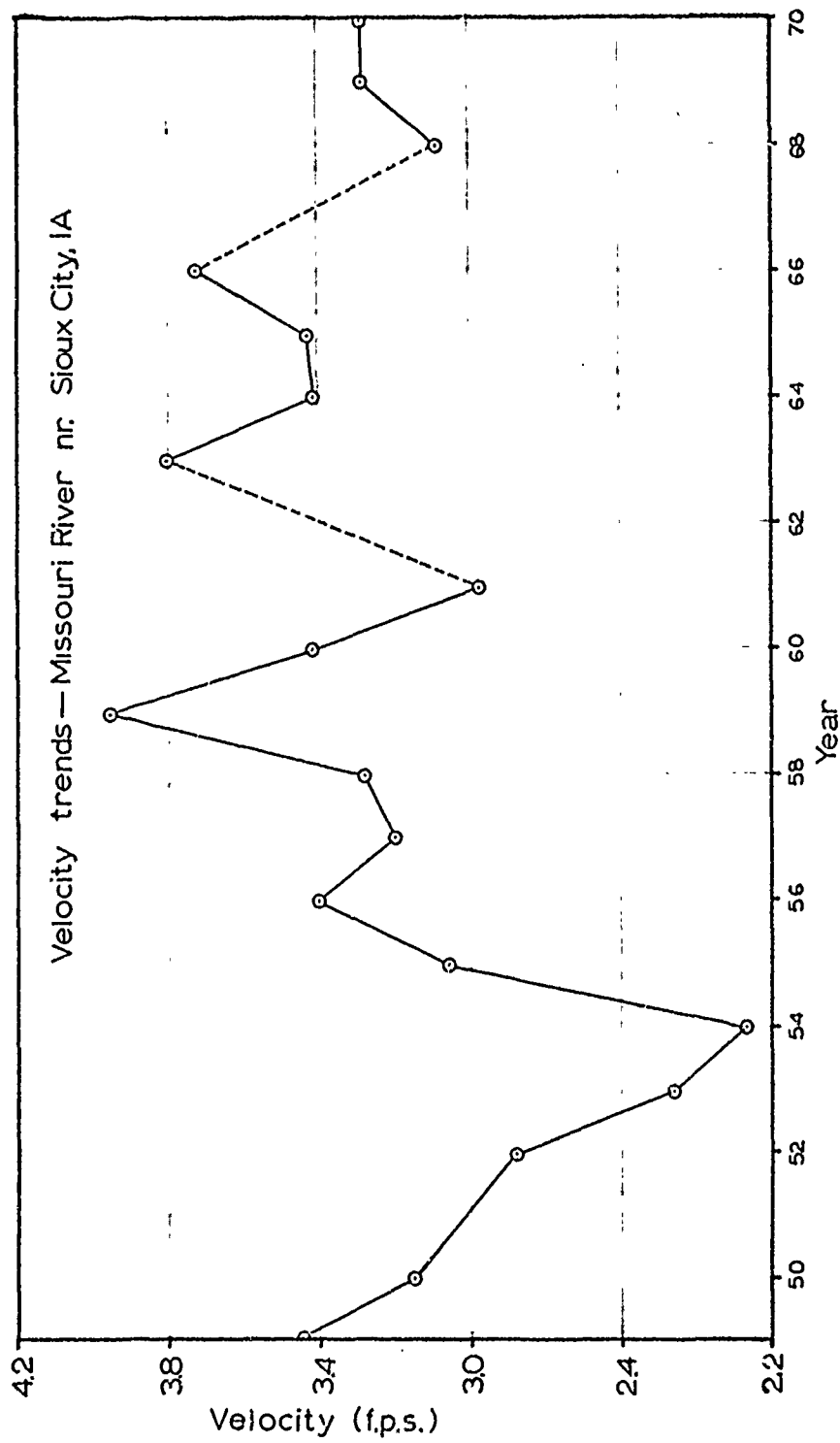
FIGURE 9. MISSOURI RIVER VELOCITY TRENDS
