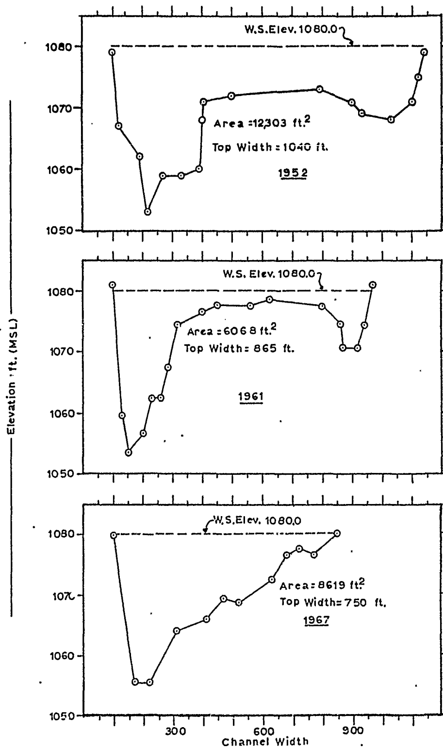
FIGURE 4. CHANNEL CROSS SECTION HISTORY AT RIVER MILE 731.49
