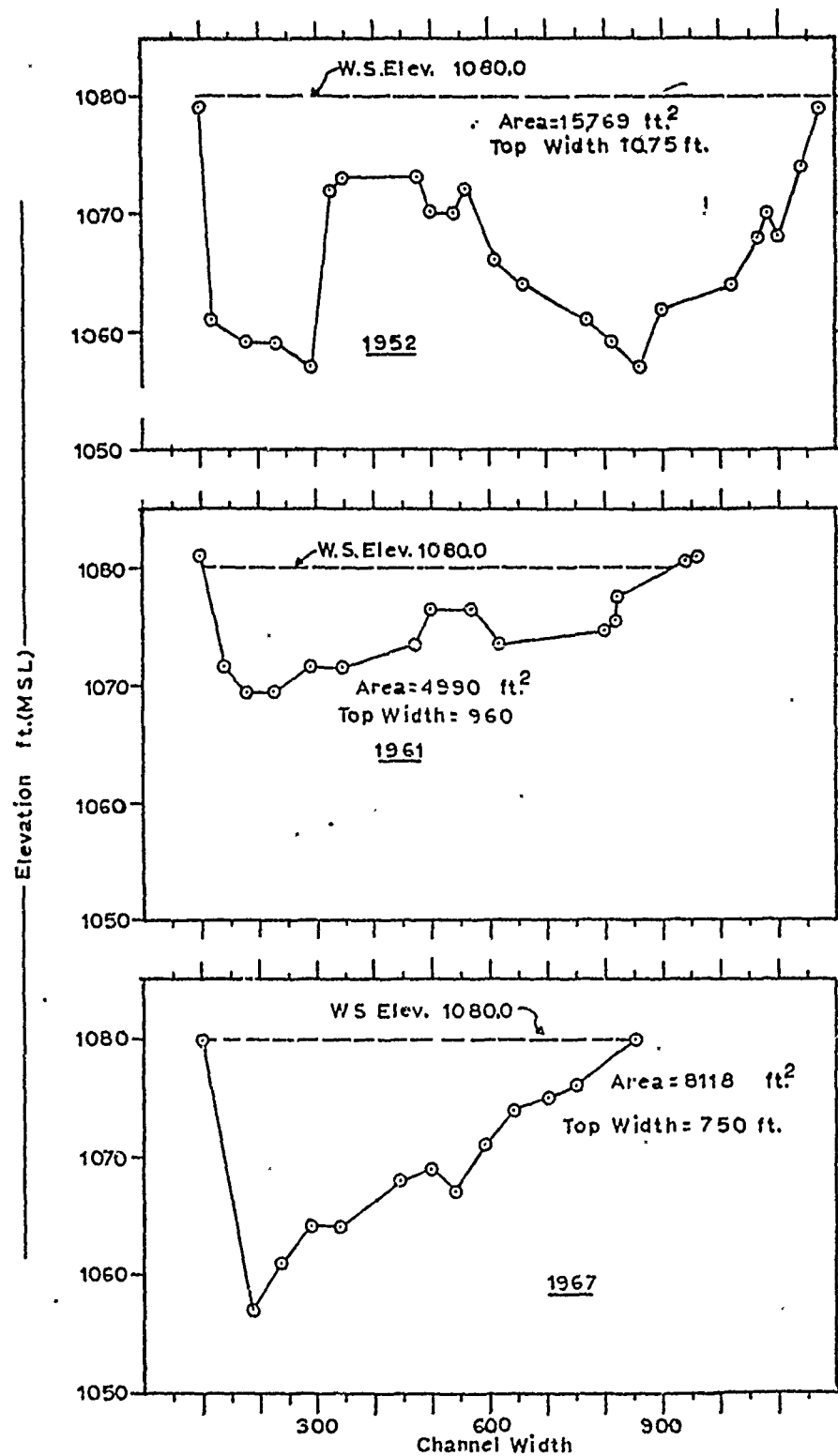
FIGURE 3. CHANNEL CROSS SECTION HISTORY AT RIVER MILE 731.7
