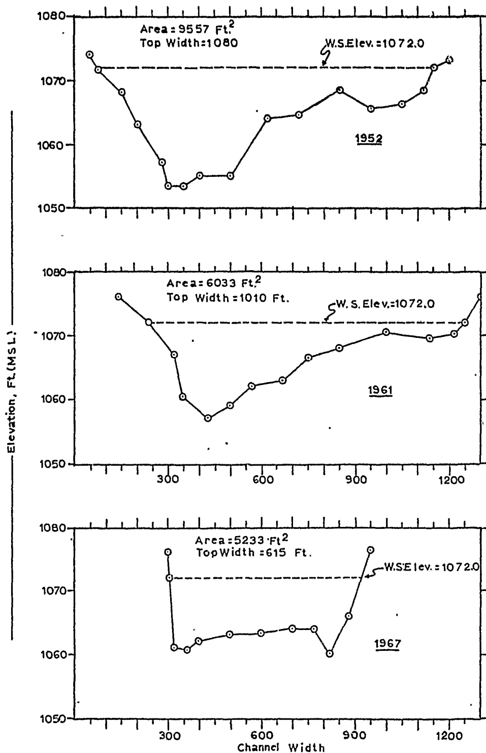
FIGURE 5. CHANNEL CROSS SECTION HISTORY AT RIVER MILE 727.9
