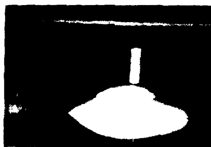
Initial Cavitation on Neck at 21.0 knots
