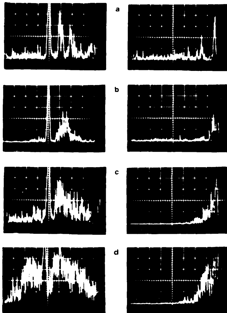
Figure 8. Plasma wave structure transition to turbulent conditions. Vertical and horizontal scales same as Fig. 7. a) \eta = .009 , breakdown of fine structure and high level of background noise in both electron plasma wave and ion acoustic wave measurements. b) \eta = .010 , broadband of frequencies driven near original plasma waves for both electron plasma waves and ion acoustic waves. c) \eta = .020 , and d) \eta = .040 , turbulent electron plasma waves and ion acoustic waves.
