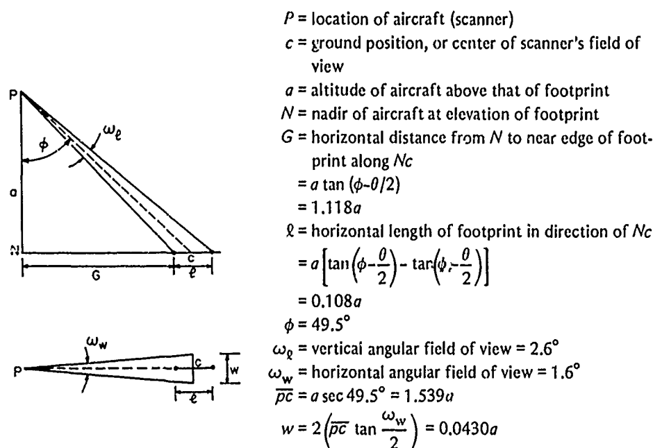
Figure 9. PMIS scanning geometry, and formulae for footprint determination.
