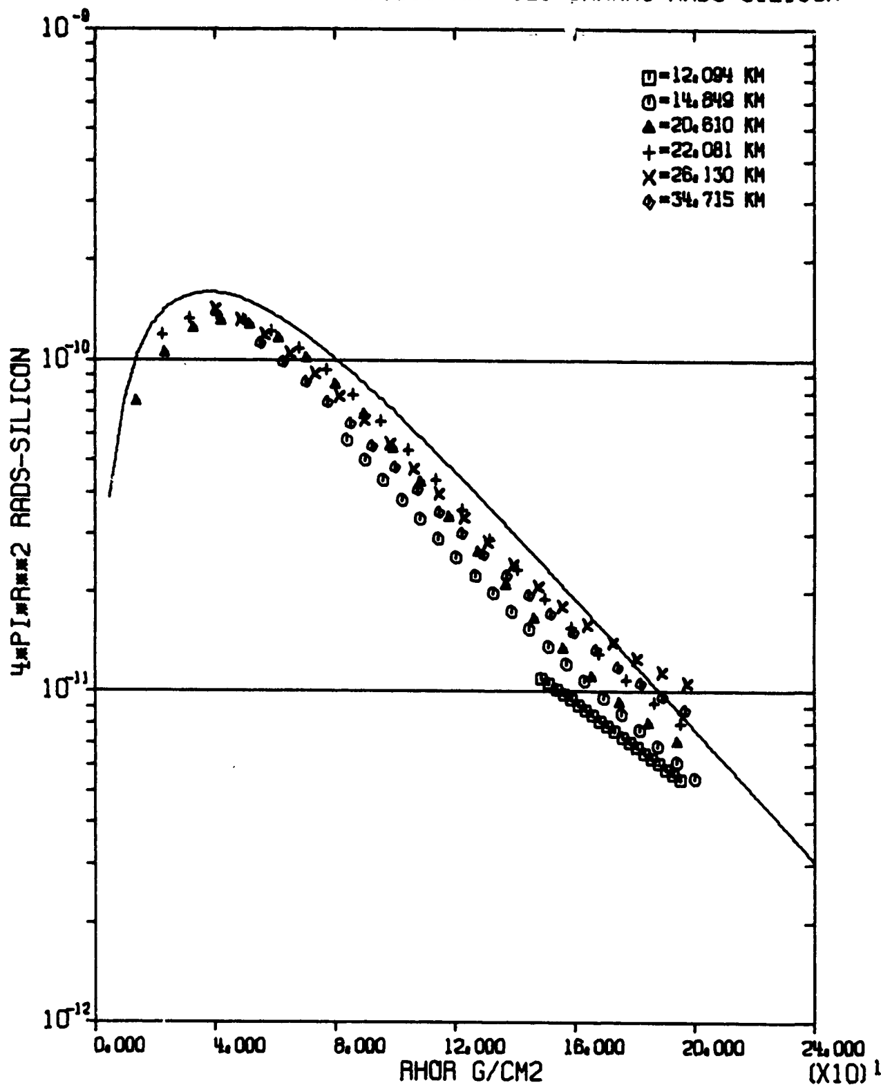
FIGURE C-55 MORSIAK FIT DATA-4PIR**2 GAMMA SI DOSE, THERMONUCL SOURCE IN REAL AIR AT 20.0 KM. ALL SAMPLING ALTITUDES
