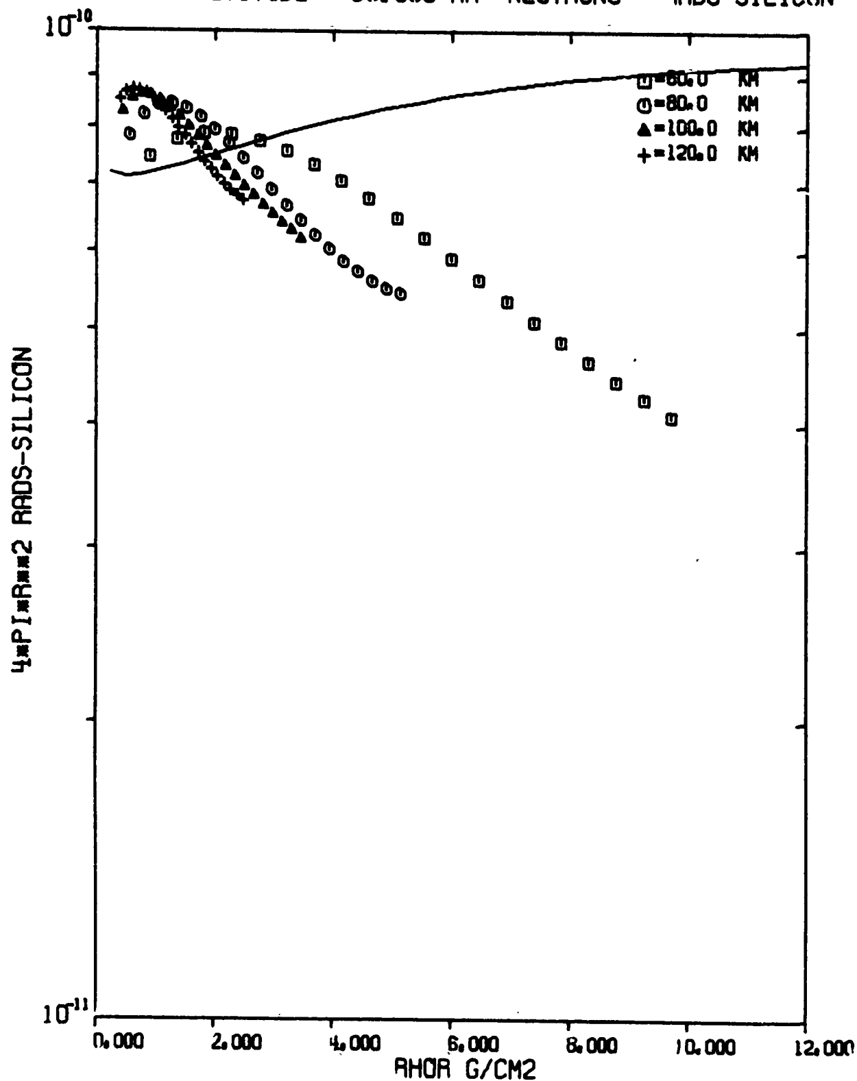
FIGURE C-53 MOKSAIR FIT DATA-4PIR**2 NEUTRON SI DOSE, FISSION. SOURCE IN REAL AIR AT 60.0 KM. SAMPLING ALTITUDES 60, 80, 100, AND 120 KM.
