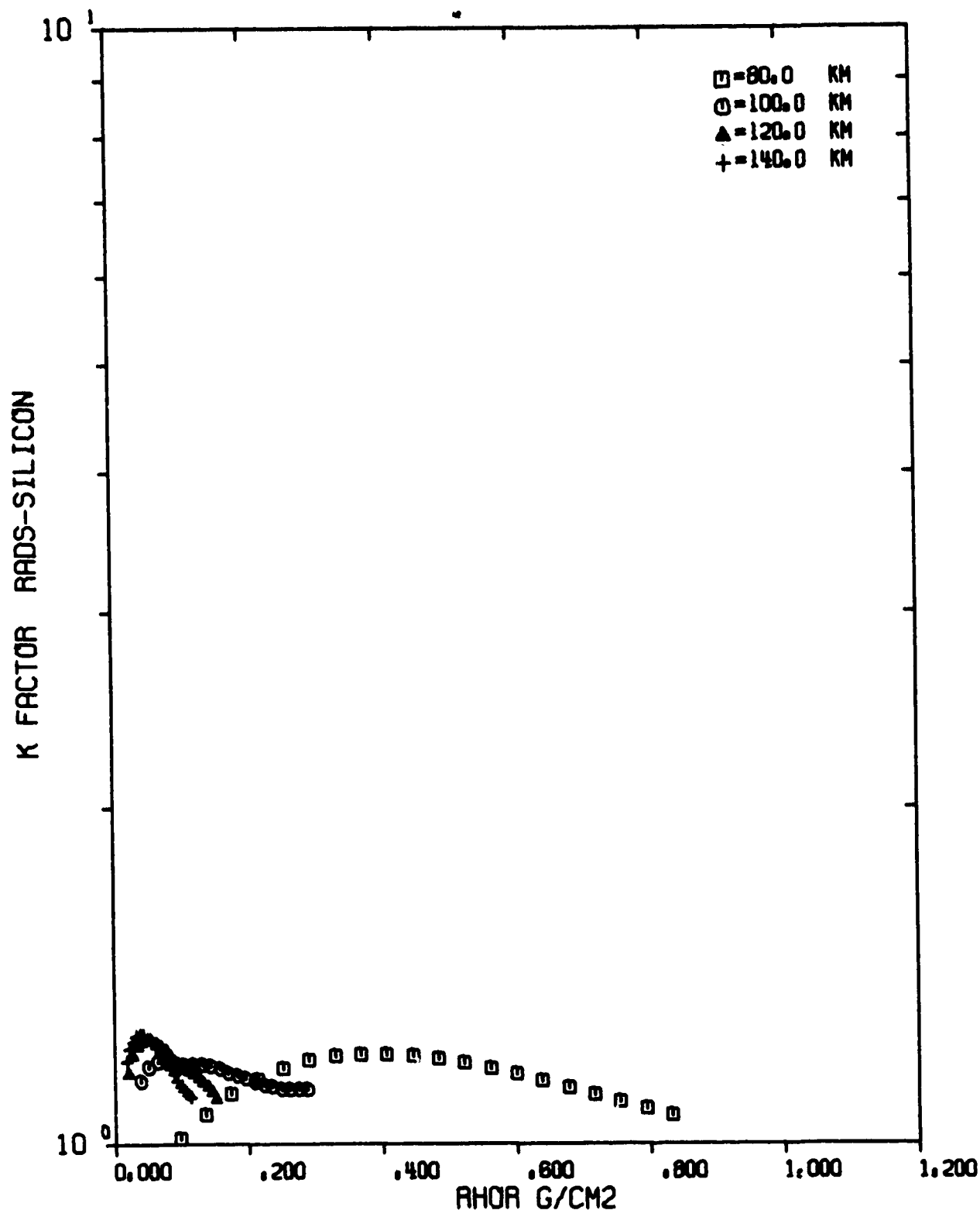
FIGURE C-46 MORSRIR FIT DATA-NEUTRON SILICON K-FACTOR FISSION SOURCE IN REAL AIR AT 80.0 KM. SAMPLING ALTITUDES 80, 100, 120, AND 140 KM.
