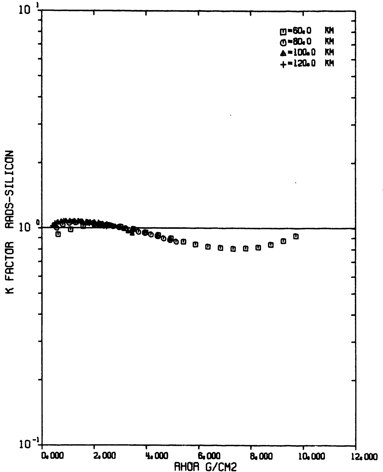
FIGURE C-70 MORSAR FIT DATA-NEUTRON SILICON K-FACTOR THERMONUCL SOURCE IN REAL AIR AT 60.0 KM. SAMPLING ALTITUDES 60,80,100, AND 120 KM.
