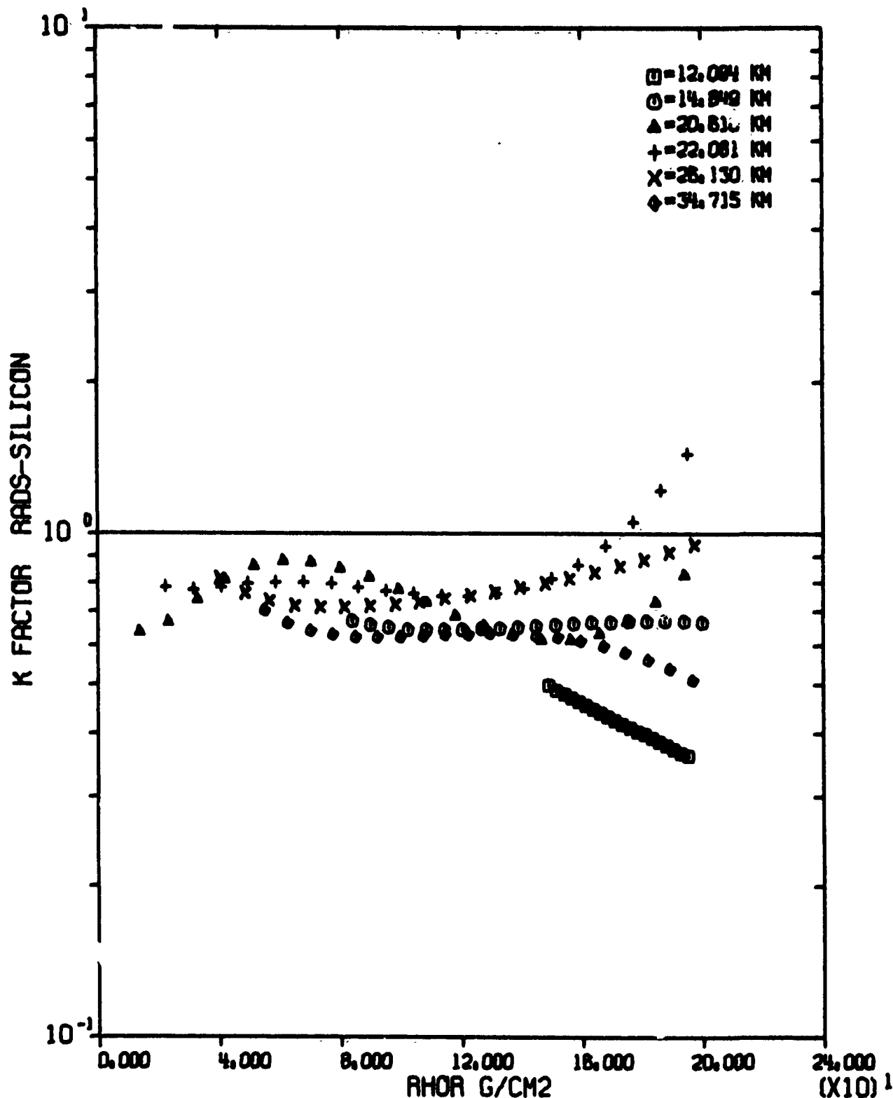
FIGURE C-20 MORSARK FIT DATA-GAMMA SILICON K-FACTOR, FISSION SOURCE IN REAL AIR AT 20.0 KM. ALL SAMPLING ALTITUDES
