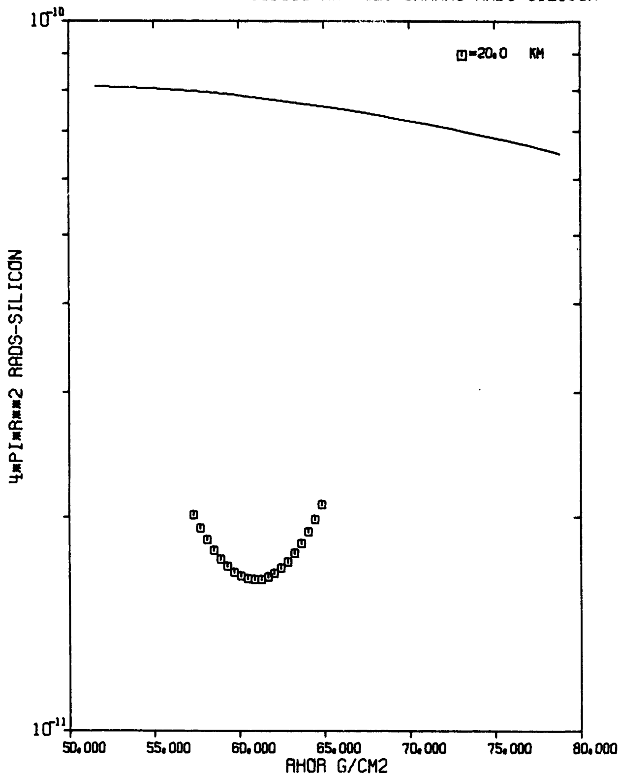
FIGURE C-39 MORSAR FIT DATA-4PIR**2 GAMMA SI DOSE, FISSION SOURCE IN REAL AIR AT 80.0 KM. SAMPLING ALTITUDES 20 KILOMETERS.
