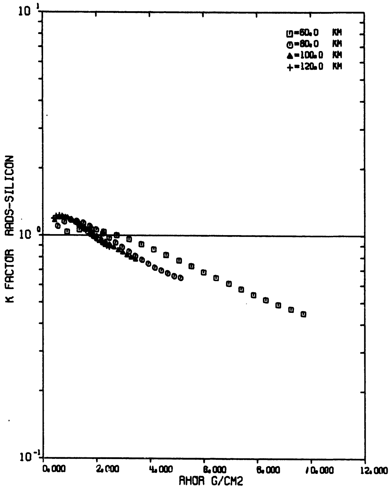
FIGURE G-34 MORSARK FIT DATA-NEUTRON SILICON K-FACTOR FISSION SOURCE IN REAL AIR AT 60.0 KM. SAMPLING ALTITUDES 60, 80, 100, AND 120 KM.
