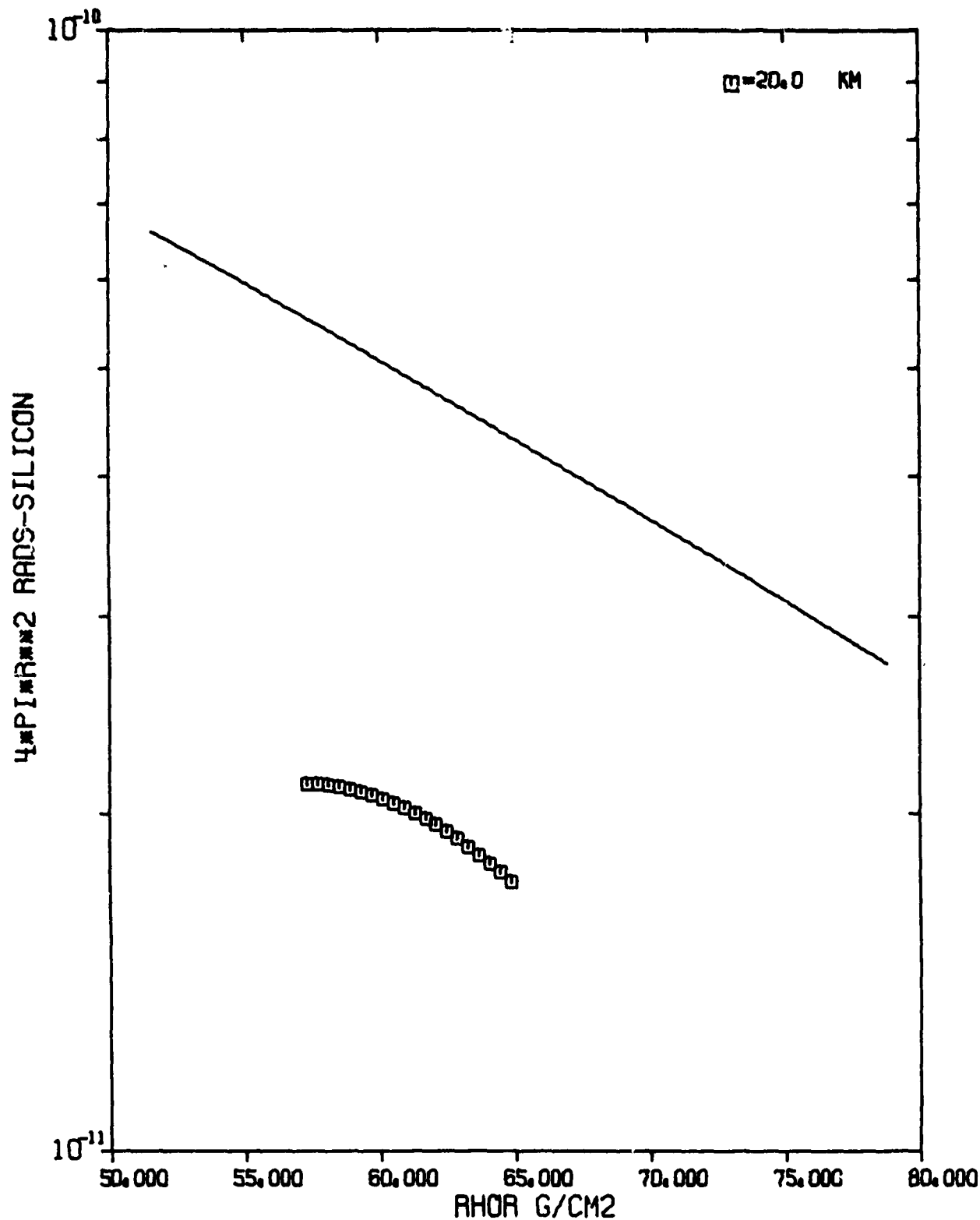
FIGURE 3-73 MORS4IR FIT DATA-4PIR**2 NEUTRON SI DOSE, THERMONUCL SOURCE IN REAL AIR AT 80.0 KM. SAMPLING ALTITUDES 20 KILOMETERS.
