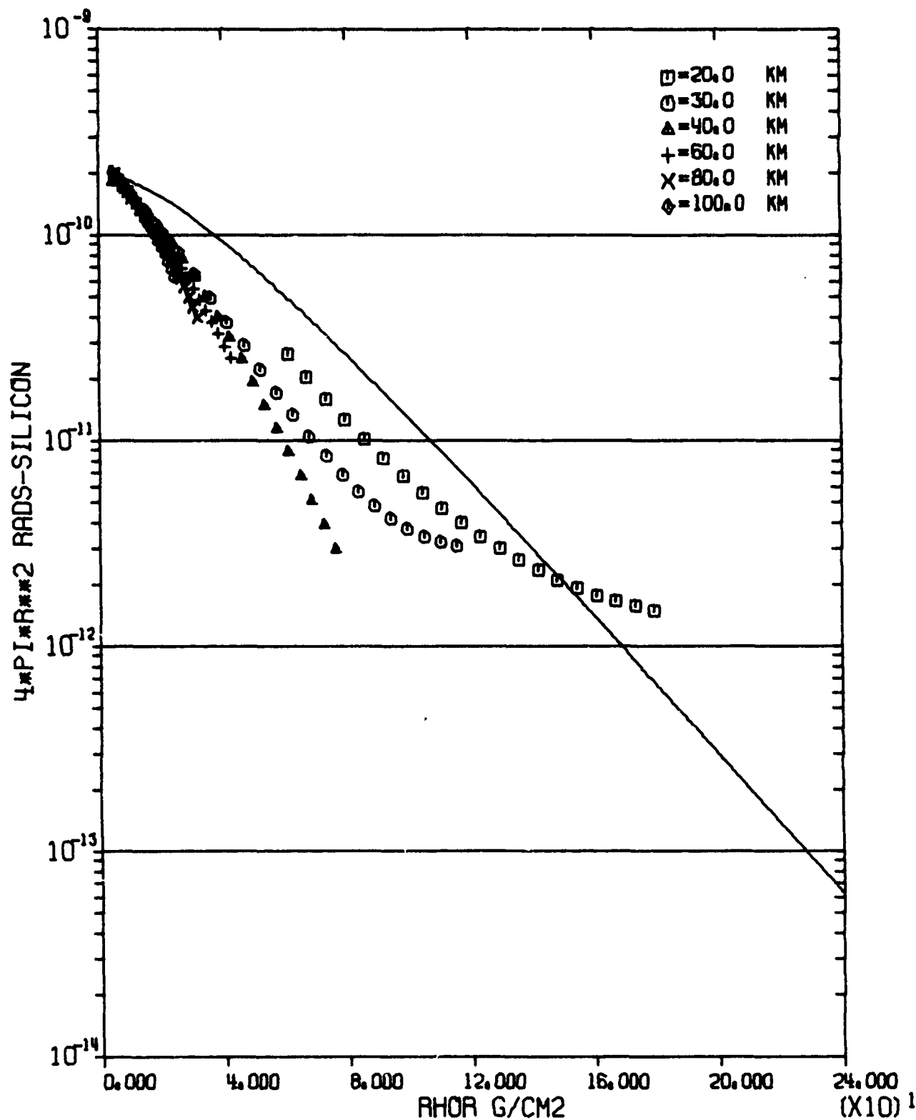
FIGURE G-61 MORSAR FIT DATA-4PIR**2 NEUTRON SI DOSE, THERMONUCL SOURCE IN REAL AIR AT 40.0 KM. ALL SAMPLING ALTITUDES
