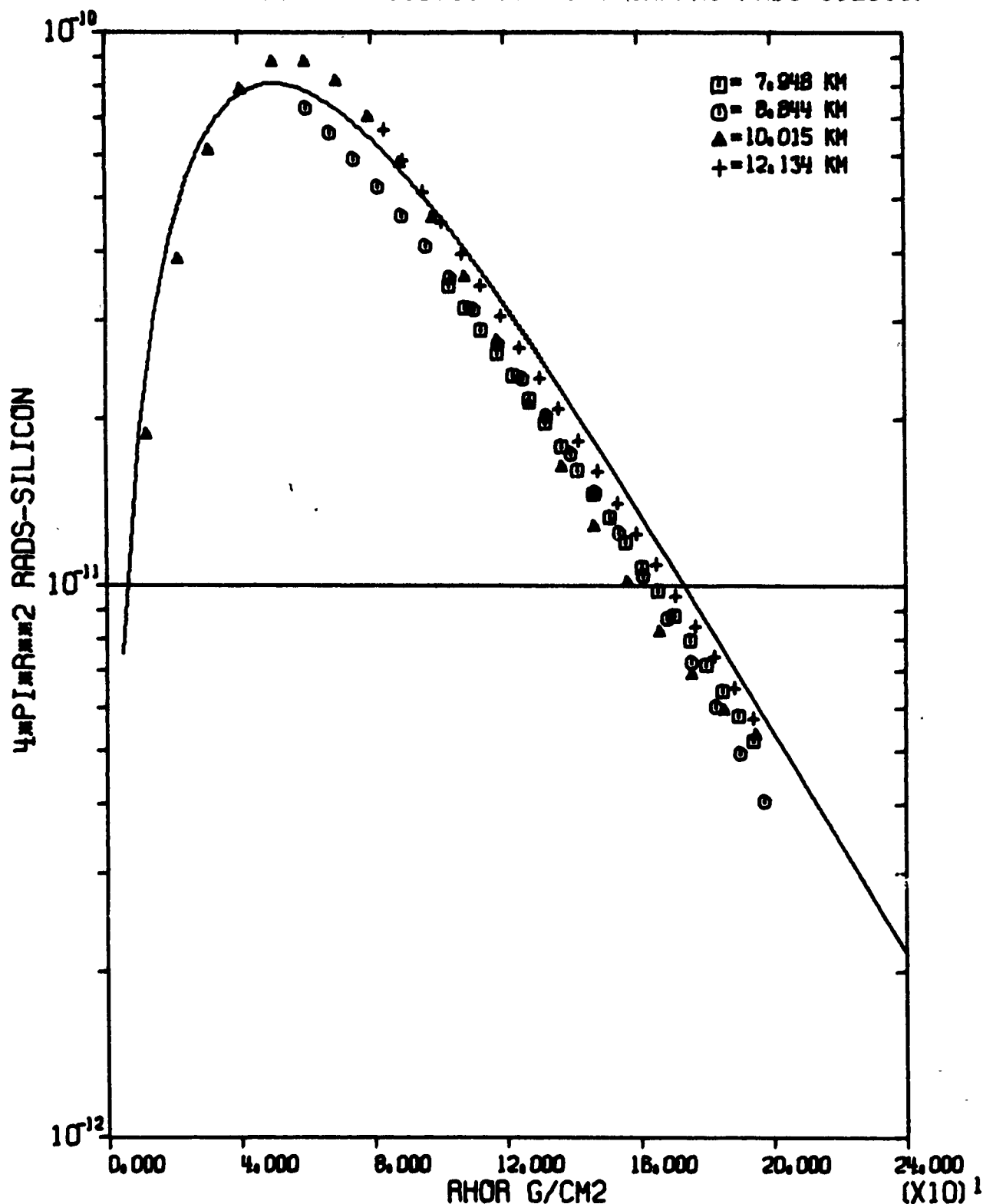
FIGURE C-11 MORSAR FIT DATA-4PIR**2 GAMMA SI DOSE, FISSION SOURCE IN REAL AIR AT 10.0 KM. ALL SAMPLING ALTITUDES
