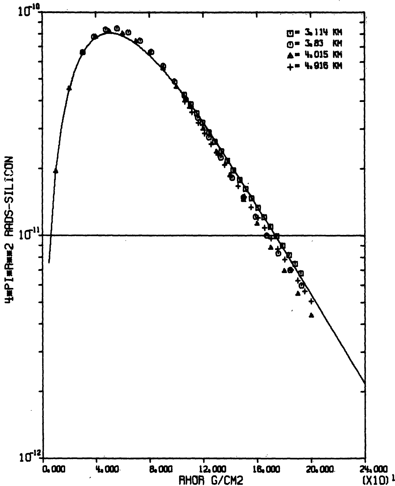
FIGURE C-3 MOKSAIR FIT DATA-4PIR**2 GAMMA SI DOSE, FISSION SOURCE IN HOMO AIR AT 4.0 KM. ALL SAMPLING ALTITUDES
