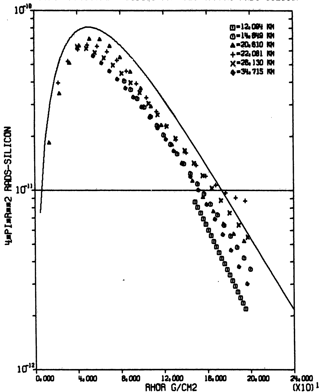
FIGURE C-19 MORSRIR FIT DATA-4PIR**2 GAMMA SI DOSE, FISSION SOURCE IN REAL AIR AT 20.0 KM. ALL SAMPLING ALTITUDES
