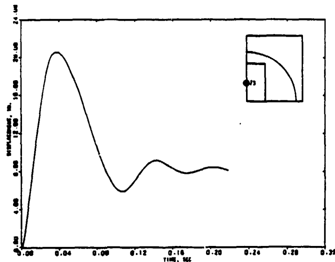
(a) Displacement
