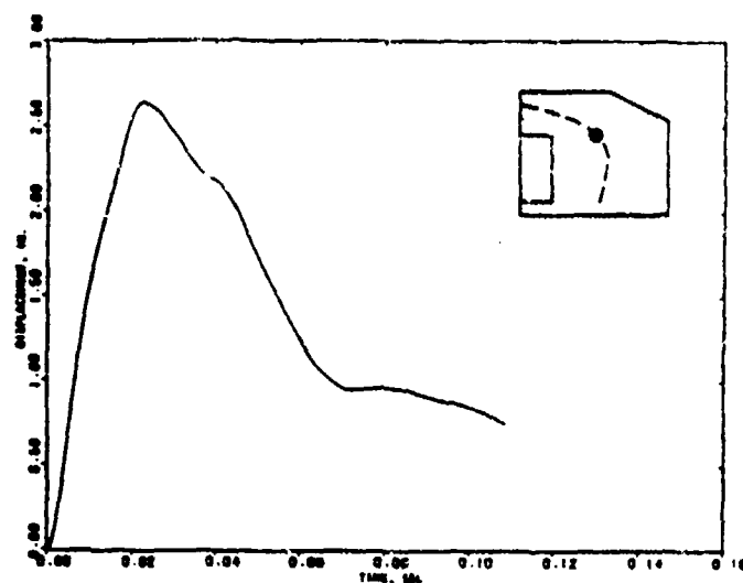
(a) Displacement
