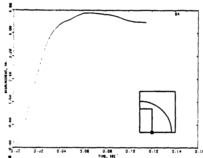
(a) Displacement
