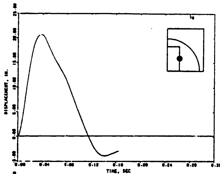
(a) Displacement
