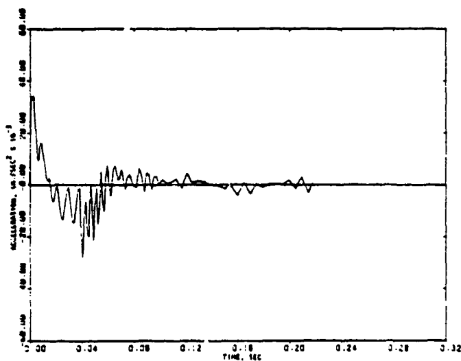
FIGURE 5-4. COMPUTED MOTION OF SOUTH AND WEST IGLOOS AT NODE 49 (Refined ESKIMO-1 calculation)
