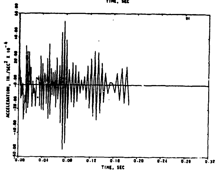
FIGURE 5-63. COMPUTED MOTION OF NORTHEAST IGLOO (ESKIMO IV) AT NODE 91
