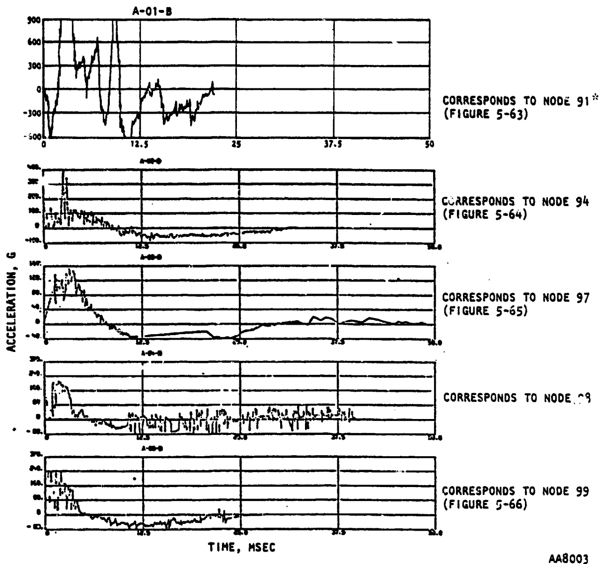
FIGURE 5-72. MEASURED ACCELERATION TIME HISTORIES OF NORTHEAST HE LL OF ESKIMO IV (Ref. 6)
