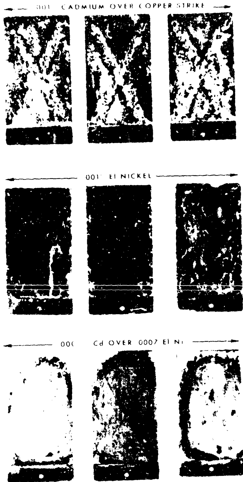
Figure 6. Results of 168 hour \text{SO}_2 -Salt Spray Exposure
