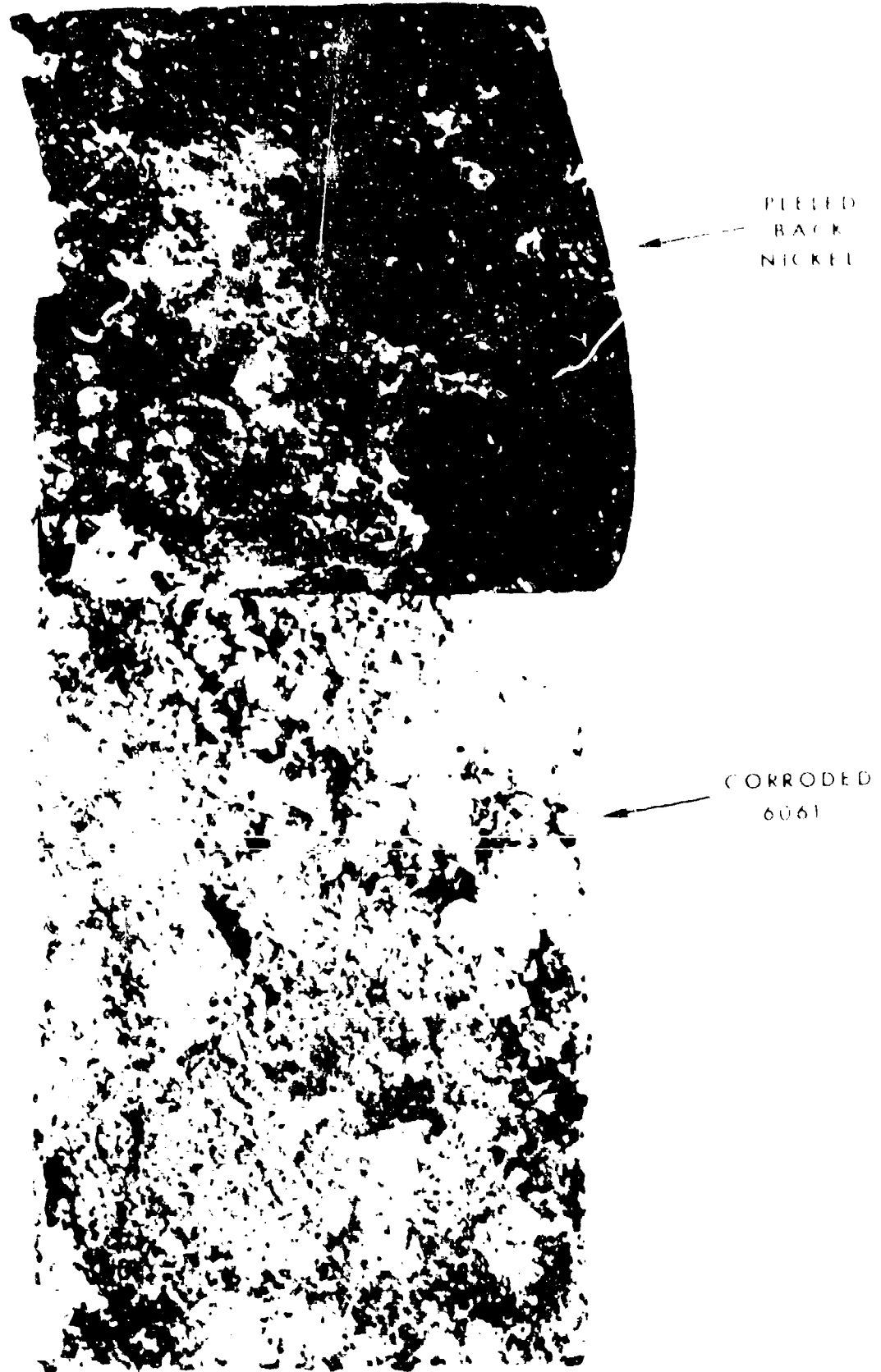
Figure 7. Electroless Nickel .001" over 6061 Aluminum Alloy - 168 hours Exposure to SO 2 -Salt Spray
