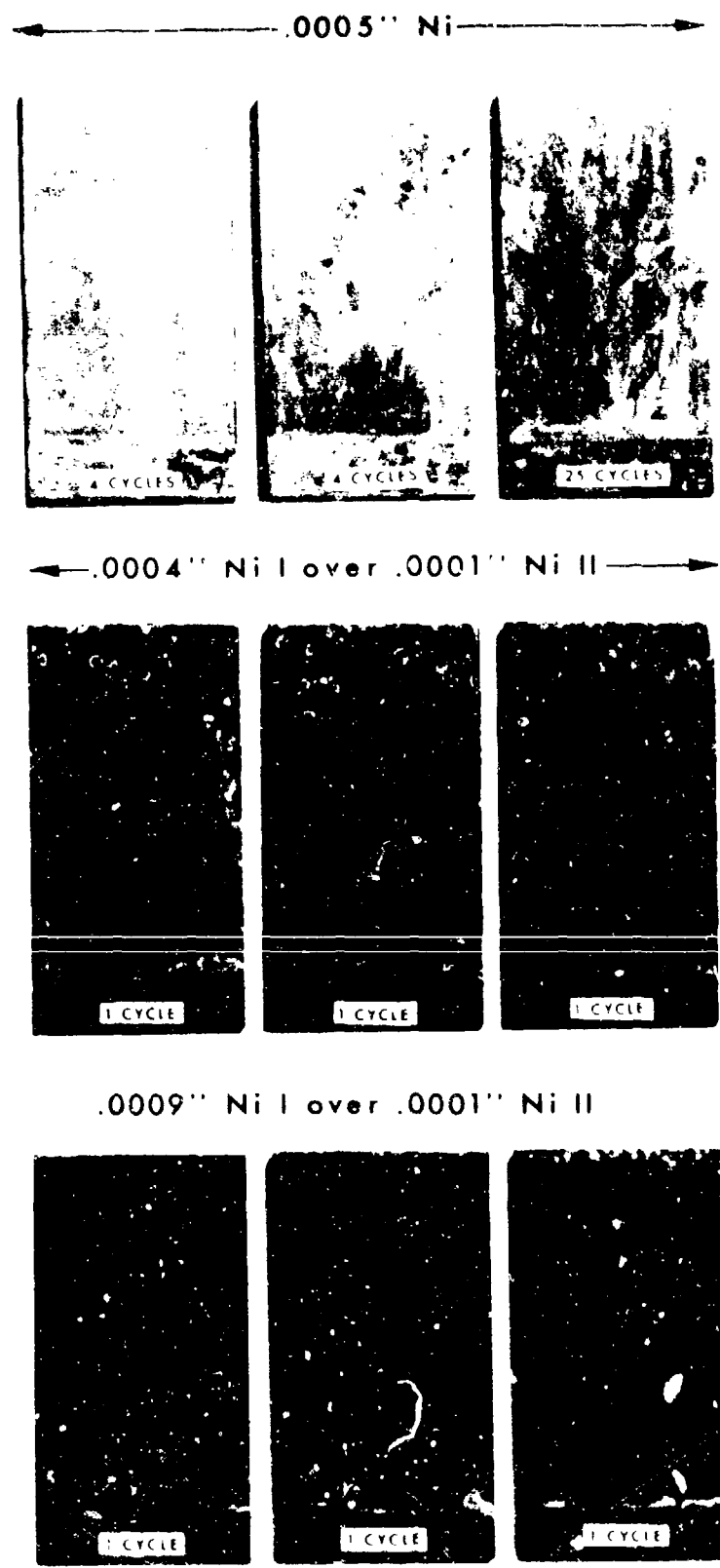
Figure 3. CYCLIC HEATING/CORROSION RESULTS Electroless Nickel Coatings
