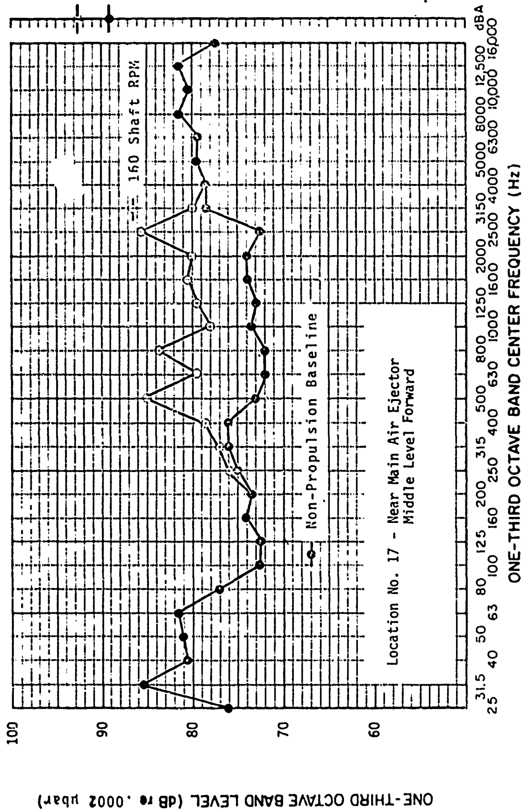
FIGURE 5: USS ELMER MONTGOMERY PRE-RAV NOISE TRIALS MEASUREMENT LOCATION NO. 17 IN ENGINE ROOM
