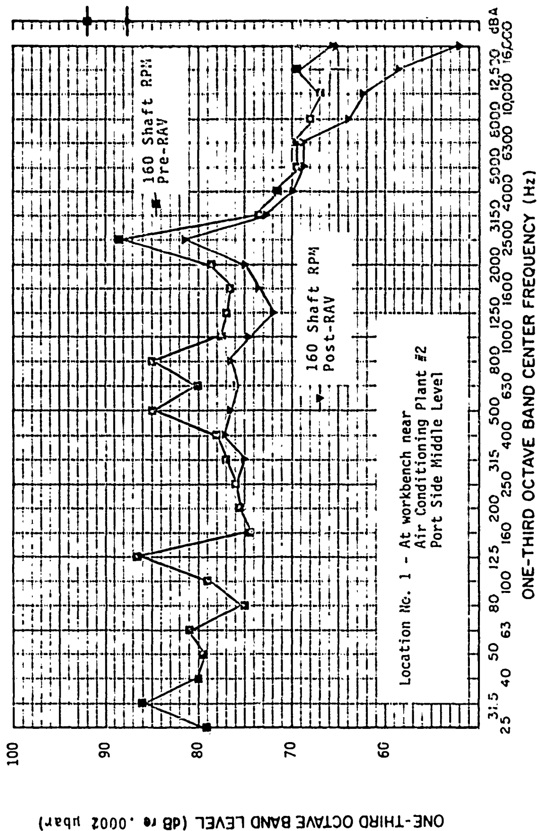
FIGURE 18: COMPARISON OF PRE-AND POST-RAV NOISE TRIALS MEASUREMENT LOCATION NO. 2 IN ENGINE ROOM
