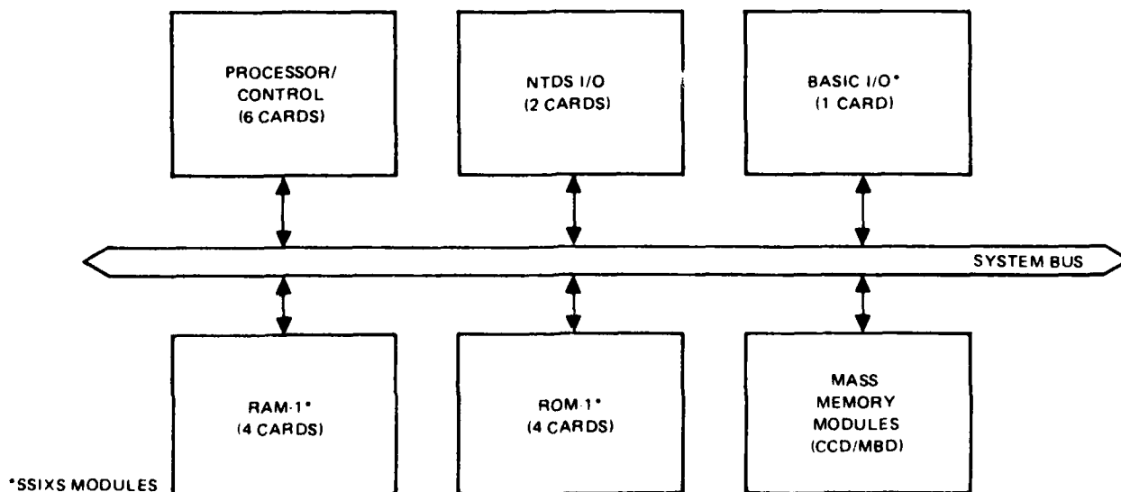
Figure 1. MIMC architecture.
