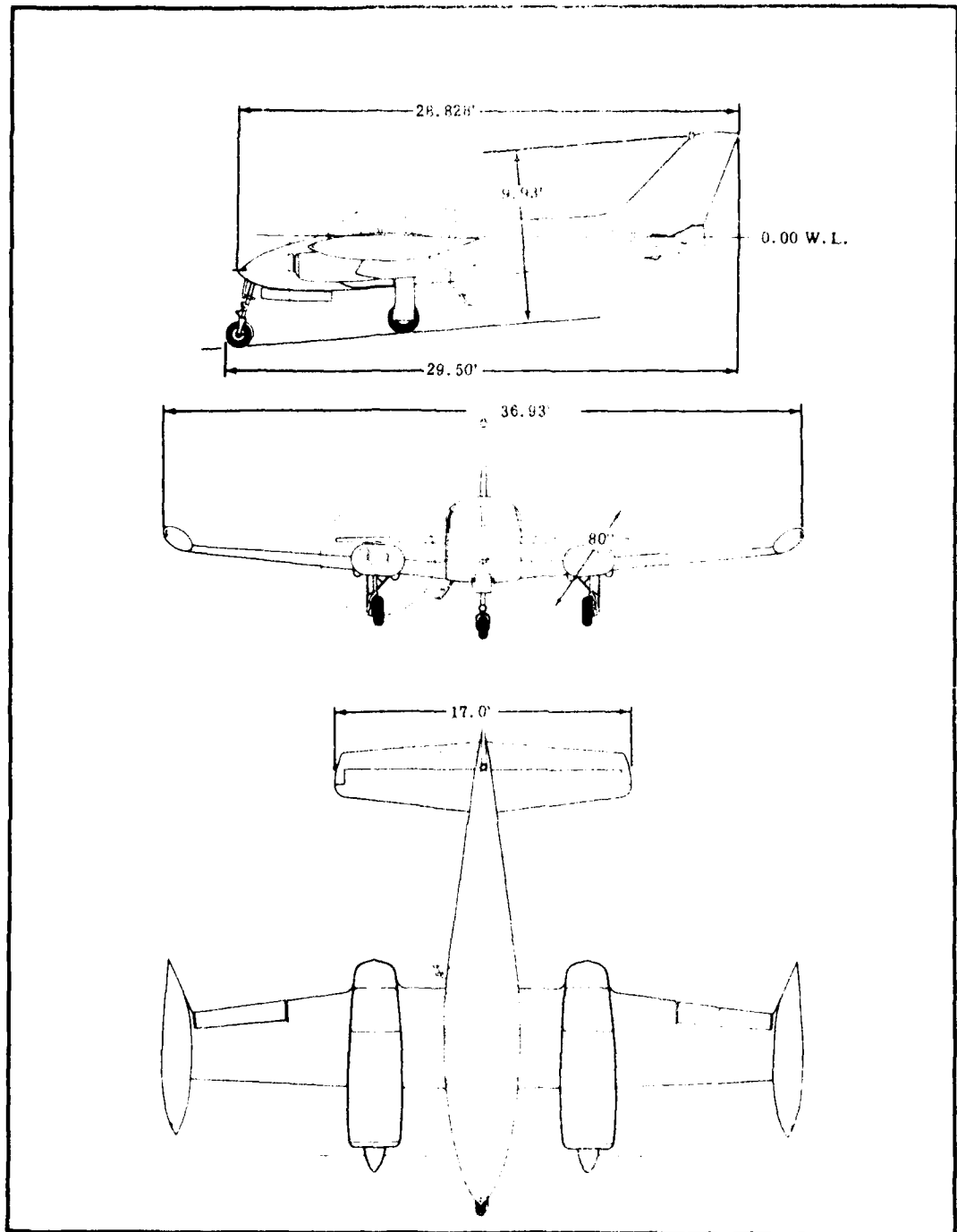
Figure 3. General dimensions of Model 310I Airplane.
