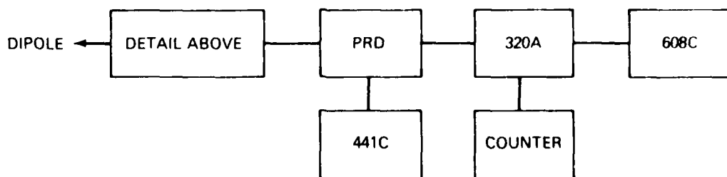
Fig. 8 — Test setup for antenna impedance measurements
