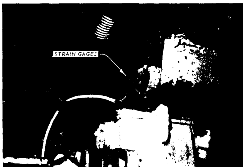
Figure 27. Crane equalizer bar (3-1/2 in. by 4-1/4 in.) with strain gages installed
