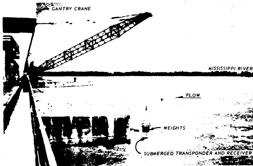
Figure 15. Surveying the scour hole, 5 May 1973
