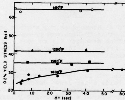
FIG. 2 Yield strength of TD-Nichrome as a function of time at temperature, following rapid heating.
