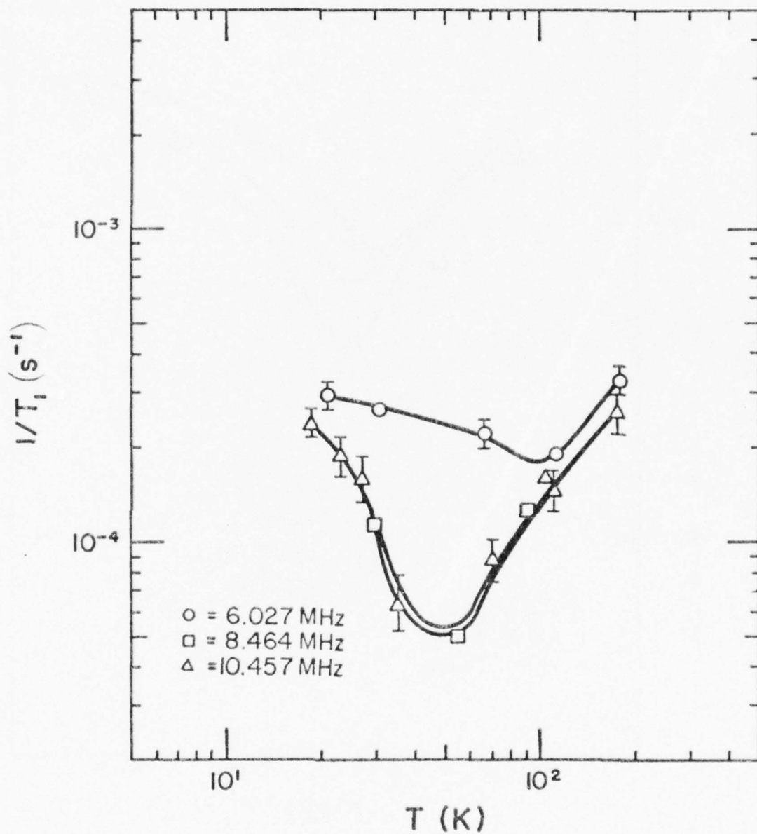
Figure 15. 29 Si spin-lattice relaxation rate vs. temperature: 10-15 after irradiation, before annealing
