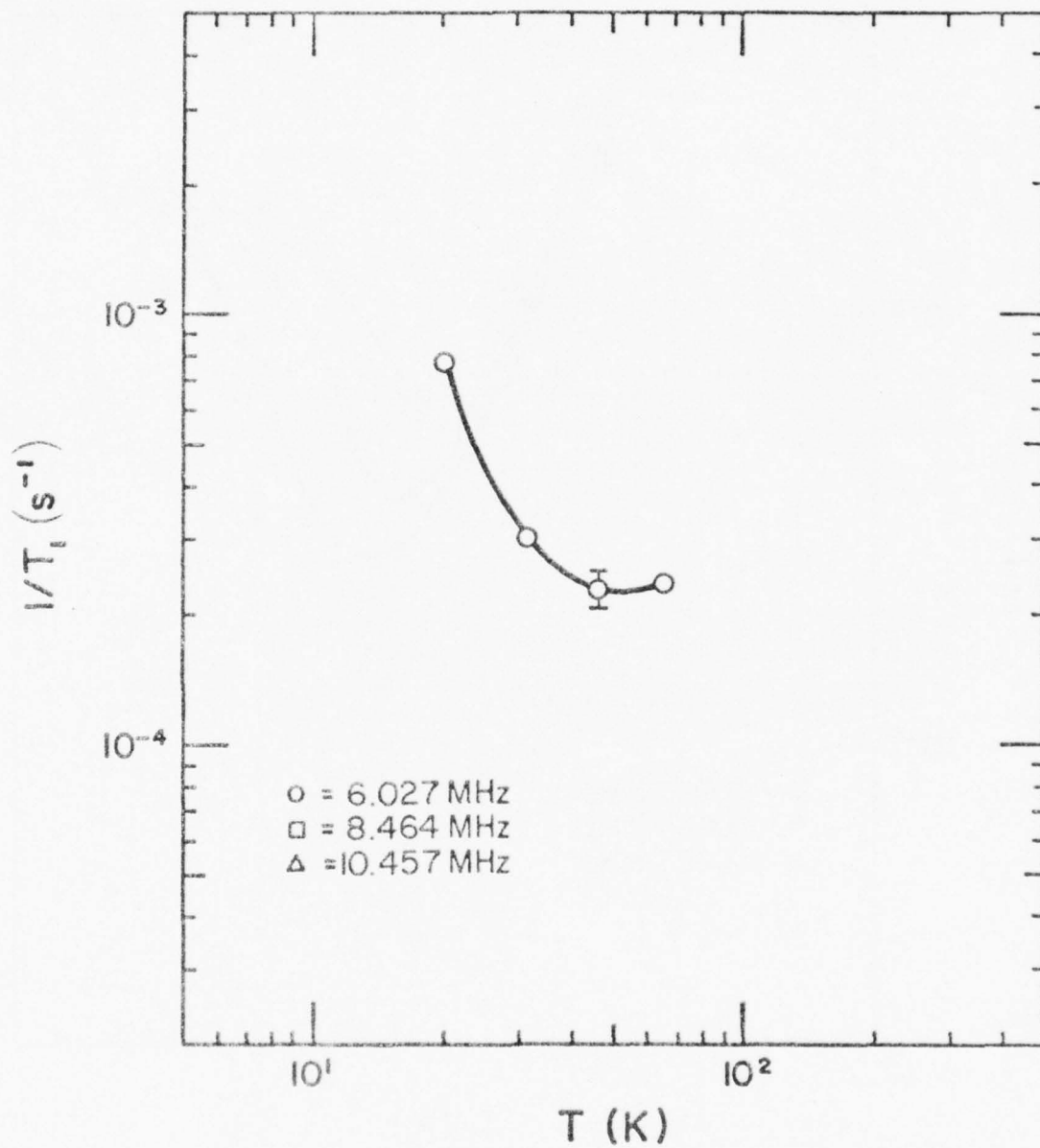
Figure 14. ^{29}\text{Si} spin-lattice relaxation rate vs. temperature: 1-15 after irradiation, before annealing
