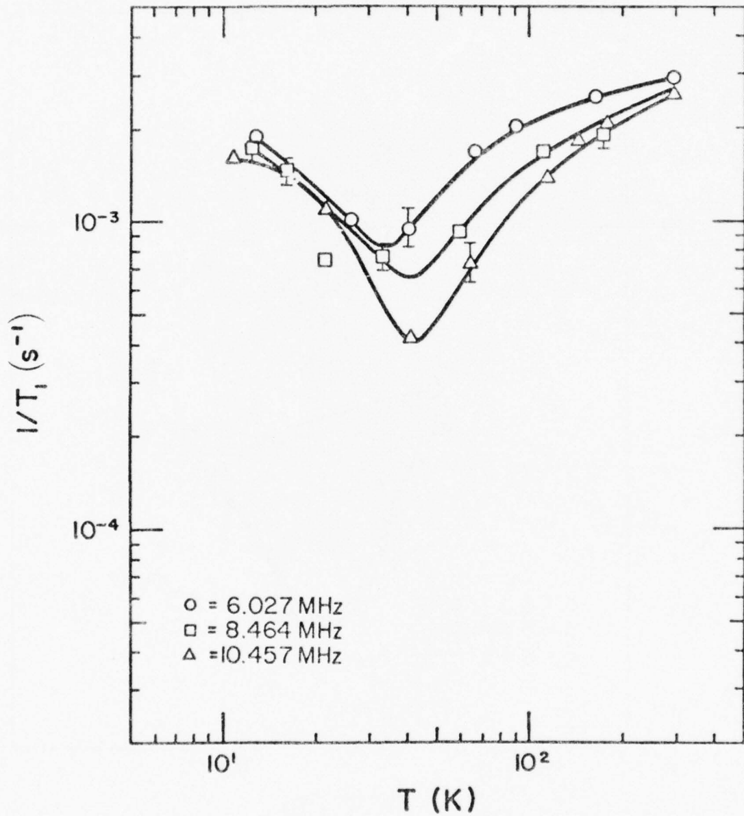
Figure 16. 29 Si spin-lattice relaxation rate vs. temperature: 10-17 after irradiation, before annealing
