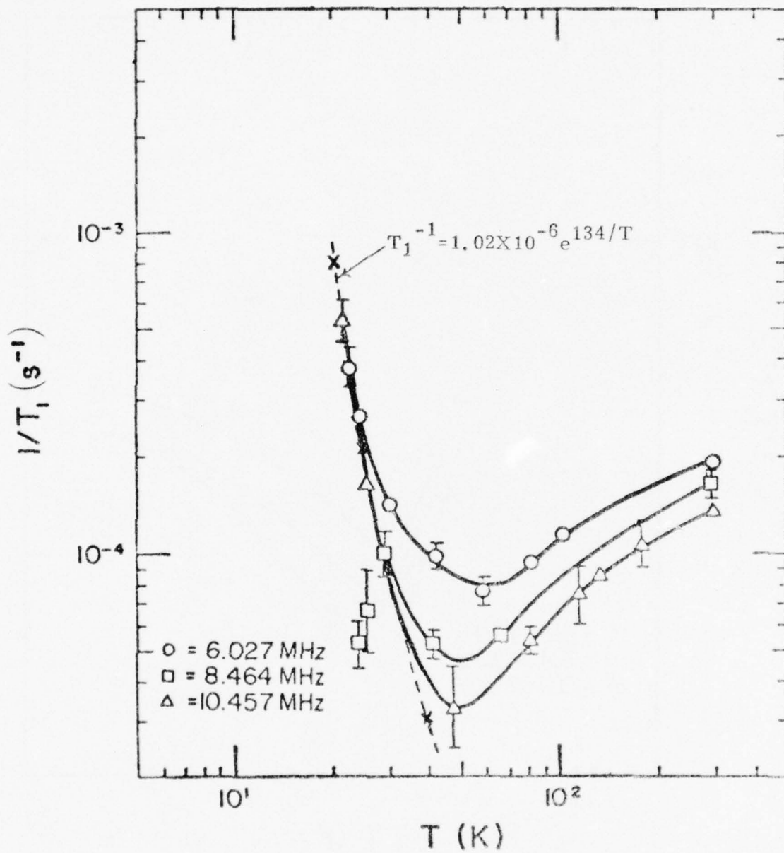
Figure 7. ^{29}\text{Si} spin-lattice relaxation rate vs. temperature: l-o before irradiation
