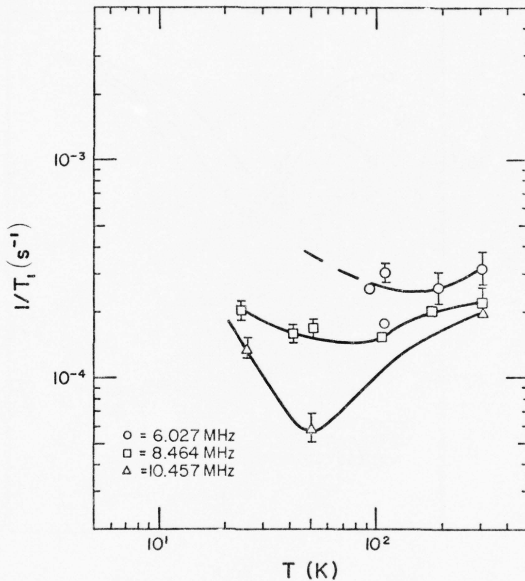
Figure 9. 29 Si spin-lattice relaxation rate vs. temperature: 10-15 before irradiation
