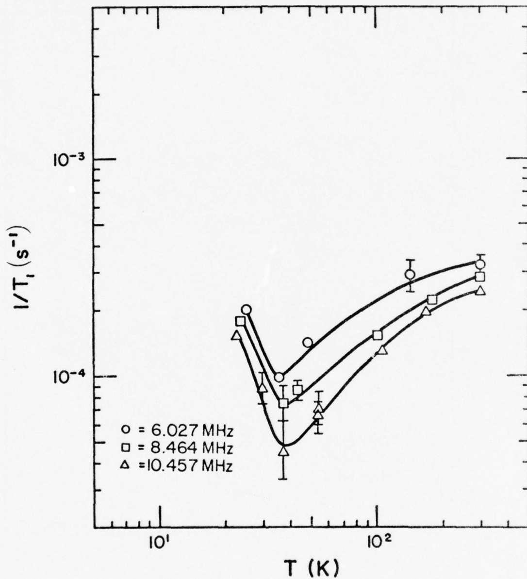
Figure 8. 29 Si spin-lattice relaxation rate vs. temperature: 1-15 before irradiation
