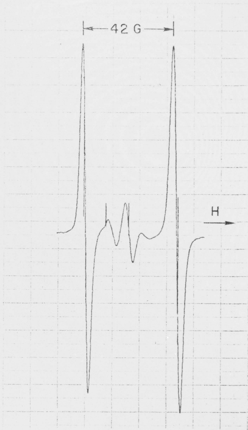
Figure 21. Derivative of P donor electron absorption at 6 K; single, double, and triple electron spectra are present
