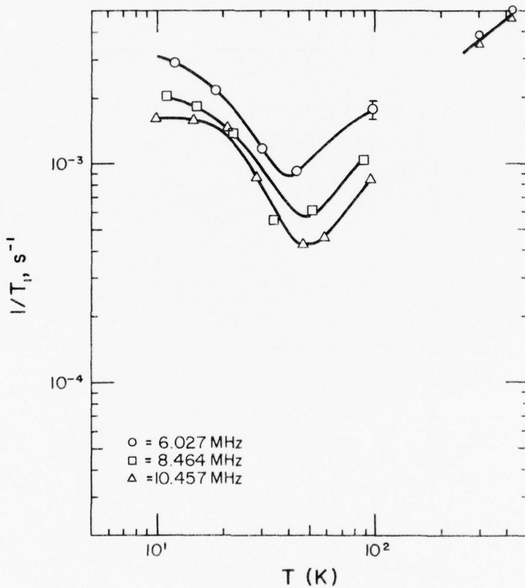
Figure 19. ^{28}\text{Si} spin-lattice relaxation rate vs. temperature: 10-17 after irradiation and 13 hours annealing
