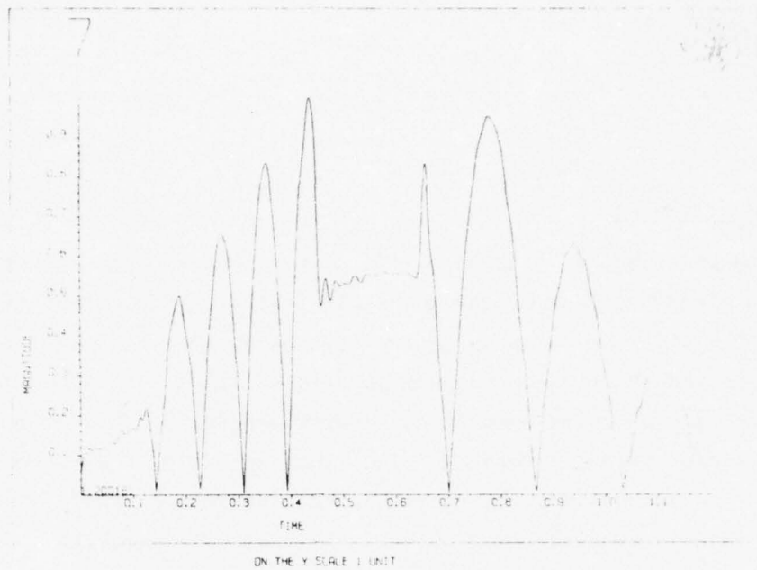
Figure 39(a) Envelope of the Time Domain Output of the TAPS System for the Three-Tone Input Signal of Figure 17 with -15 dB Gaussian Weighting
