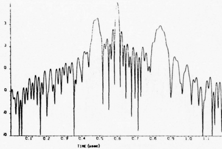
Figure 19(a) Typical Chirp Transform of the Three-Tone Input of Figure 18
