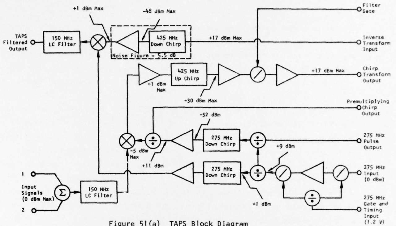
Figure 51(a) TAPS Block Diagram
