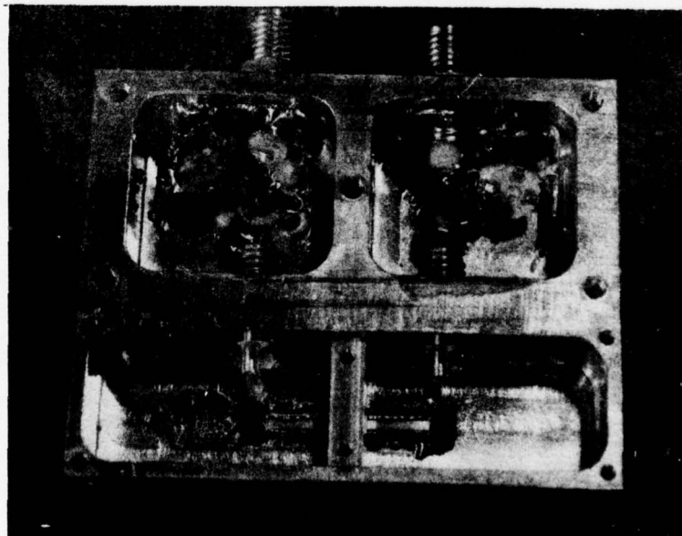
Figure 51(b) Packaged SAW Linear FM Filter
