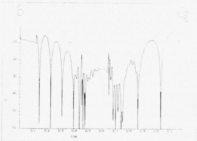
Figure 39(b) Difference Between the TAPS Input and Output Signals Normalized to the Signal Peak for -15 dB Gaussian Weighting
