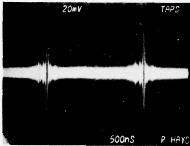
(a) B = 26 \text{ MHz} , T = 0.5 \mu\text{sec}
