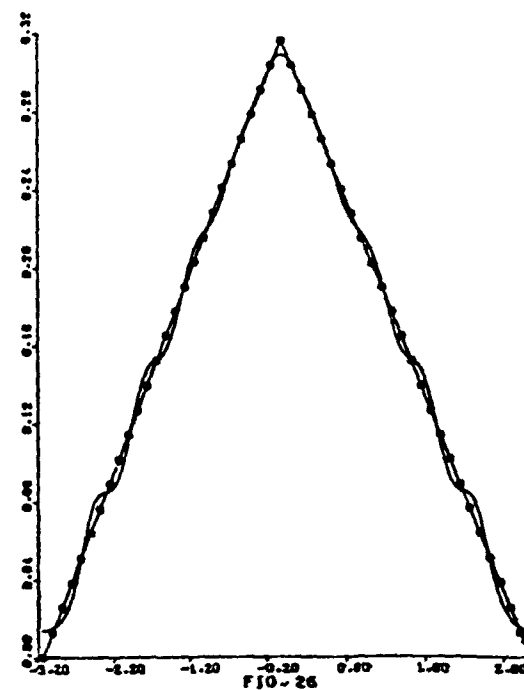
Triangular averaging orders 8 and 9
