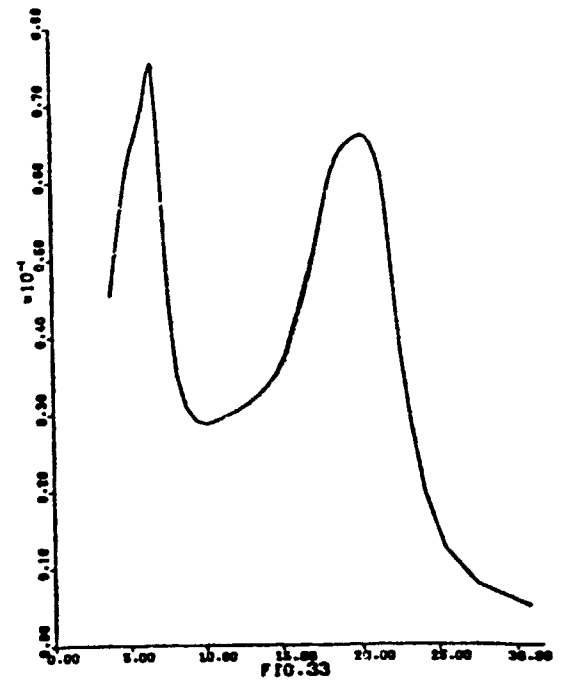
Spline SLP1 = 22
