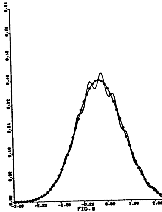
Normal (0.5,1) order 10
