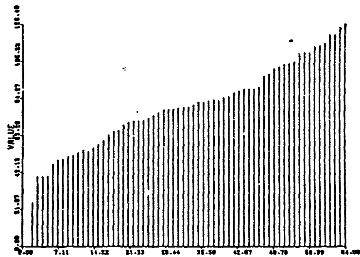
Figure A2 Same data ordered
