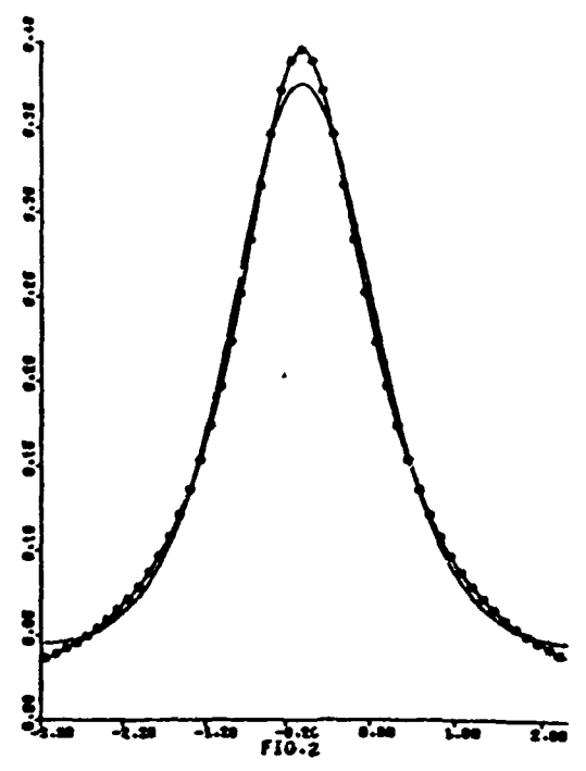
Cauchy order 2
