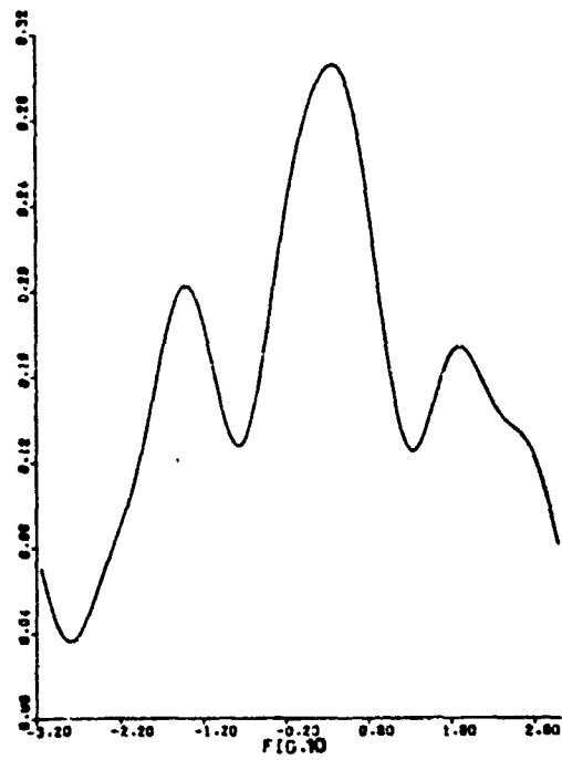
Sample characteristic function horizontal line at 0.016
