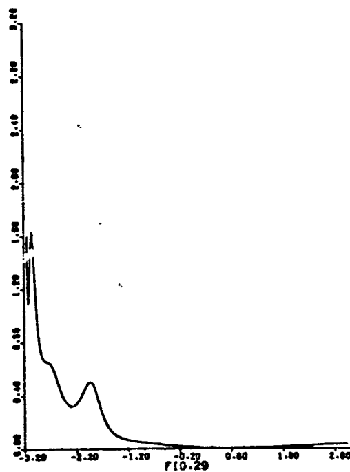
Square-root transformation order 2
