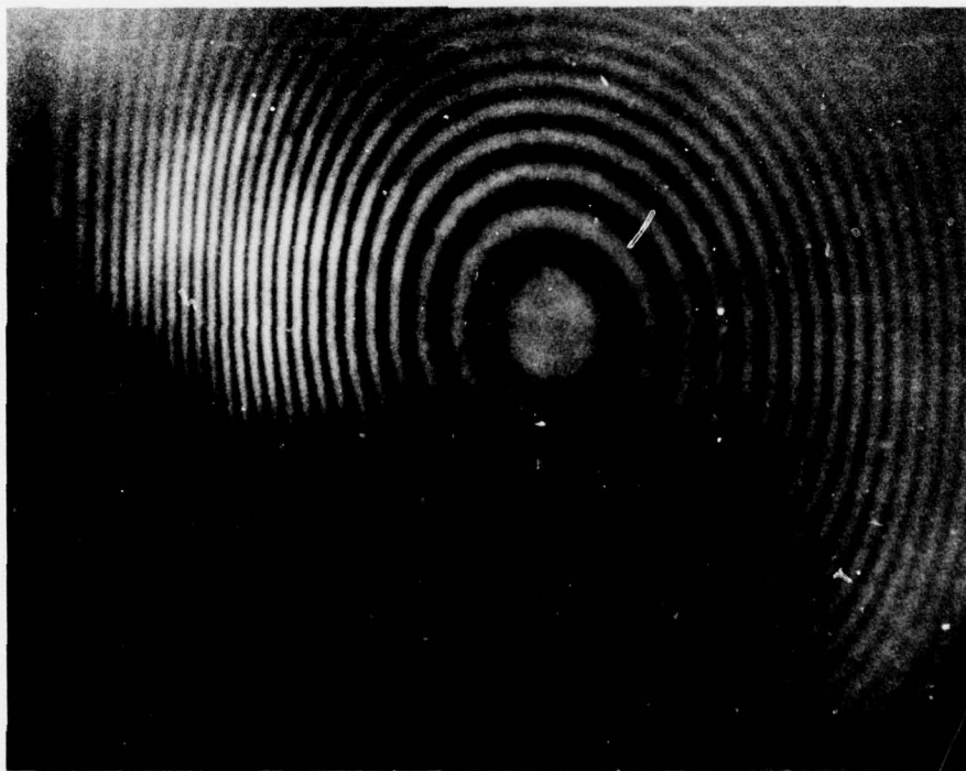
Figure 4. Typical Holographic Interferogram Obtained from the Central Region of a Plexiglass Cell (pressure = 5.15 \times 10^{-3} psi)
