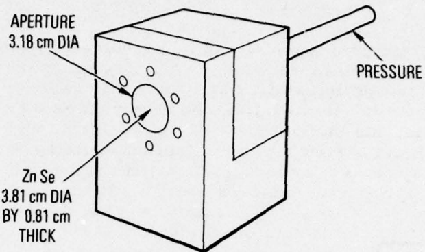
1a. Small Pressure Cell
