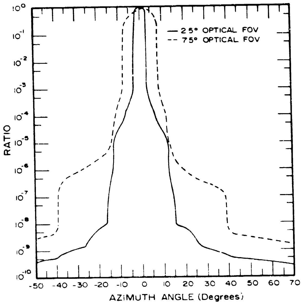
Figure 10. NR-1 baffle response as measured with 2.5° and 7.5° optical fields of view.
