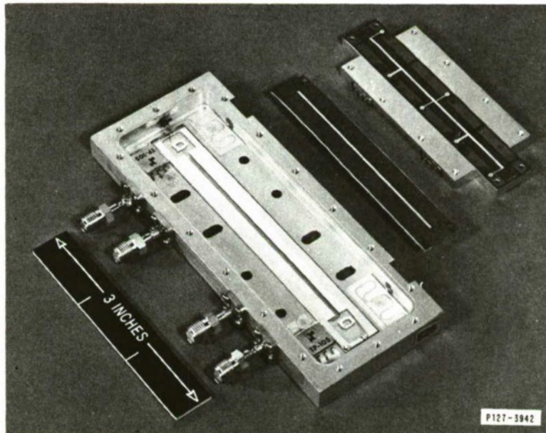
Fig.II-2. Three main convolver subassemblies. The base holds the \text{LiNbO}_3 delay line and matching networks. A Kapton sheet has the two silicon strips bonded to it. The Kapton circuit which provides the electrical interconnections to the silicon is attached to the pressure-plate assembly.
