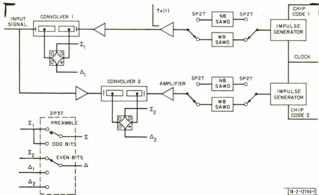
Fig.II-1. Convolver module schematic. The convolver module is used to interface the DPSK convolver with the input RF signal and digital chip codes. The module contains two SAW devices which are impulsed for either narrowband or wideband chip coding. An output switching network is used either to combine the convolvers during the preamble or to alternately select each of them during communications.
