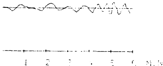
Fig. 8 Kongsberg NHI recordings 10 Dec 1972 and 23 July 1973 and crosscorrelation function. The correlation function peaks at a lag of 11 sek.
