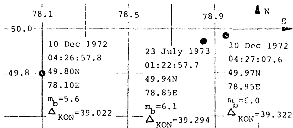
Fig. 1 Approximate great circle paths from the Eastern Kazakh test sites to KON (Norway) and CHG (Thailand). Below the locations and ISC parameters of the three events discussed in the text.
