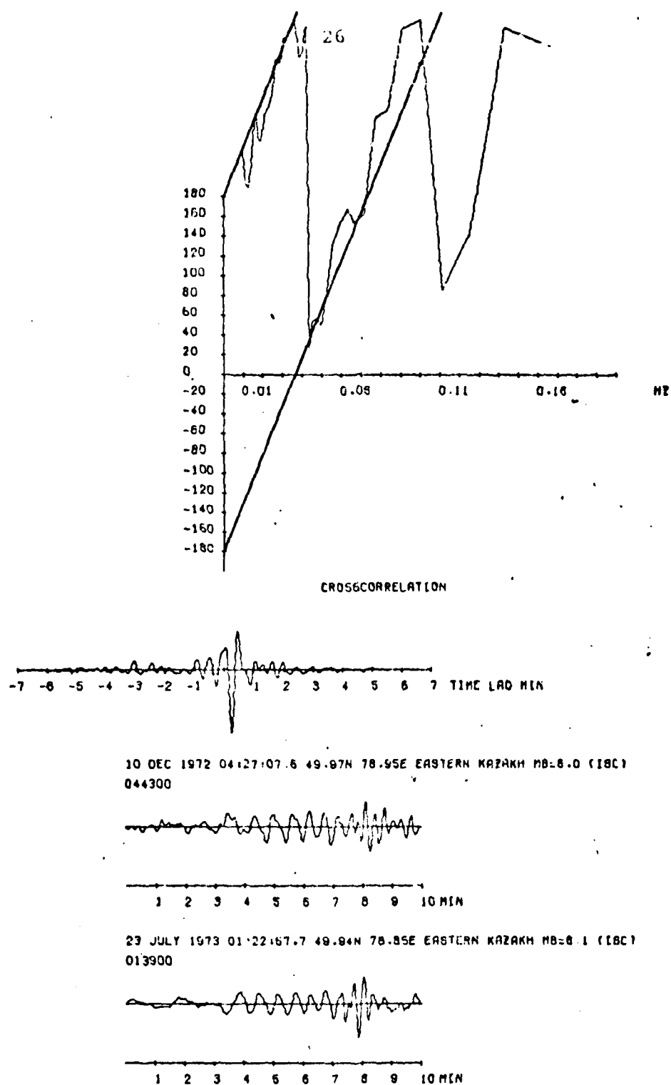
Fig. 4 Kongsberg ZHI recordings, crosscorrelation function and phase angle differences between the 10 Dec. 1972 and the 23 July 1973 event. The linear phase angle given by the solid lines represents a time shift of 14 sec which is the location of the crosscorrelation peak relative to 0-lag.
