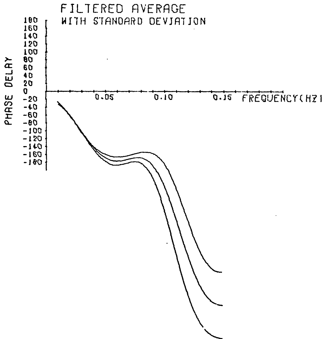
Fig. 4. A low pass filtered version of the phase difference curve in fig. 3 given with its standard deviation.
