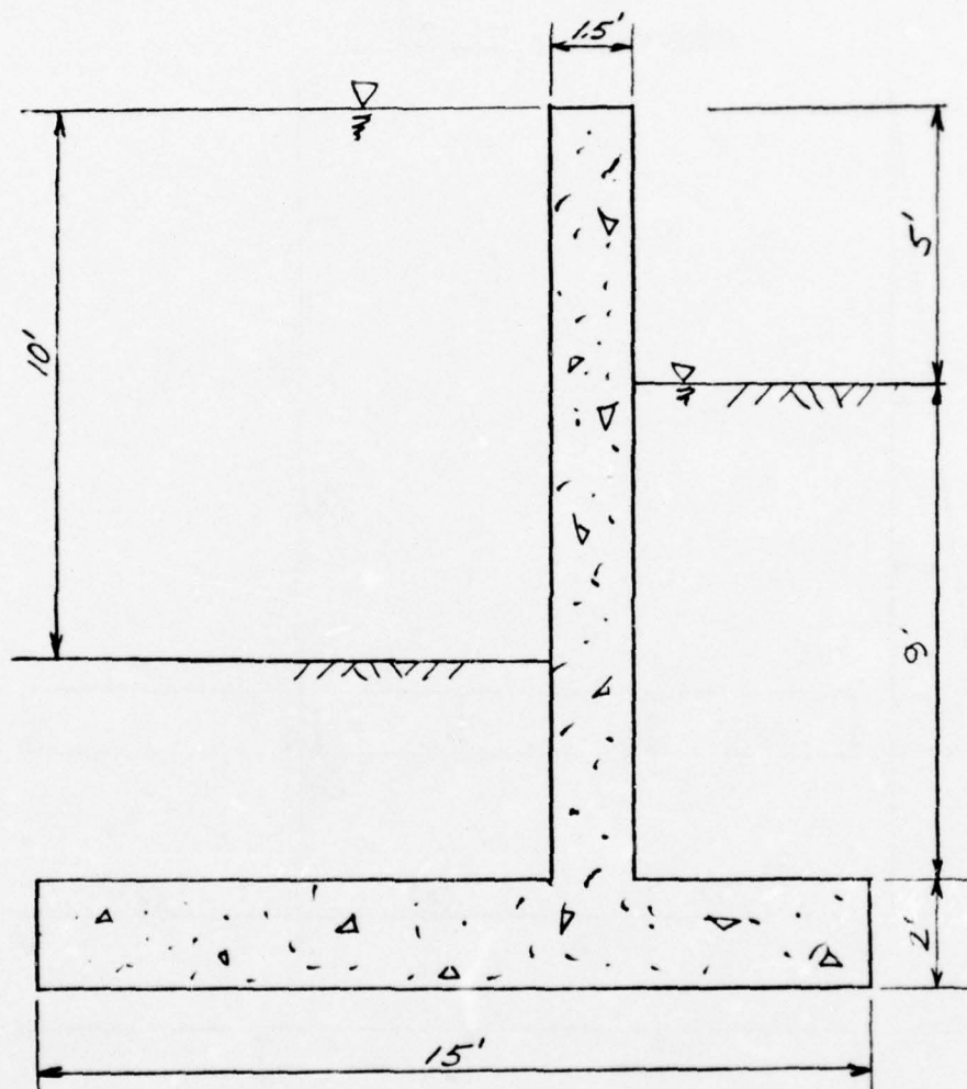
Section of Test wall Sketch 1.
