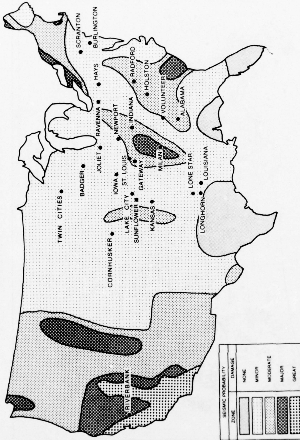
Figure 5. Seismic zone map of contiguous states
