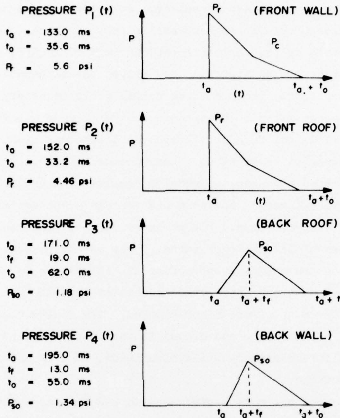
Figure 18. Load-time curves
