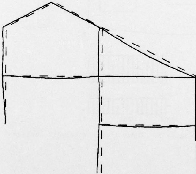
Figure 4. Displacement diagram
