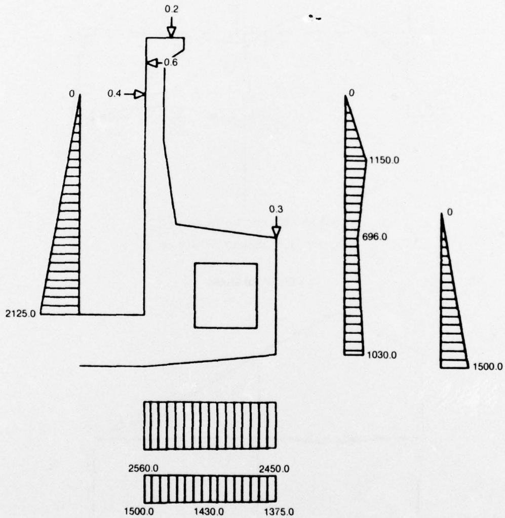
Figure 5. Input for lock culvert analysis
