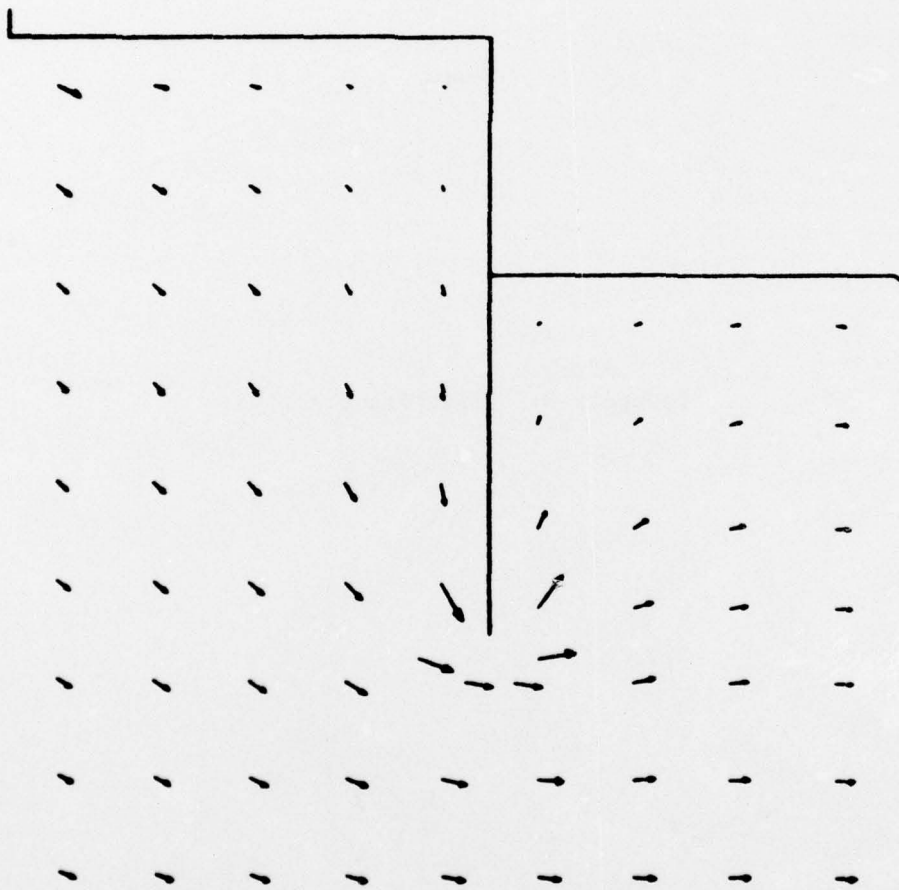
Figure 6. Vector plot of flows from FEM analysis
