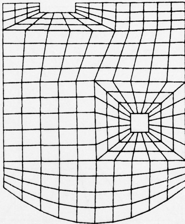
Figure 2. FEM grid of problem
