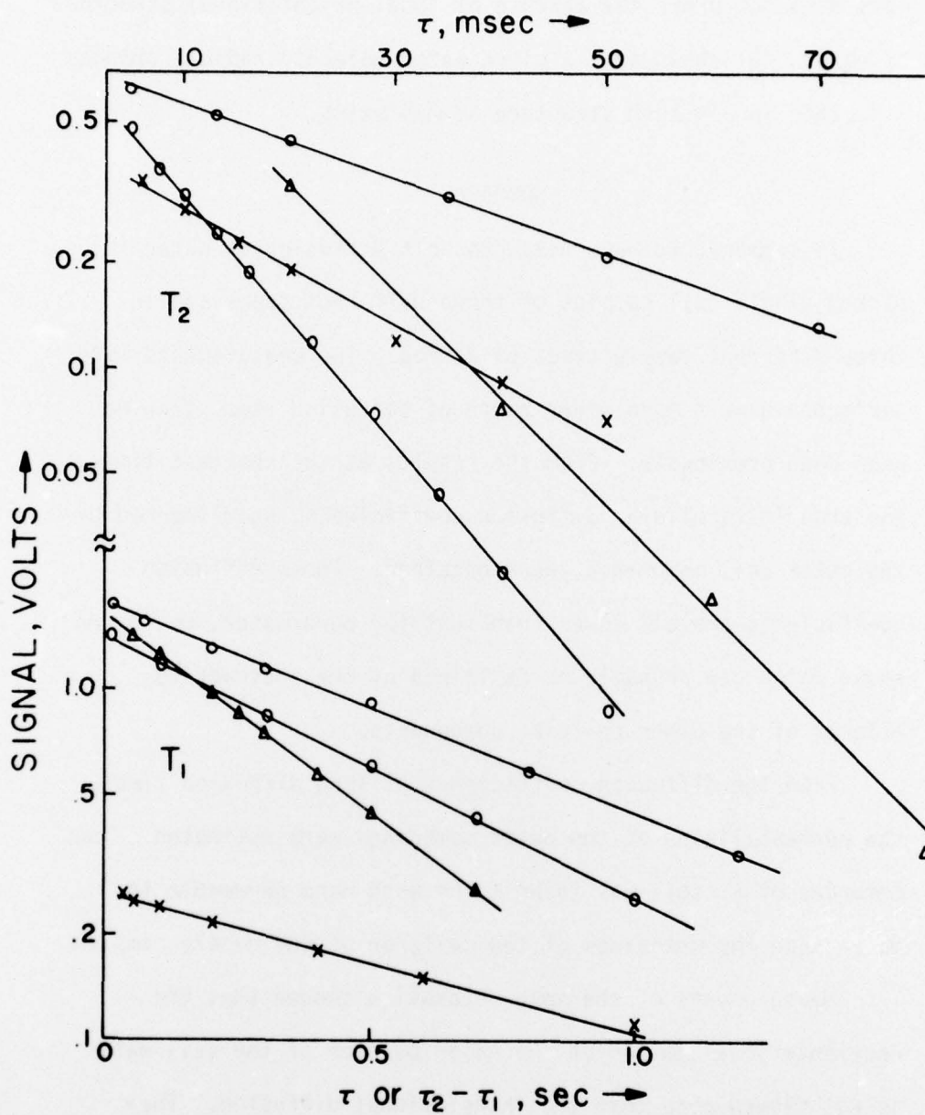
Figure 6. Representative signal decay curves due to T_1 and T_2 . The symbols are: o, red cells; \Delta , yeast; x, frog 2 muscle.
