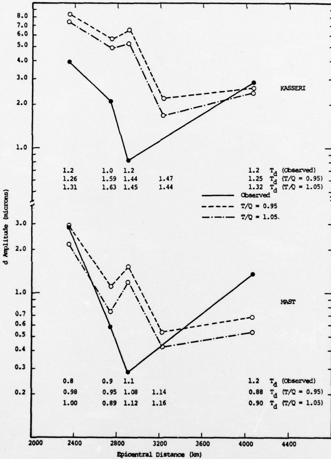
Figure 6. Comparison of theoretical and observed d amplitudes for MAST and KASSERI.
