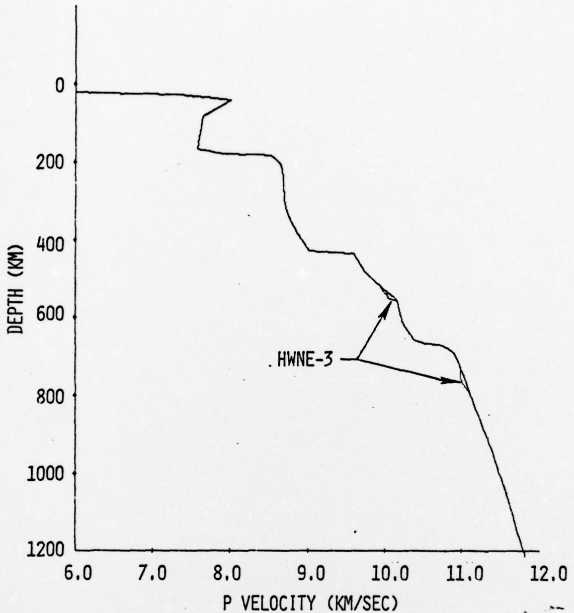
Figure 3. P velocity versus depth for the upper mantle model HWNE-3. This model is a slightly modified version of HWNE (Helmburger and Wiggins, 1971) with the differences as indicated in the figure.
