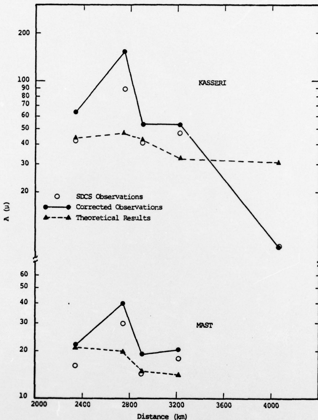
Figure 10. Comparison of theoretical and observed Airy phase amplitudes at five SDCS stations for KASSERI and MAST. Two observed values are shown; one set (SDCS) apparently used the LRSM nominal response curves and we corrected for the calibration response data.
