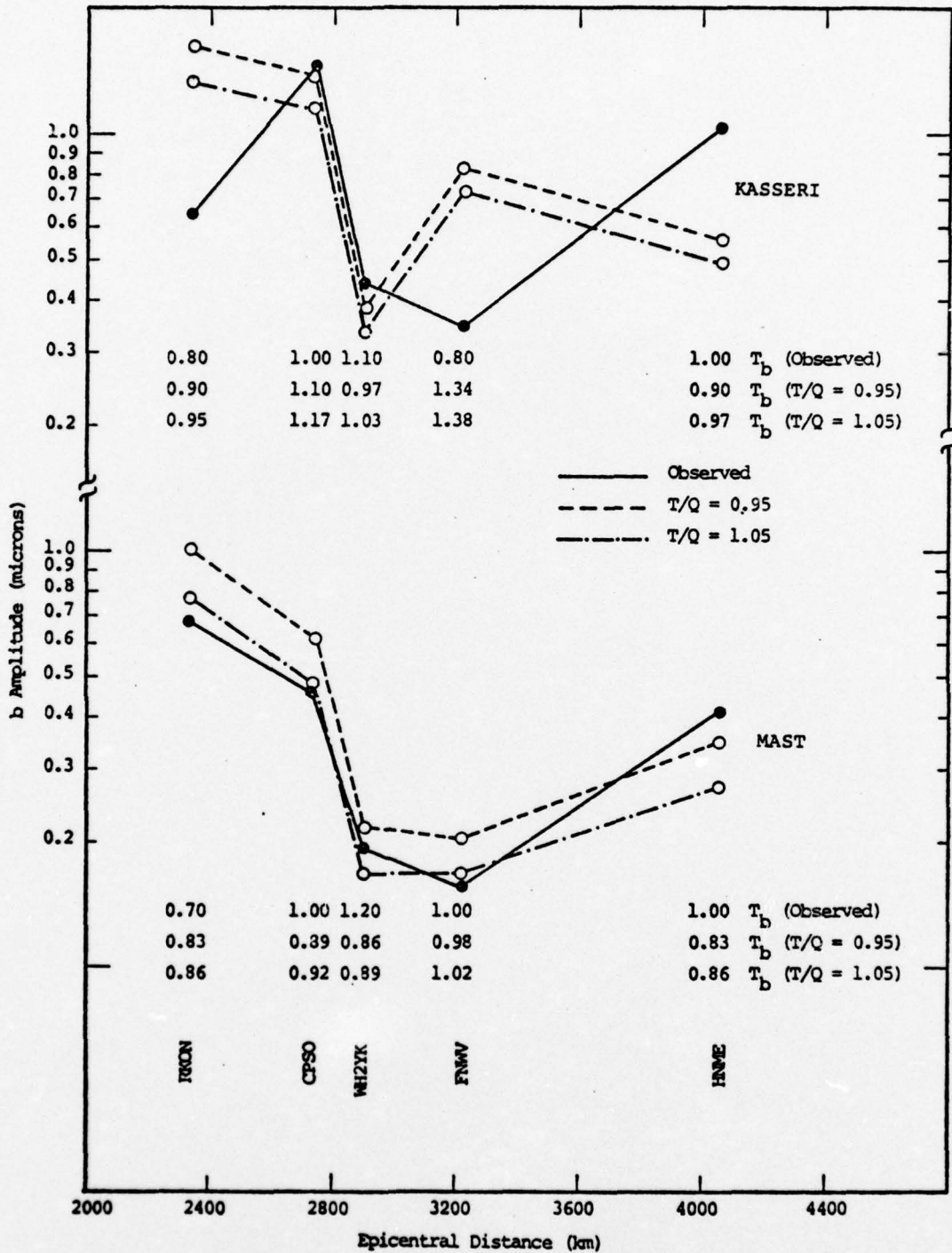
Figure 5. Comparison of theoretical and observed b amplitudes for MAST and KASSERI at five SDCS stations. Seismograms were computed for two values of T/Q as indicated. The KASSERI source function is denoted 148 and the upper mantle model is HWNE-3.
