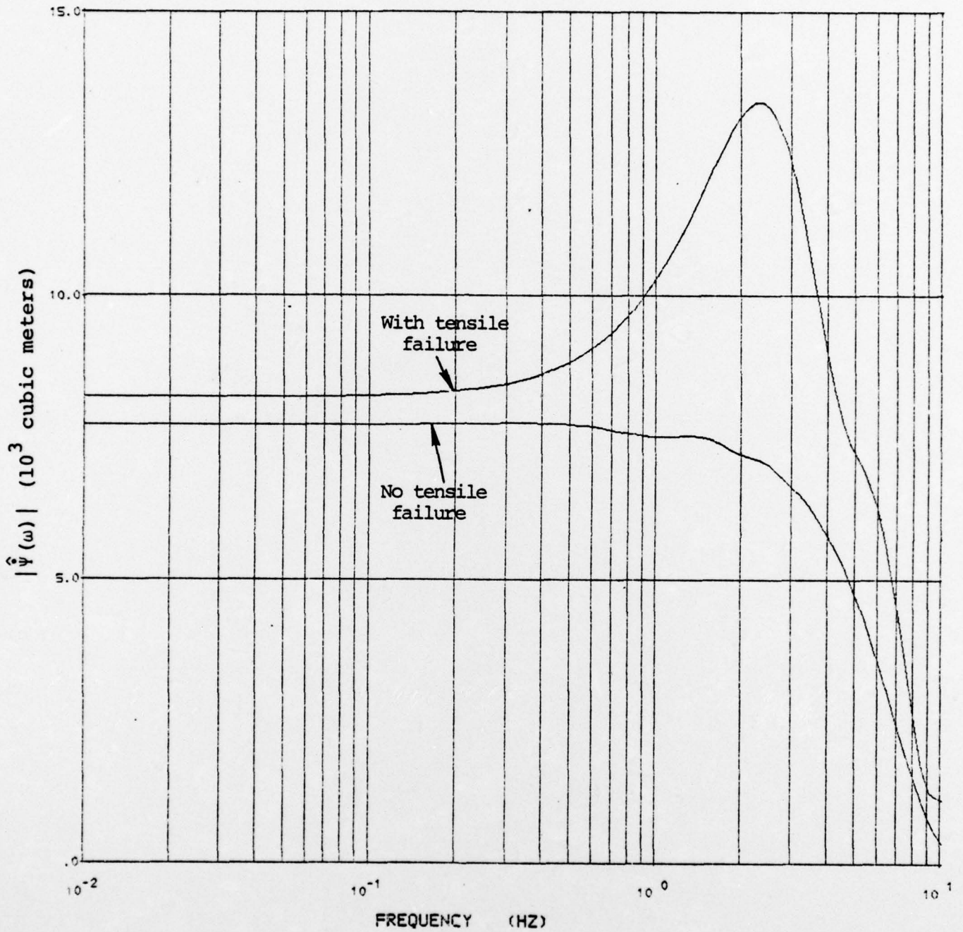
Figure 3.5. The amplitude of the transformed reduced velocity potential for two spherically symmetric explosion calculations. The explosion yield is 15 kt.
