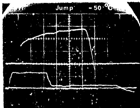
Fig. 5. Oscilloscope records for test conditions. (On left of figure pair, the initial condition)
