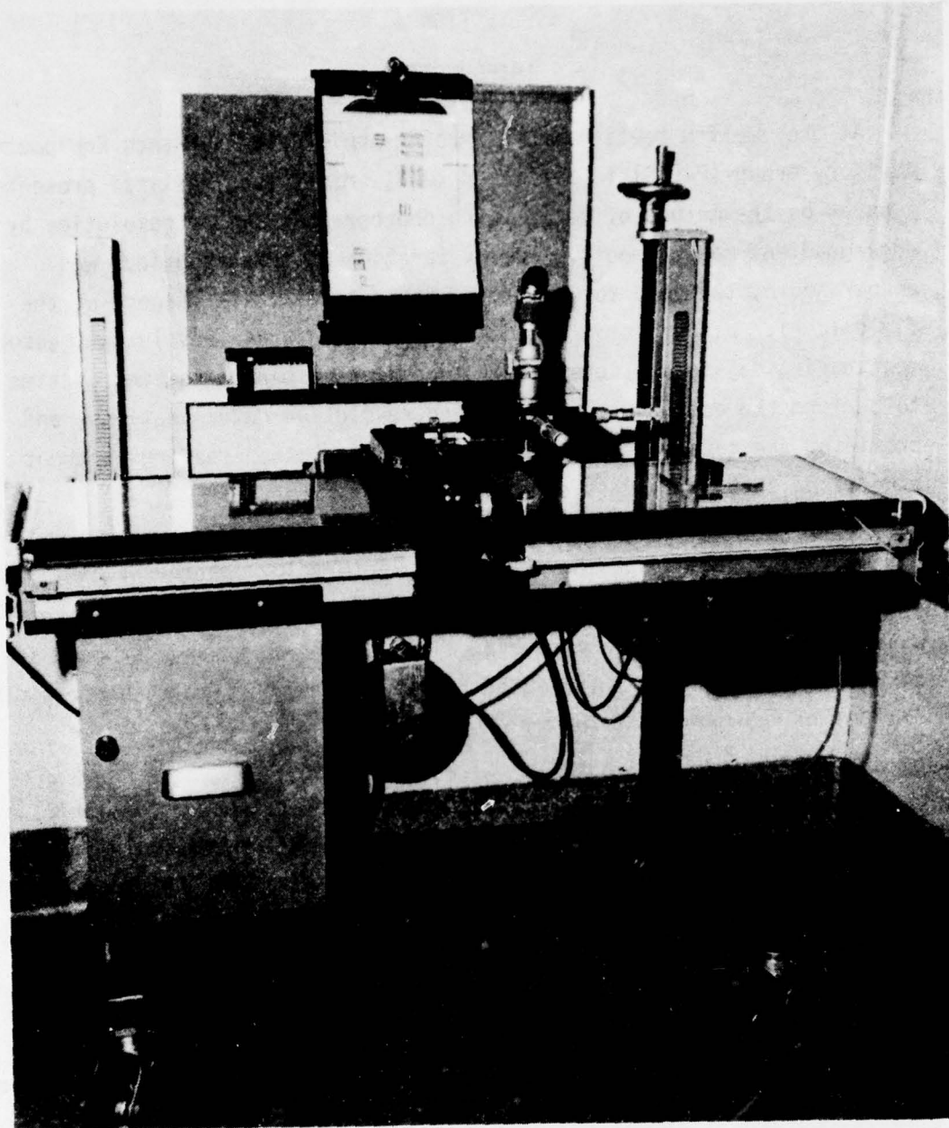
Figure 1. The Edge Gradient Image Analysis Microscope Mounted on a Richard's Light Table
