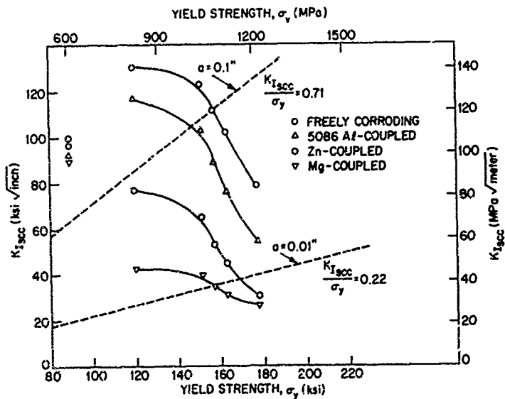
Fig. C1 — K_{I SCC} data for 17-4 PH steel of different yield strengths under four electrochemical conditions. (Conversion factors: 1 ksi = 6.895 MPa, 1 ksi√in. = 1.099 MPa√m, 1√in. = 1.594√cm, 1 in. = 2.54 cm.)
