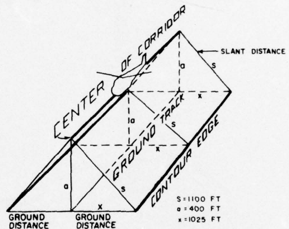
b. Perspective view showing altitude slant distance, center of corridor, and the contour lines paralleling the corridor.
