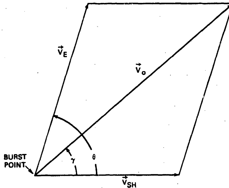
Figure 4. Static and Dynamic Fragment Emission.
