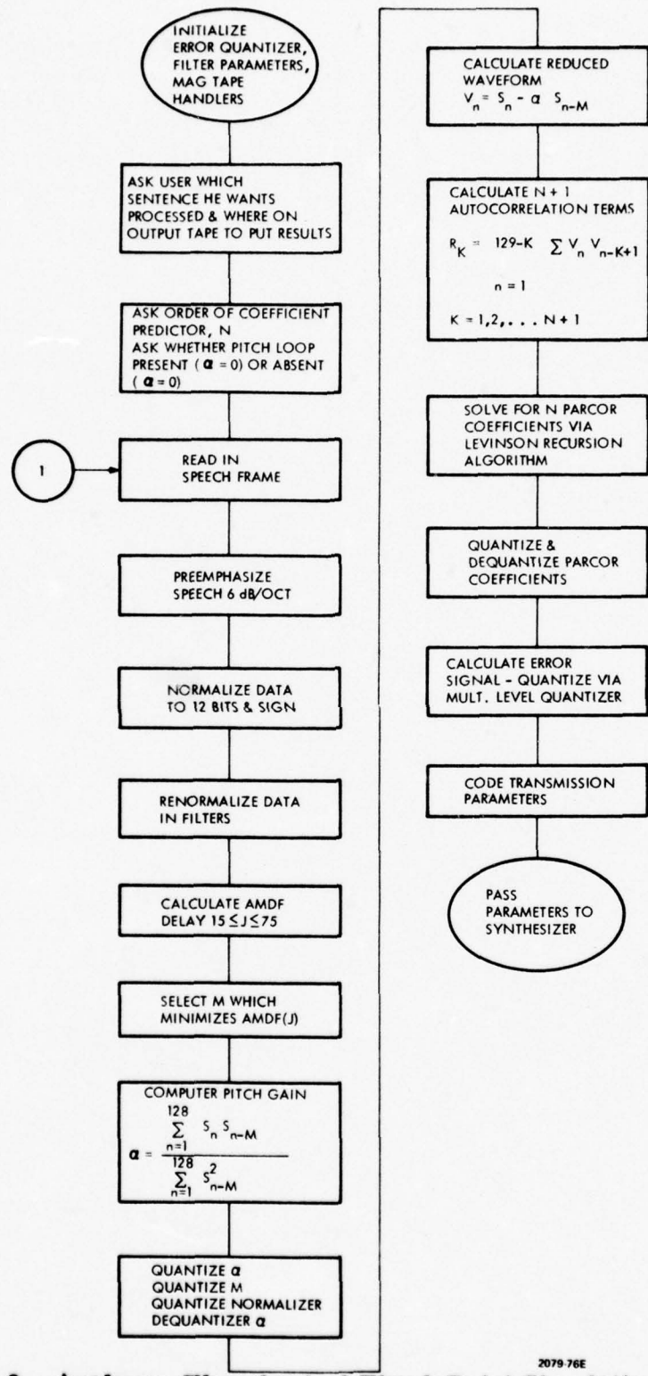
2079 76E Figure 2-8. Analyzer Flowchart of Fixed-Point Simulation for APCQ Coder
