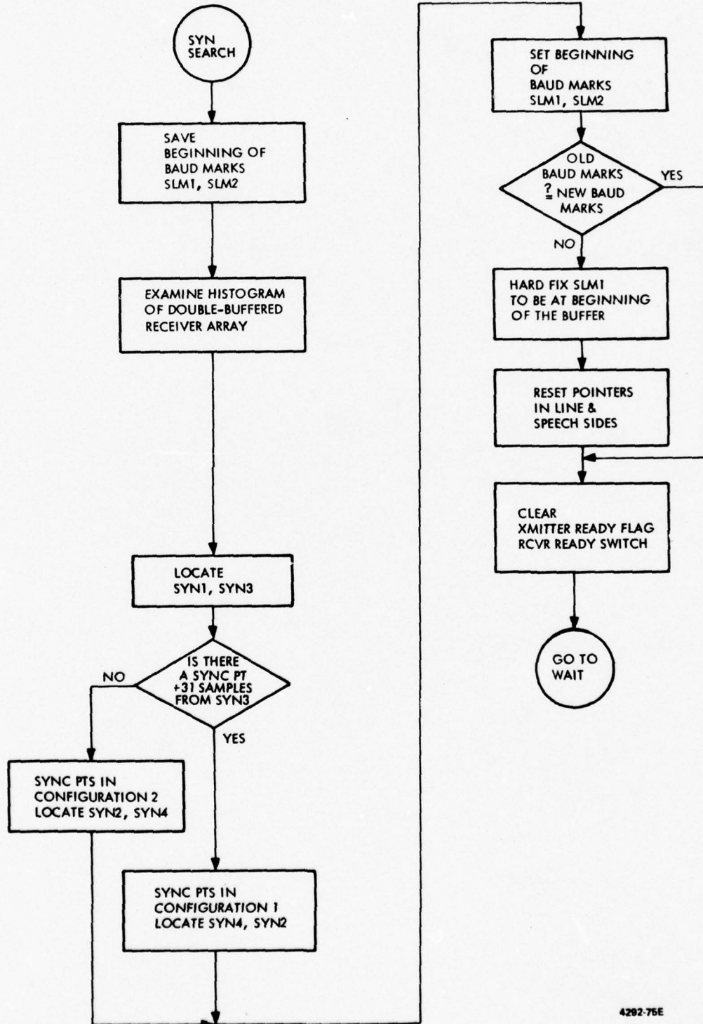
Figure 3-3. Synchronization Search
