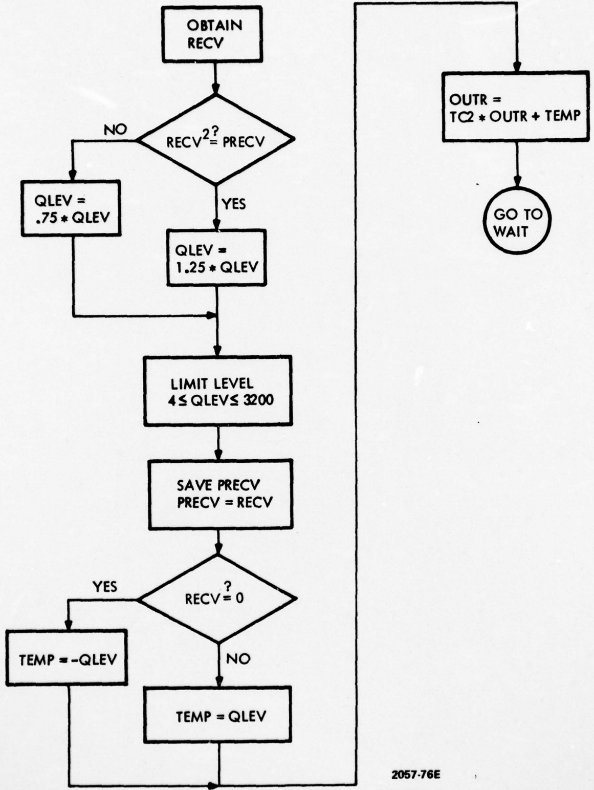
Figure 3-30. Receiver for CVSD-D
