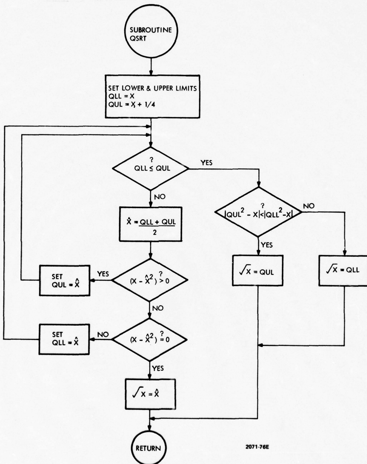
Figure 3-16. Subroutine QSRT
