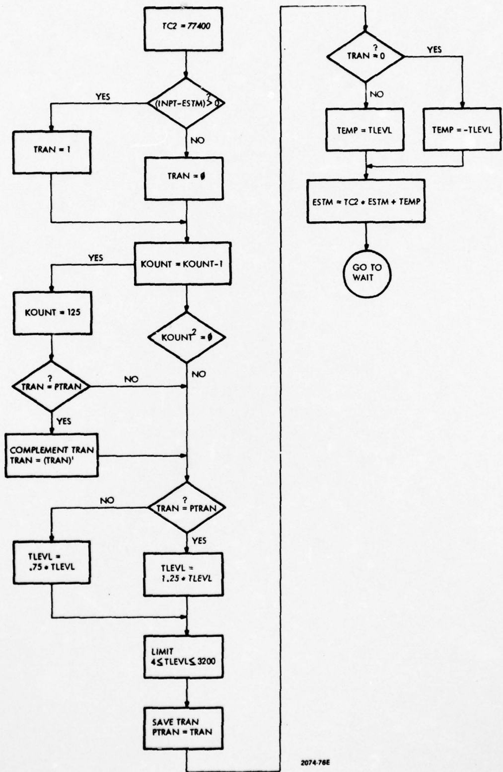
Figure 3-29. Transmitter for CVSD-D
