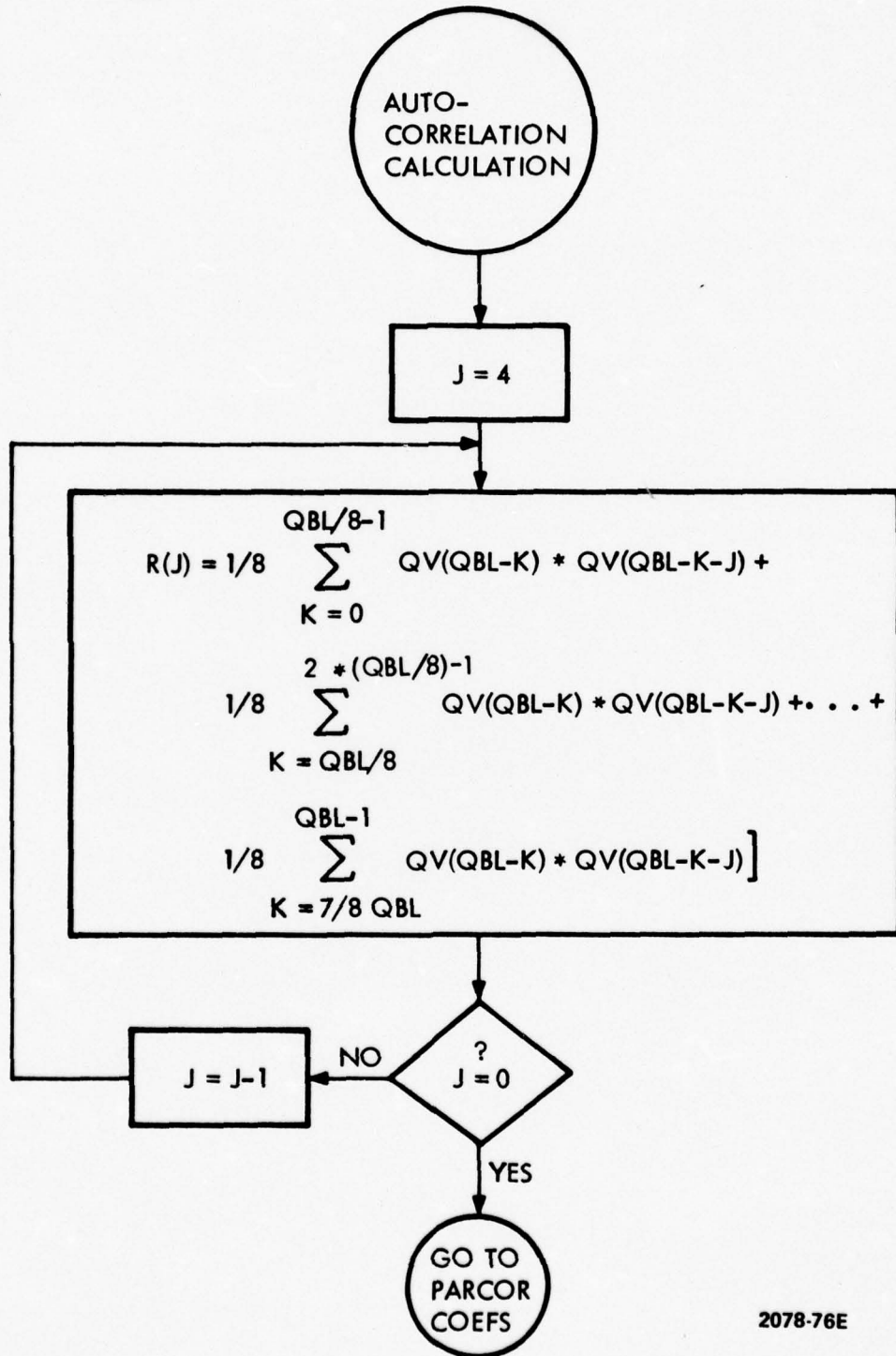
Figure 3-8. Autocorrelation Calculation
