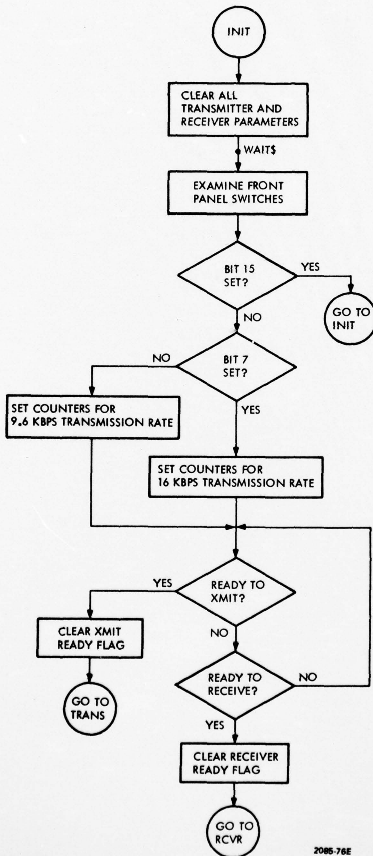
Figure 3-22. Initialization and Wait Loop
