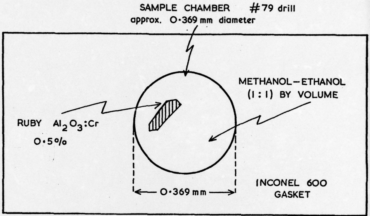
TOP VIEW
