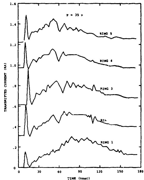
Figure 8d. Transmitted current measured on equal-area rings.
