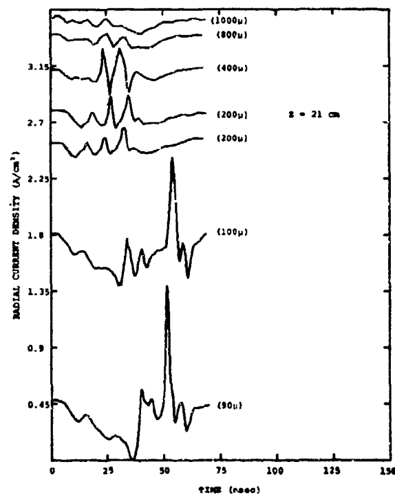
Figure 10h. Radial current density measured by the flush-mounted current probes (FMCP).
