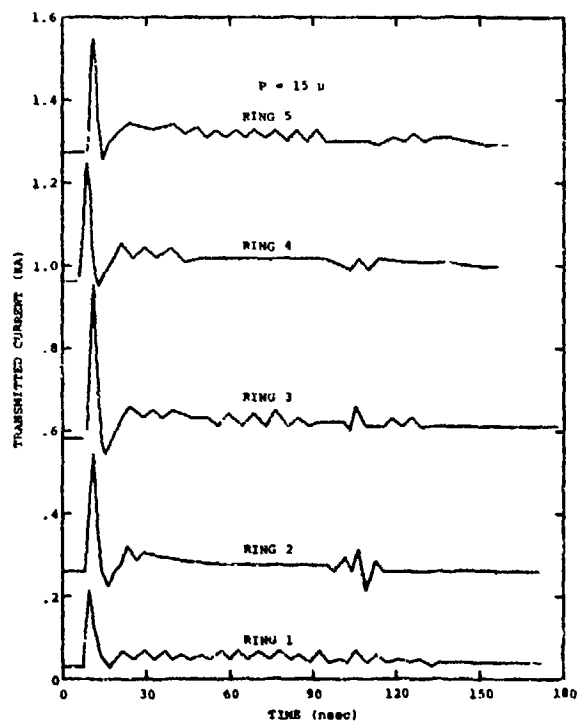
Figure 8b. Transmitted current measured on equal-area rings.
