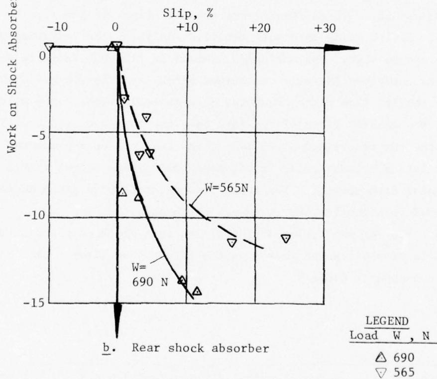
Fig. 19. Relations between \vec{F} \cdot \vec{\delta} and slip for front and rear shock absorbers, free-pitch mode, LSS 5 , phase I tests
