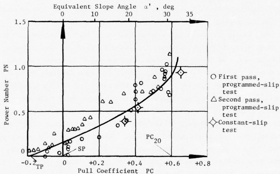
b. Power number as function of pull coefficient and equivalent slope angle
