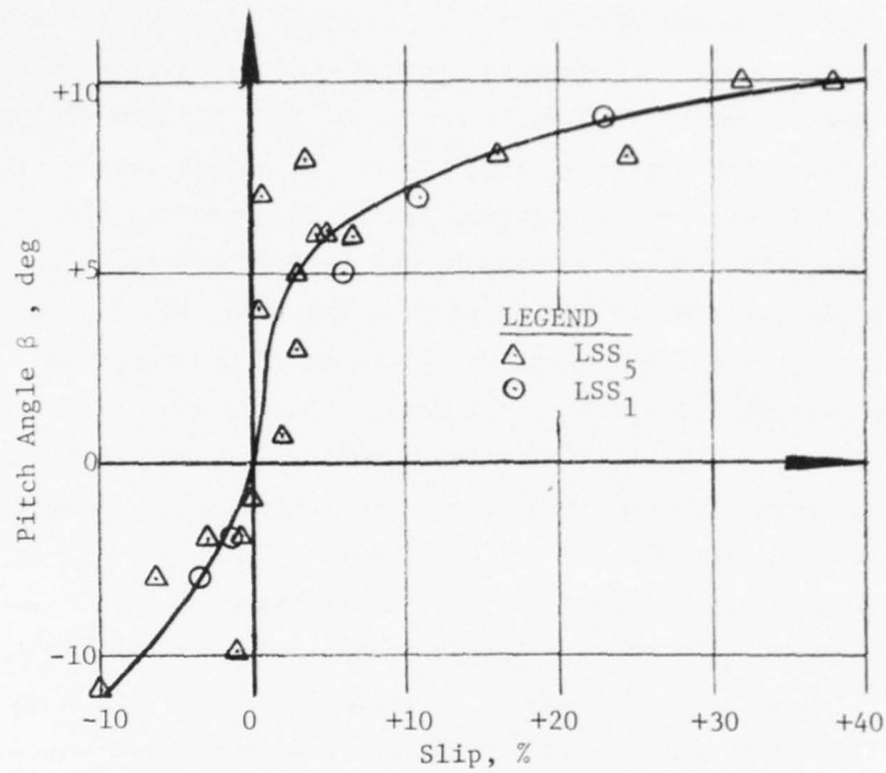
Fig. 16. Relation of pitch angle \beta to slip from tests with ELMS II in free-pitch mode
