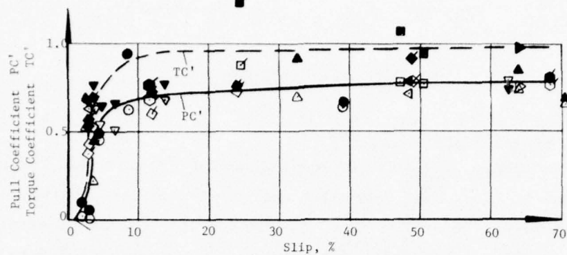
a. Pull and torque coefficients as functions of slip (open symbols: PC' ; closed symbols: TC' )
