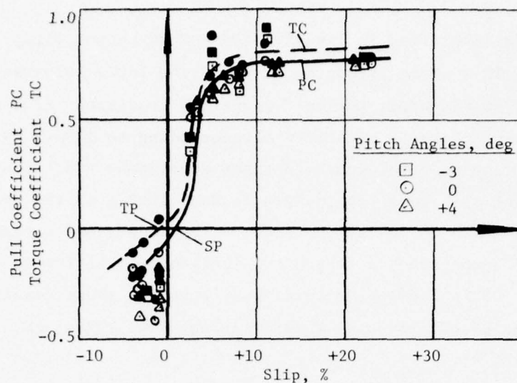
a. Pull and torque coefficients as functions of slip (open symbols: PC; closed symbols: TC)
