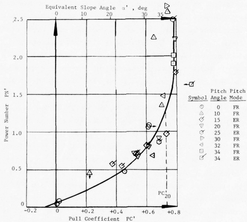
b. Power number as function of pull coefficient and equivalent slope angle
