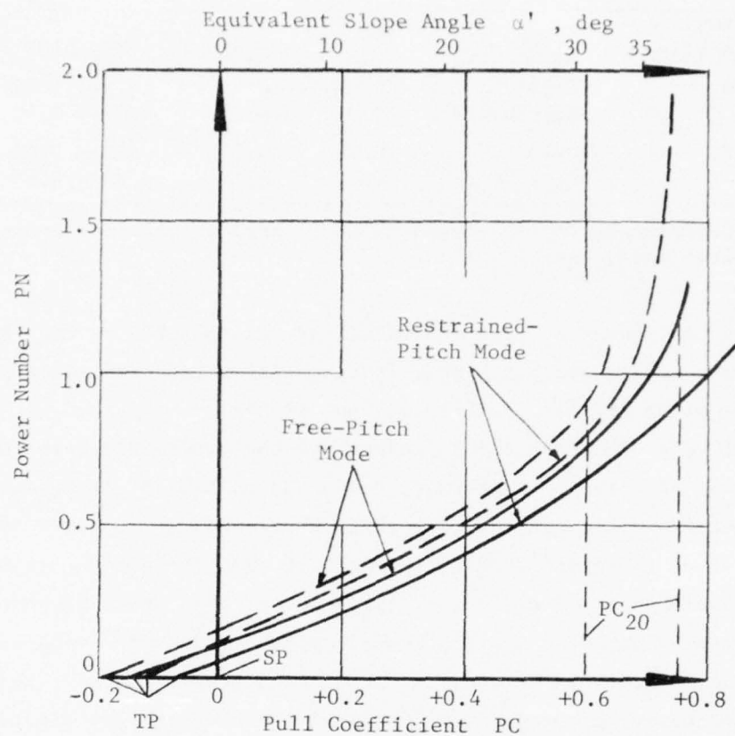
Fig. 17. Summary of PN versus PC relations developed from tests on level ground (phase I, figs. 10-13), soil conditions and pitch modes tested (solid lines: LSS 5 ; dashed lines: LSS 1 )
