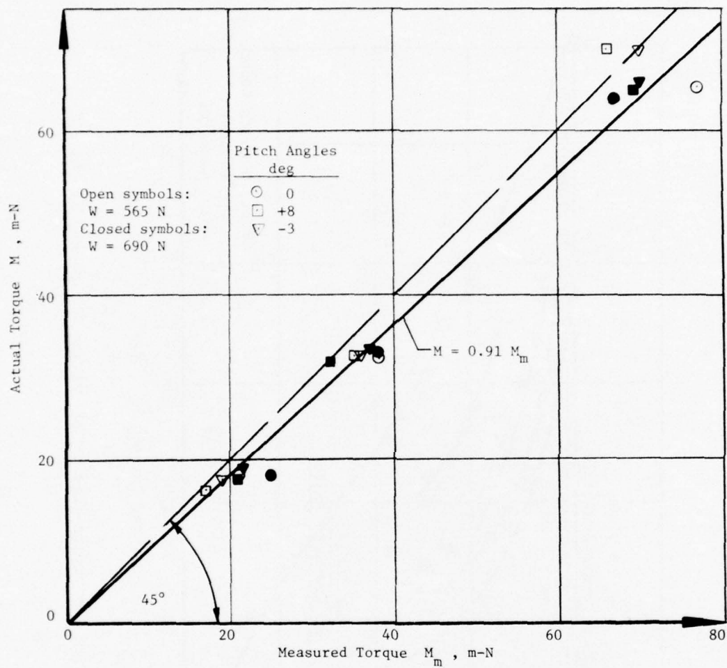
Fig. 5. Calibration for strain-gage torque method for phase I
