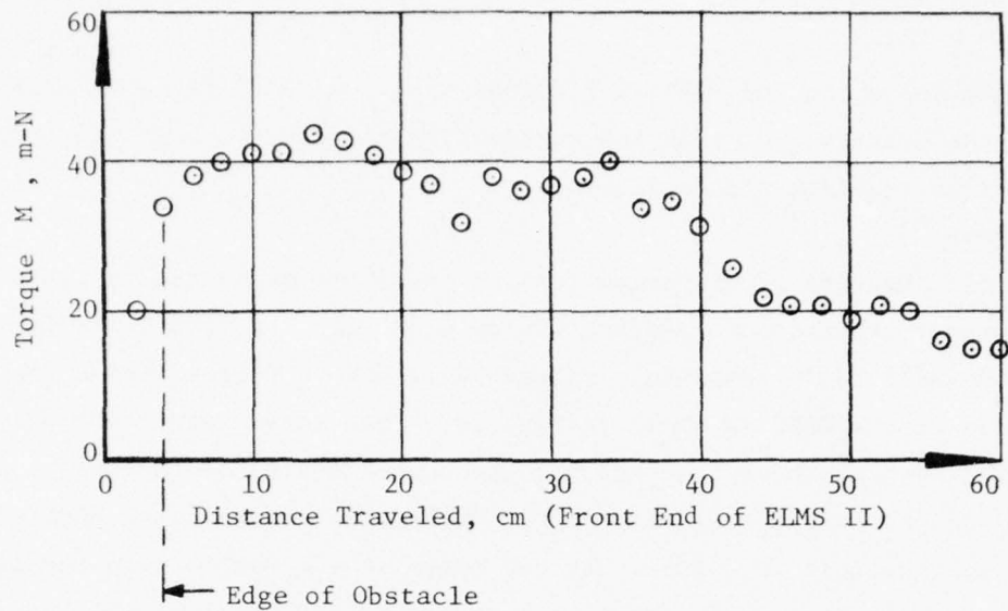
Fig. 25. Torque requirements for ELMS II in free-pitch mode climbing a 46-cm-high obstacle
