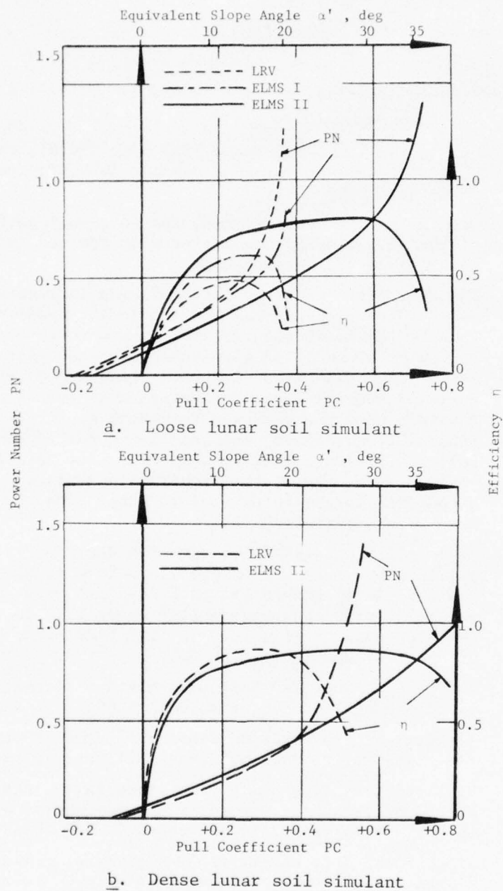
Fig. 30. Comparison of ELMS I, ELMS II, and LRV wheel performances on level ground
