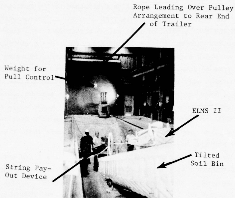
Fig. 7. Test setup for phase II, slope tests
