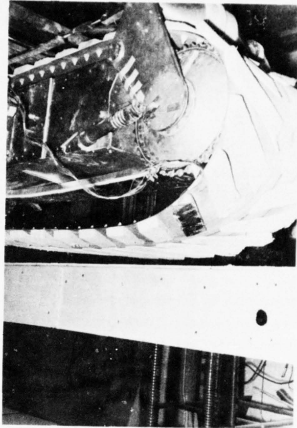
Fig. 9. Close-up of grouser instrumented for measuring contact pressure distribution
